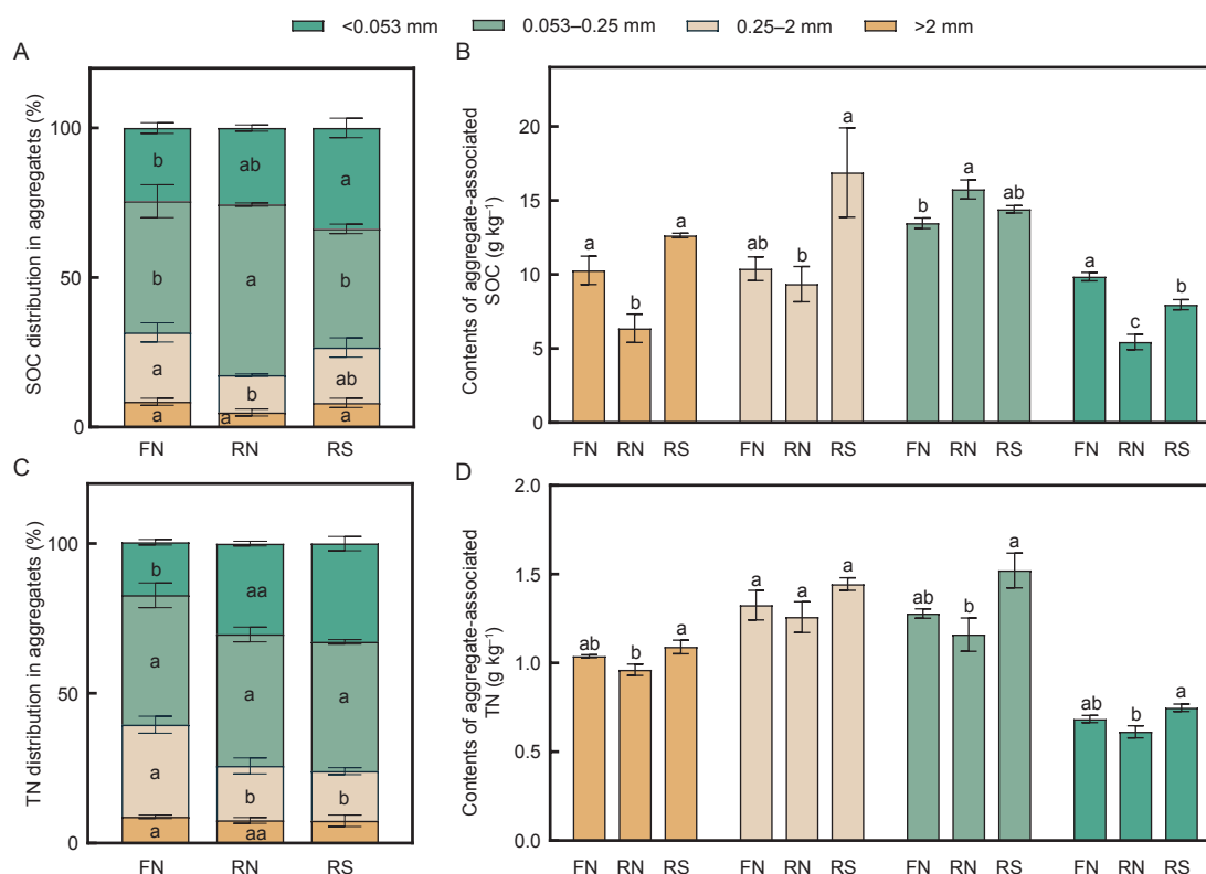
Fig. 1 Soil organic carbon (SOC) (A) and total nitrogen (TN) (C) distributions in soil aggregate fractions, and aggregate-associated SOC (B) and TN (D) contents. FN, conventional N application; RN, reduced N application; RS, reduced N with straw mulching. Different lowercase letters indicate significant differences between treatments at P<0.05 . Error bars represent the standard error ( n=3 ).
