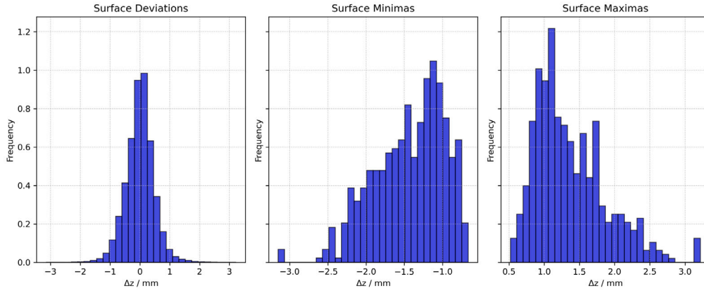
Fig. 2. Histograms representing the distribution of z-control point deviations in heliostat surface data, parameterized by NURBS. The left panel shows the overall distribution of surface deviations across all z-control points from all measured heliostat surfaces. The middle panel displays the distribution of the strongest negative deviations (surface minima) for each heliostat, while the right panel shows the strongest positive deviations (surface maxima). The views in the middle and right panel highlight outliers, providing clearer insight into the extremes of the heliostat surfaces.
