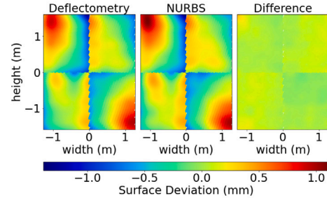
b) left: deflectometry surface constructed by a conventional integration-based algorithm from the deflectometry normals, middle: NURBS based heliostat surface, right: difference plot
