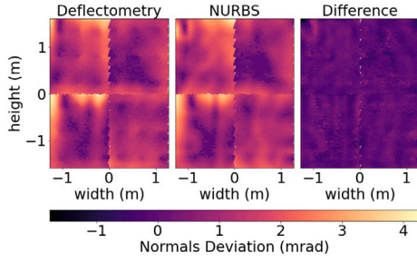
a) Left: normal deviation to the ideal flat surface of a deflectometry measurement, middle: normal deviation to the ideal flat surface of the NURBS parametrization of the deflectometry measurement, right: difference plot
