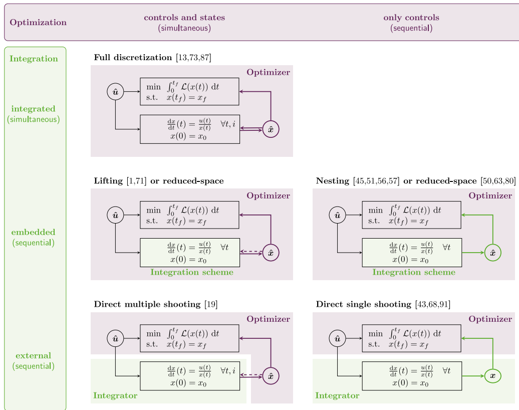
Fig. 2. Schematic overview of standard and hybrid methods for solving optimal control problems like (OCP). Such optimal control problems extend an algebraic optimization problem (upper box) by differential equations (lower box). From top to bottom, the handling of the differential equations changes, namely from transforming it into constraints handled by the optimizer (□) via using an integration scheme hidden from the optimizer (◻) to using an external integration software (◻). Arrows from controls and/or states to the model boxes indicate optimization variables. In the schemes on the left, both controls and states are optimized after applying state discretization (↔). The dashed arrow indicates that only a part of the state values are optimized (↔). In the schemes on the right, the state values are dependent variables since state integration is used (→).
