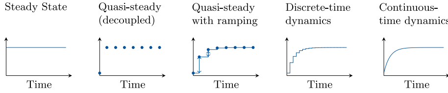
Fig. 4. Schematic overview of different paradigms for modeling process dynamics.
