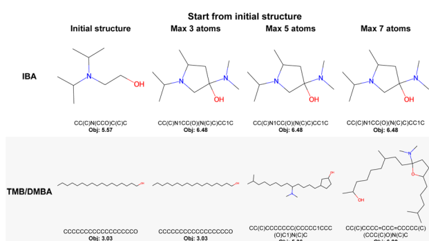
Fig. 6 Best molecule designed by GraphXForm when augmenting a specific initial structure by adding up to 3, 5, or 7 atoms. Bonds can be added without restriction. For the TMB/DMBA task, the designed molecule is also required to remain an alcohol.
