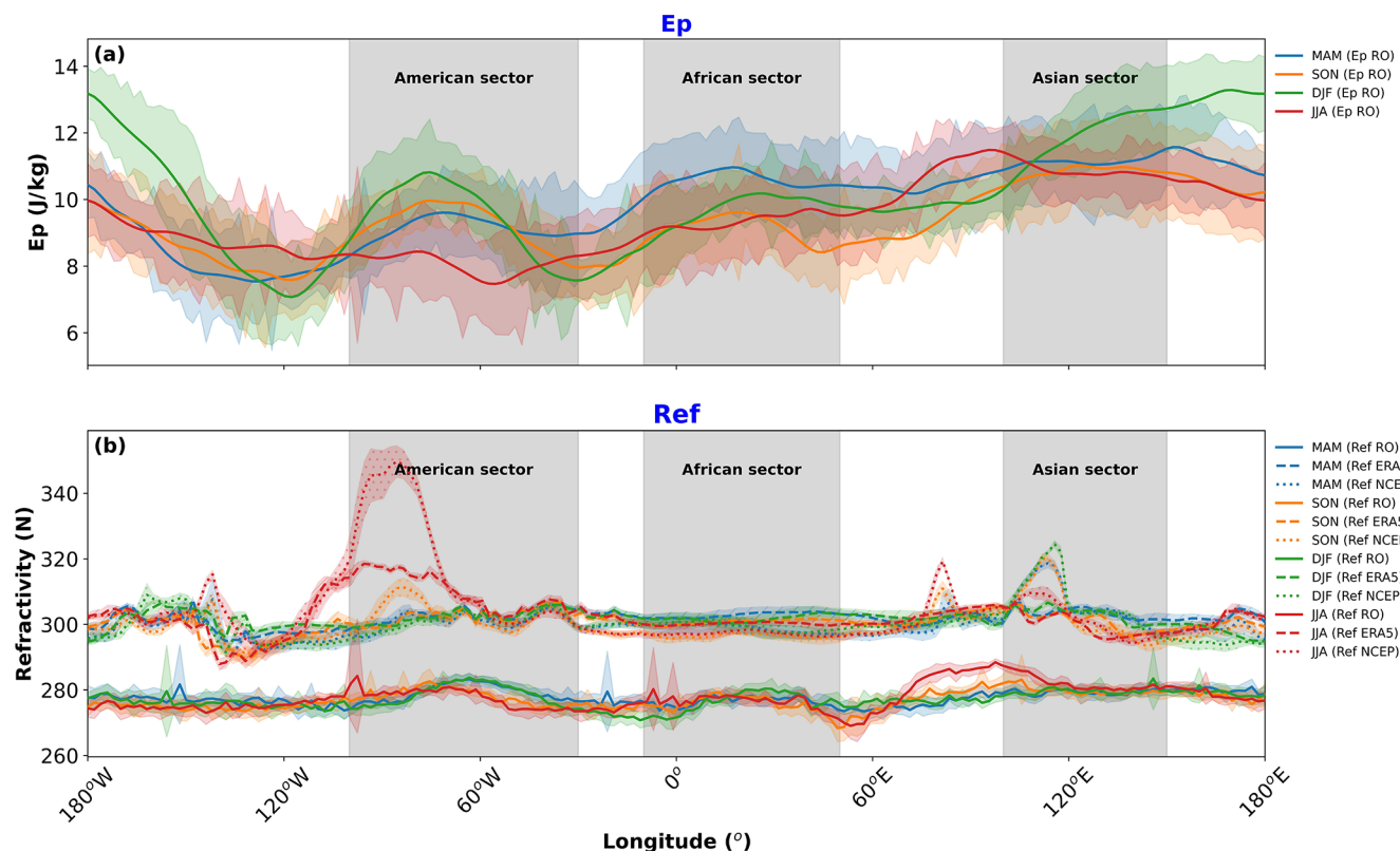
Figure 10. Longitudinal profiles of 11-year seasonal mean peak values derived from Gaussian fits. (a) Seasonal mean E_p peak values ( Q_{\text{peak}, E_p} , \text{J kg}^{-1} ) from RO for DJF (green), MAM (blue), JJA (red), and SON (orange). (b) Seasonal mean refractivity peak values ( Q_{\text{peak}, N} , N) from RO (solid lines), ERA5 (dashed lines), and NCEP (dotted lines) for DJF (green), MAM (blue), JJA (red), and SON (orange). Shading represents the standard deviation associated with the seasonal mean values.
