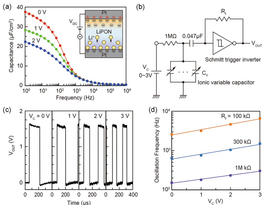
Fig. 29. (a) Variable capacitance demonstrated by a Pt/LiPON/Pt capacitor. The inset illustrates operation under application of V_{DC} . (b) VOC composed of a Schmitt trigger inverter and Pt/LiPON/Pt capacitors. (c) Typical output waveforms V_{OUT} obtained for different V_c at 50^\circ\text{C} with 4 Pt/LiPON/Pt capacitors. (d) Oscillation frequency plotted as a function of V_c with different feedback resistance values of R_f . Reprinted with permission from Ref. [150]. Copyright (2020) American Chemical Society.
