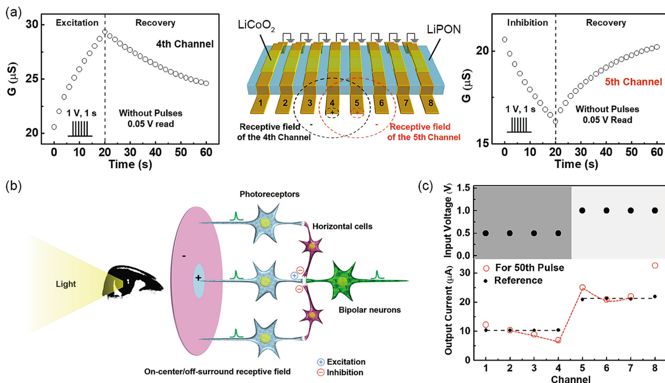
Fig. 22. Lateral inhibition in multi \text{LiCoO}_2 channels arranged on a common LiPON electrolyte film. (a) Excitation of one channel and inhibition of a neighboring channel by applying voltage pulses. (b) Schematic diagram of an on-center/off-surround receptive field in the retina consisting of photoreceptors directly and indirectly connected via horizontal cells to a bipolar cell. (c) Implementation of the Mach band effect by a device with eight channels. Reprinted with permission from Ref. 123. Copyright (2021) American Chemical Society.
