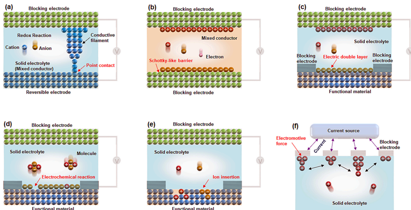
Fig. 2. Device structures and operating principles of ionic nanarchitectonics for controlling (a) a conductive filament, (b) a Schottky-like barrier, (c) an electronic double layer, (d) electrochemical reaction, (e) ion insertion, (f) electromotive force. Reprinted with permission from Ref. 18. Copyright (2022) Wiley-VCH GmbH.
