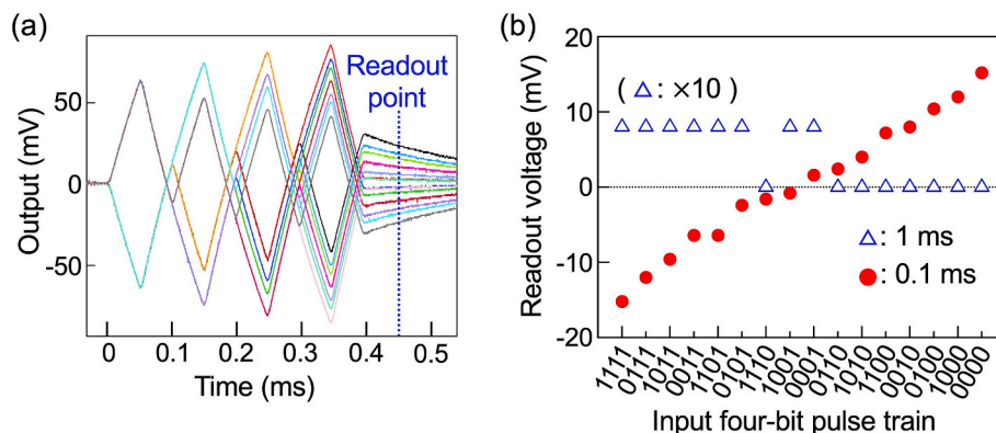
Fig. 15. Experimental result on 4-bit pulse classification. (a) Change in output measured for an input consisting of a four-bit pulse train. The readout point is indicated. (b) Readout voltages for each four-bit pulse train. Reprinted from Ref. [98]. Copyright 2024 The Japan Society of Vacuum and Surface Science.
