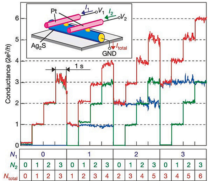
Fig. 5. Changing the QC states of individual channels independently from N = 0 ( \times 2e^2/h ) to 3 ( \times 2e^2/h ). 50-ms-long pulsed bias voltages of 200 mV (from 0 to 1), 100 mV (from 1 to 2), 80 mV (from 2 to 3) and –260 mV (from 3 to 0) were applied. Reprinted with permission from Ref. [22]. Copyright (2005) Springer Nature.
