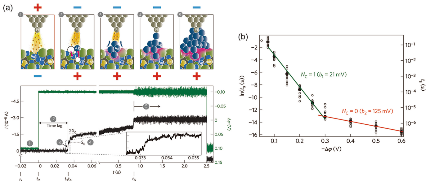
Fig. 6. (a) Relationship between filament formation process and current response in an experiment on Fe-doped \text{RbAg}_4\text{I}_5 film evaporated on a Ag substrate under application of a constant voltage by STM. The numbers (1–5) define five time domains in the current-time characteristic corresponding to the microscopic processes illustrated in the upper part of the figure. t_i denotes the starting time of the i th process. The inset shows the current increase in time domain (3), where the current reached the value of a single atomic point contact. (b) Switching time plotted as a function of bias voltage. The measurement was carried out at room temperature on a STM Pt tip and \text{RbAg}_4\text{I}_5 surface. Reprinted with permission from Ref. [30]. Copyright (2012) Springer Nature.
