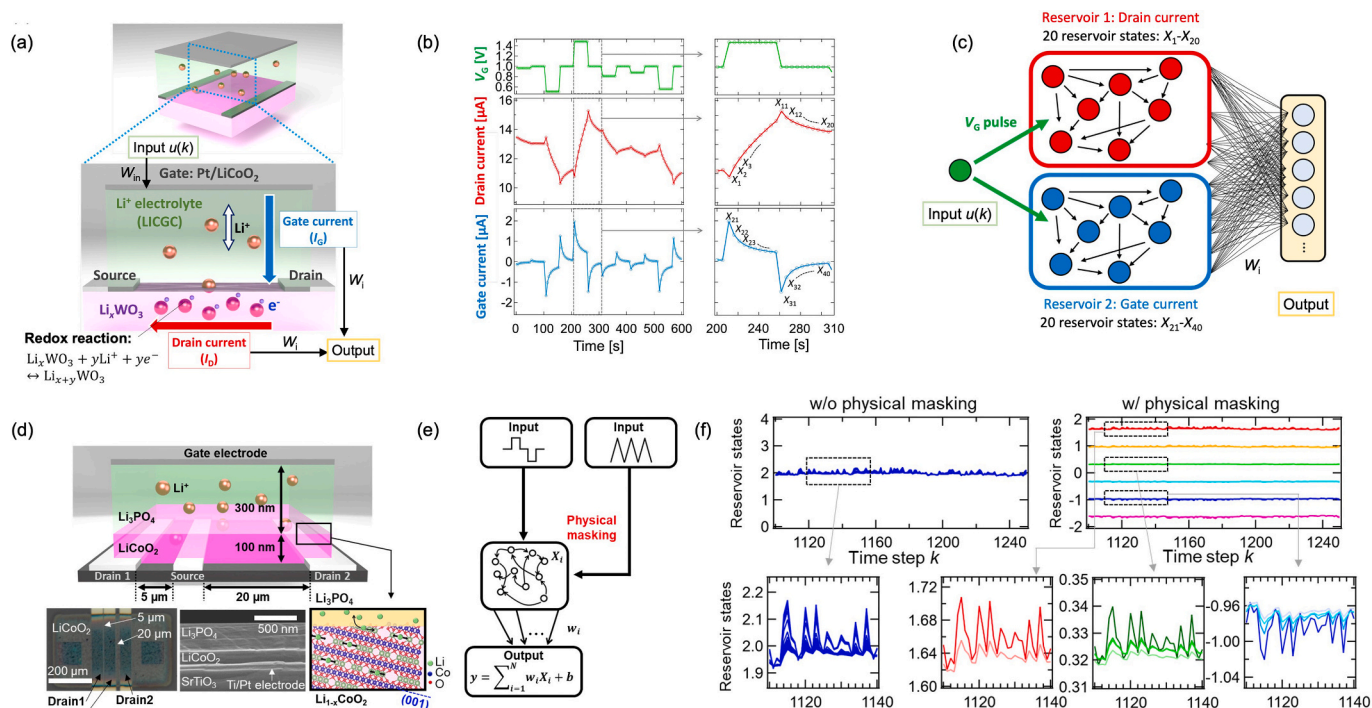
Fig. 20. (a) Schematic image of a \text{Li}_x\text{WO}_3 -based redox-IGR. (b) Gate voltage pulse stream, drain current response, and gate current response during operation of the redox-IGR. Forty reservoir states X_i ( i = 1, \dots, 40 ) are obtained as shown in the panels on the right. (c) General concept of a reservoir computing system with redox-IGRs. W_i denotes the readout weight. Reprinted with permission from Ref. [108]. Copyright (2023) Wiley-VCH GmbH. (d) Schematic and optical images of \text{LiCoO}_2 -based redox-ion gating reservoir (IGR), cross-sectional SEM micrograph of a \text{LiCoO}_2 redox-IGR, and depiction of insertion (desertion) of \text{Li}^+ ions in (104) oriented \text{LiCoO}_2 . (e) Reservoir computing with physical masking. (f) Reservoir state waveforms ( X_1, X_2, \dots, X_{20} ) w/o and w/ physical masking. Reprinted with permission from Ref. [110]. Copyright (2023) Springer Nature.
