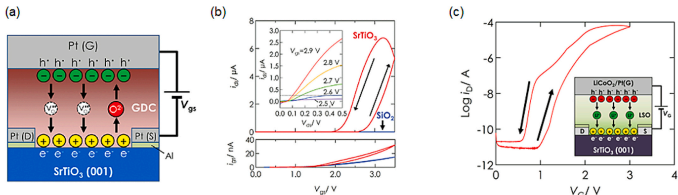
Fig. 24. (a) Schematic illustration of STO-based EDLT using GDC oxide ion conductor and STO single crystal. Yellow and green circles indicate positive and negative charges accumulated at interfaces through oxide ion and vacancy migration. O^{2-} and V_O show negative oxide ion and the positive vacancy, respectively. (b) i_{ds} vs. V_{gs} (upper panel) and i_{gs} vs. V_{gs} (lower panel) characteristics of STO-based EDLT measured at 473 K in air (red lines). For comparison are shown results for a SiO 2 -based EDLT consisting of a SiO 2 substrate and GDC oxide ion conductor (blue lines). The inset depicts i_{ds} vs. V_{ds} characteristics for various V_{gs} . Reproduced with permission. [128] Copyright 2013, AIP Publishing. (c) Electrical conduction characteristic ( i_D vs. V_G ) of STO-based EDLT with LiSiO 4 electrolyte measured at RT in vacuum. Reprinted with permission. [133] Copyright (2015), AIP Publishing. (For interpretation of the references to colour in this figure legend, the reader is referred to the web version of this article.)
