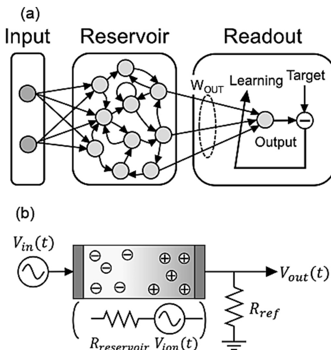
Fig. 12. (a) Artificial neural network (ANN) for reservoir computing. (b) Reservoir operations based on movements of ions in an electrolyte.
