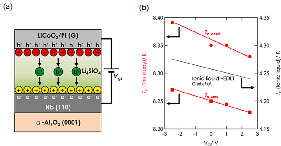
Fig. 26. (a) Schematic illustration of Nb-based EDLT composed of LSO Li + ion conductor and LCO gate electrode. Yellow and red circles represent positive and negative charges accumulated at interfaces due to Li + ion migration. (b) Variation in superconducting transition temperatures ( T_{c, \text{onset}} and T_{c, \text{zero}} ) plotted with respect to V_G . Reprinted with permission from Ref. [133] Copyright (2015), AIP Publishing. (For interpretation of the references to colour in this figure legend, the reader is referred to the web version of this article.)
