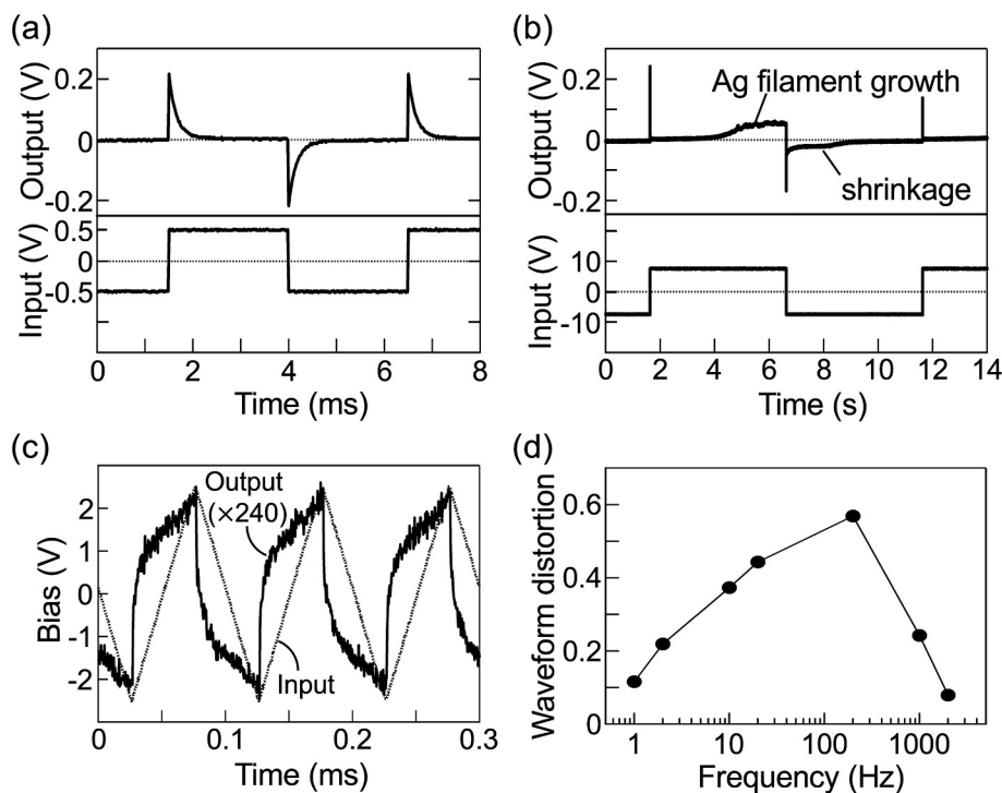
Fig. 14. Nonlinear transformation using an \text{Ag}_2\text{S} -based reservoir. Output measured with rectangular pulse input with an amplitude and period of (a) 0.5 V and 2.5 ms and (b) 7.5 V and 5 s. (c) Measured output for triangular pulse input (2.5 V, 0.05 ms). (d) Degree of nonlinear transformation of triangular pulse input. Reprinted with permission from Ref. [89]. Copyright 2024 The Japan Society of Vacuum and Surface Science.
