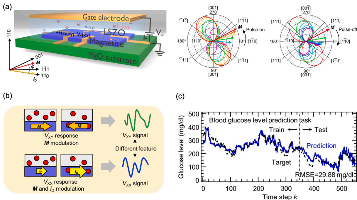
Fig. 21. (a) Schematic illustrations of (left) magnetization angle rotation ion-gating reservoir and (right) magnetic anisotropy and magnetization angle. \phi is defined as the relative angle between the electric current I_D and magnetization M . (b) Schematic illustration of V_{XY} (magnetization) and V_{XX} (drain conductance) responses to a pulsed voltage. (c) Target waveform of blood glucose level and waveform predicted with a magnetization angle rotation ion-gating reservoir. Black and blue solid lines denote target and predicted waveforms, respectively. Reprinted with permission from [114]. Copyright (2024) American Chemical Society. (For interpretation of the references to colour in this figure legend, the reader is referred to the web version of this article.)
