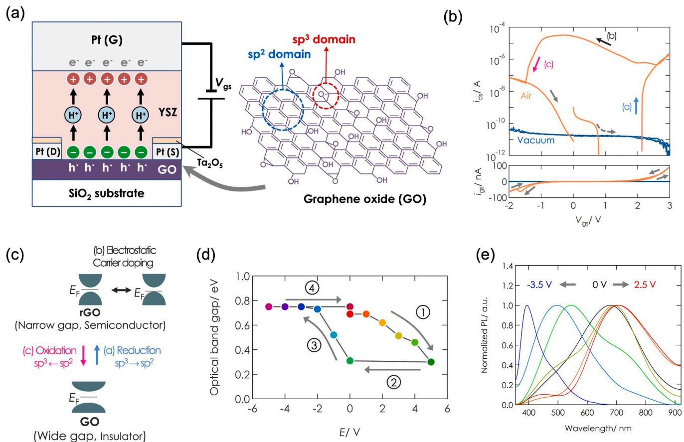
Fig. 25. (a) Schematic illustration of GO-based EDLT with YSZ proton conductor. Brown and green circles represent positive and negative charges accumulated at interfaces due to proton migration. H^+ symbols represent positively charged protons. (b) Electrical conduction characteristics of GO-based EDLT measured in air and vacuum: i_{ds} vs. V_{gs} (upper panel) and i_{gs} vs. V_{gs} (lower panel). Sweep rate of V_{gs} was 4 mV/s; V_{ds} was 0.5 V. (c) Illustration of electrostatic carrier doping (ECD) by EDL charging/discharging and bandgap tuning (BGT), corresponding to a redox reaction, of GO. (d) DC bias dependence of optical band gap tuned by the device. Reprinted with permission from Ref. [134] by The Author(s) licensed under CC BY 4.0, published by Wiley. (e) DC bias dependence of normalized photoluminescence (PL) spectra tuned by application of various DC bias voltages. Reprinted with permission from Ref. [139]. Copyright (2015) American Chemical Society. (For interpretation of the references to colour in this figure legend, the reader is referred to the web version of this article.)
