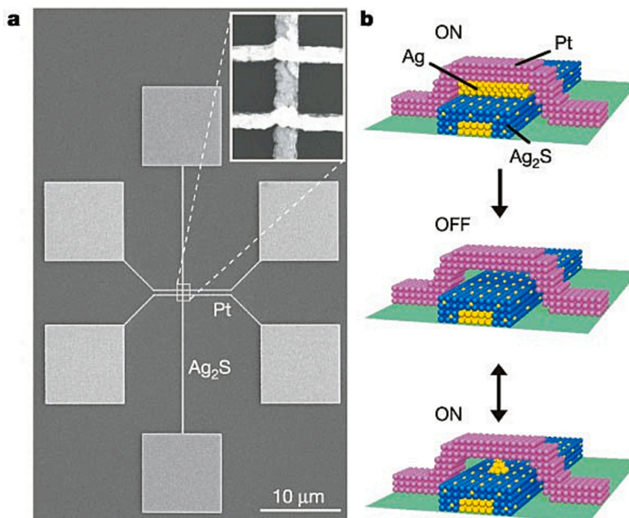
Fig. 4. (a) SEM image of a gap-type atomic switch. Two switches are formed at the crossing points of the 150-nm-wide \text{Ag}_2\text{S} wire and the two 100-nm-wide Pt wires. (b) Schematic diagrams of the atomic switch. As-formed switched-on state (top), switched-off state (middle) and switched-on state after the initial switching-off process (bottom). Reprinted with permission from Ref. [22]. Copyright (2005) Springer Nature.
