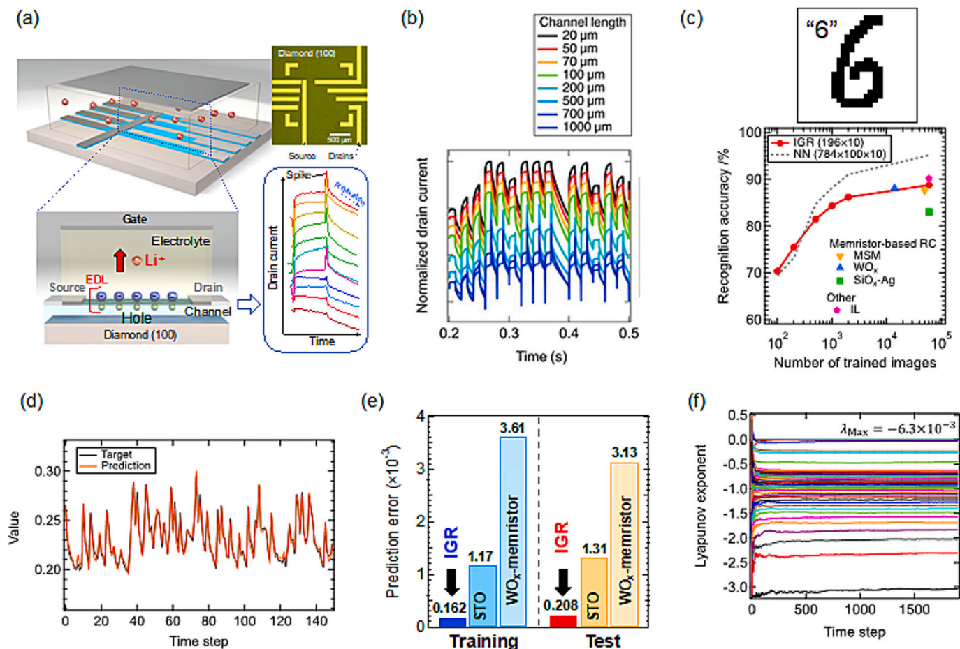
Fig. 19. (a) Illustration of ion-gating reservoir (IGR) operating in an electric double layer mechanism. (b) Drain current responses of the IGR for different channel lengths. (c) Image recognition accuracy achieved by IGR as a function of the number of training images. The dotted line shows the accuracy of a typical three-layer neural network (NN). (d) Target waveform and waveform predicted by 2nd-order nonlinear dynamic equation in the test phase. (e) Prediction errors of IGR and other physical reservoirs. (f) Lyapunov spectrum of the IGR, as calculated by the Jacobi matrix method. Reprinted with permission from Ref. [99]. Copyright (2024) the American Association for the Advancement of Science.
