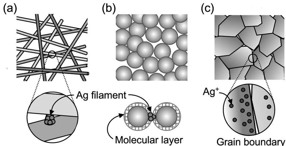
Fig. 13. Various physical reservoirs made of (a) nanowires, (b) nanoparticles, and (c) polycrystalline film.
