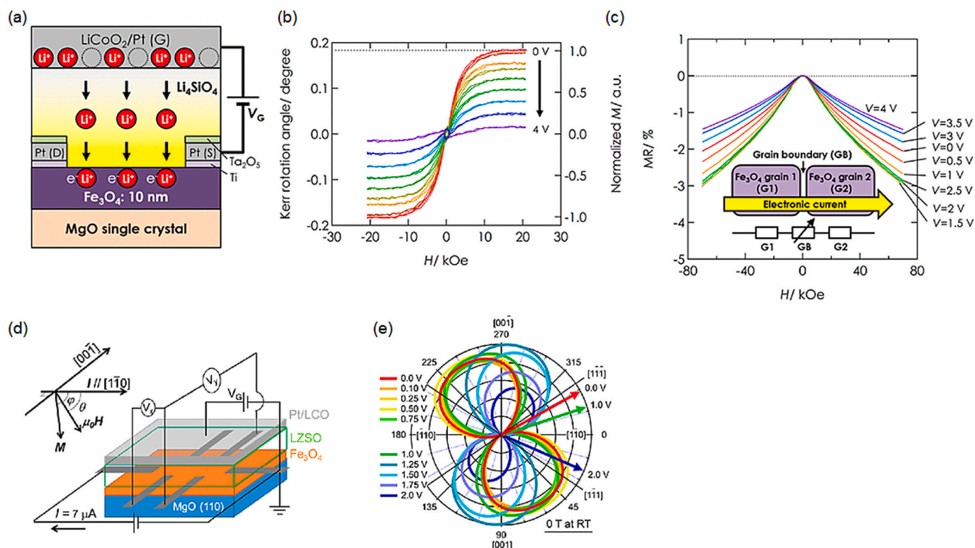
Fig. 27. (a) Schematic illustration of all-solid-state redox transistor with Fe 3 O 4 and LSO lithium ion conductor. Li + symbol represents positively charged lithium ions. Dotted circles in LiCoO 2 represent Li + ion vacancies. (b) M-H loops measured at various DC voltages. (c) DC voltage dependence of MR in Fe 3 O 4 thin film as a function of magnetic field (−70 to 70 kOe) at 250 K. Reprinted with permission from [112]. Copyright 2016 American Chemical Society. (d) Schematic illustration of an all-solid-state redox transistor and its configuration in a planar Hall measurement. V x and V y denote nano-volt meters for measuring longitudinal and transverse resistance. (e) Polar graph of MAF (magnetic anisotropy field) at various V G . The red, yellow-green, and blue arrows show the magnetization directions at V G = 0.0, 1.0, and 2.0 V, respectively. Reprinted with permission from Ref. [113]. Copyright (2020) American Chemical Society. (For interpretation of the references to colour in this figure legend, the reader is referred to the web version of this article.)
