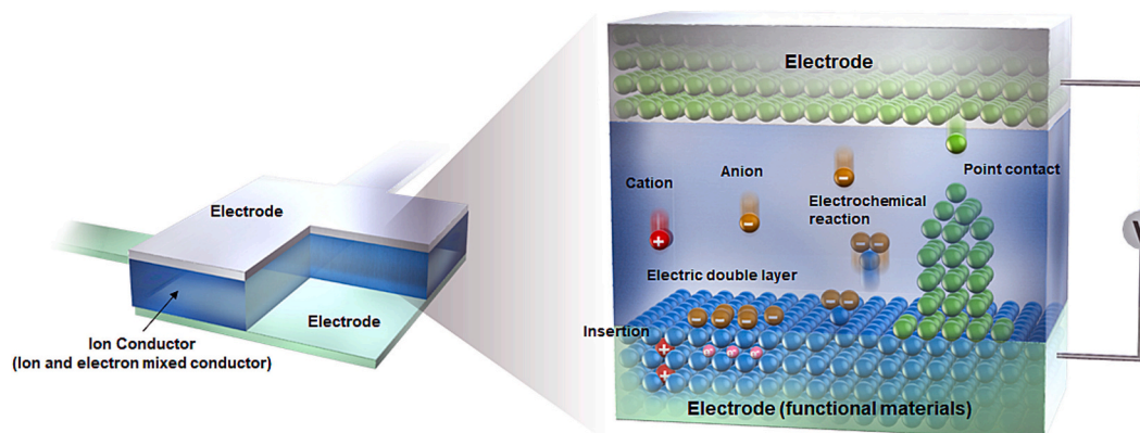
Fig. 1. Creation of solid-state ionic devices by using ionic nanoarchitectonics to create various properties and functions by exploiting localized ion transport and electrochemical phenomena. Reprinted with permission from Ref. 18. Copyright (2022) Wiley-VCH GmbH.
