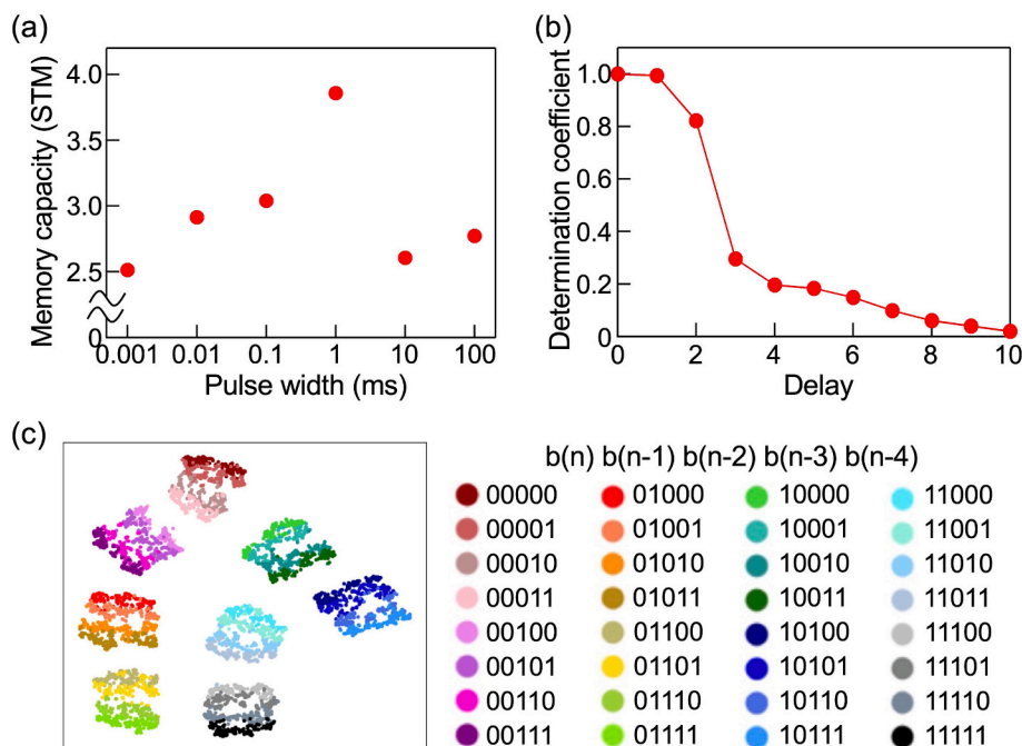
Fig. 16. Results of short-term memory task with \text{Ag}_2\text{S} -based reservoir. (a) Memory capacity measured as a function of pulse width. (b) Determination coefficient measured for a pulse width of 1 ms. (c) Distribution of output vectors visualized by t-distributed stochastic neighbor embedding (t-SNE). Reprinted with permission from Ref. [95]. Copyright 2024 The Japan Society of Vacuum and Surface Science.
