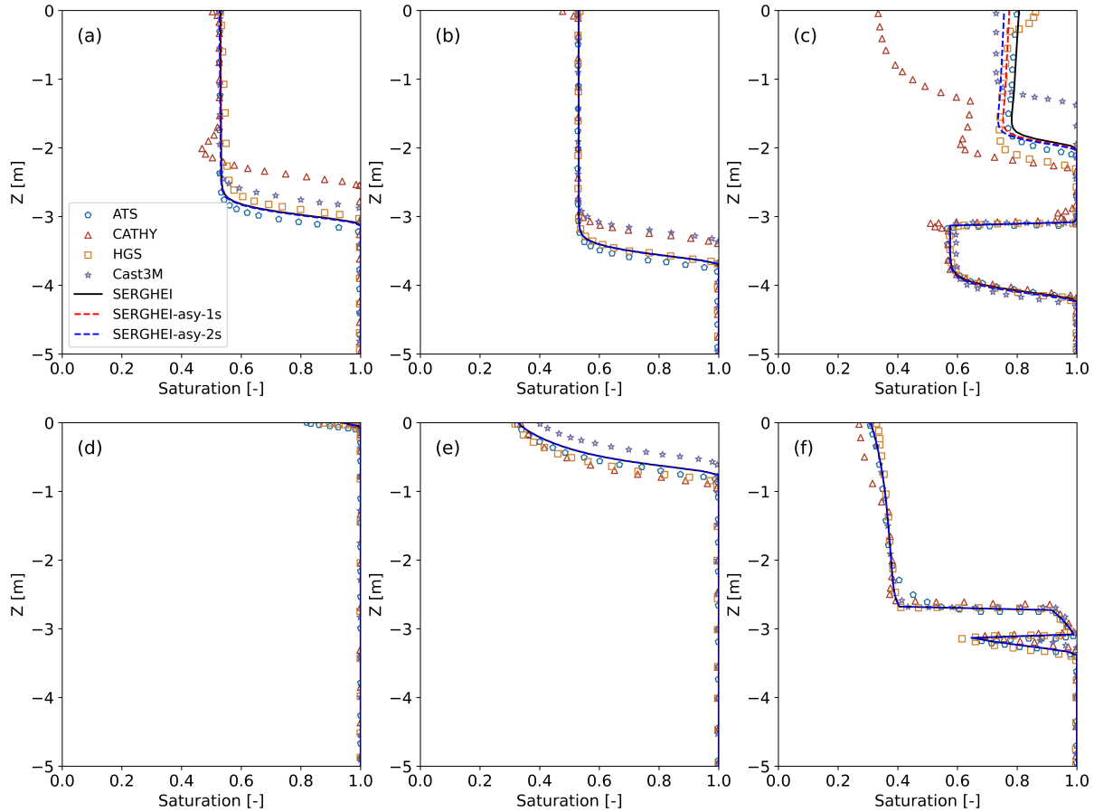
Figure 14. The simulated soil saturation profiles for (a)-(c) T=3 h and (d)-(e) T=6 h at X = 0, 8, 40 m. SERGHEI represents the synchronous calculation; SERGHEI-asy-1s and SERGHEI-asy-2s represent the asynchronous calculation with maximum time steps of 1s and 2s, respectively
