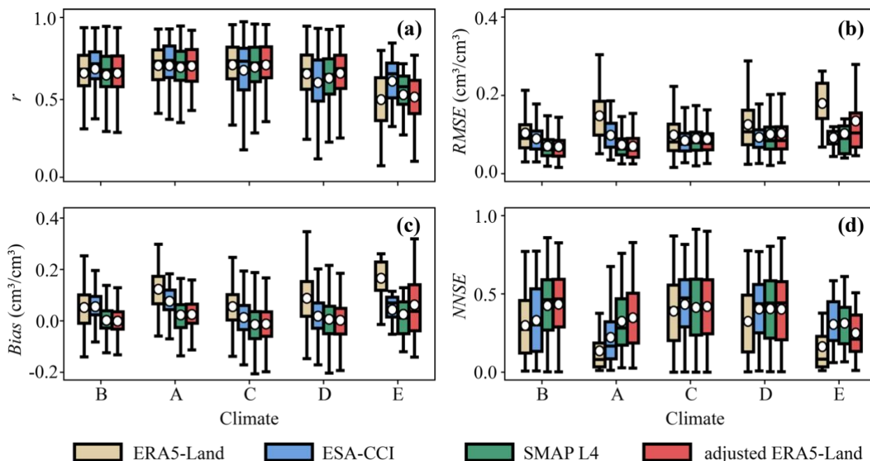
545 Figure 13. Distributions of four performance metrics, including (a) the Pearson correlation coefficient r , (b) RMSE , (c) Bias , and (d) NNSE from the comparison between in situ measurements and the four soil moisture products across different climate zones. The climate zones are categorized as A (Tropical), B (Arid), C (Temperate), D (Cold), and E (Polar). The classification of Zone B is based on precipitation and evaporation, whereas Zones A, C, D, and E are classified by temperature. Accordingly, the x-axis are ordered from the warmest to coldest (A, C, D, and E).
