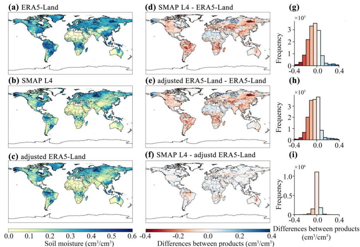
375 Figure 6. Spatial distribution of moisture dataset for an example date (January 1 st , 2016) and corresponding frequency distributions. (a-c) represent the spatial distributions of ERA5-Land, SMAP L4, and adjusted ERA5-Land, respectively. (d-f) show the spatial distributions of differences between (d) SMAP L4 minus ERA5-Land, (e) adjusted ERA5-Land minus ERA5-Land, and (f) SMAP L4 minus adjusted ERA5-Land. (g-i) provide frequency distributions corresponding to panels (d), (e), and (f), respectively.
