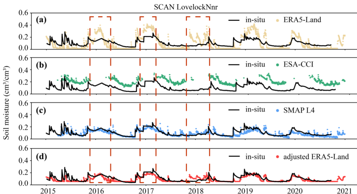
475 Figure 10. Data coverage and gaps at a representative station of SCAN LovelockNnr, Nevada, USA, comparing in situ observations with multiple soil moisture products. The time series of in situ soil moisture measurements is depicted as a solid black line, while corresponding estimates from the moisture products are shown as colored dots. Periods with missing data for the ESA-CCI dataset are highlighted by red dashed boxes.
