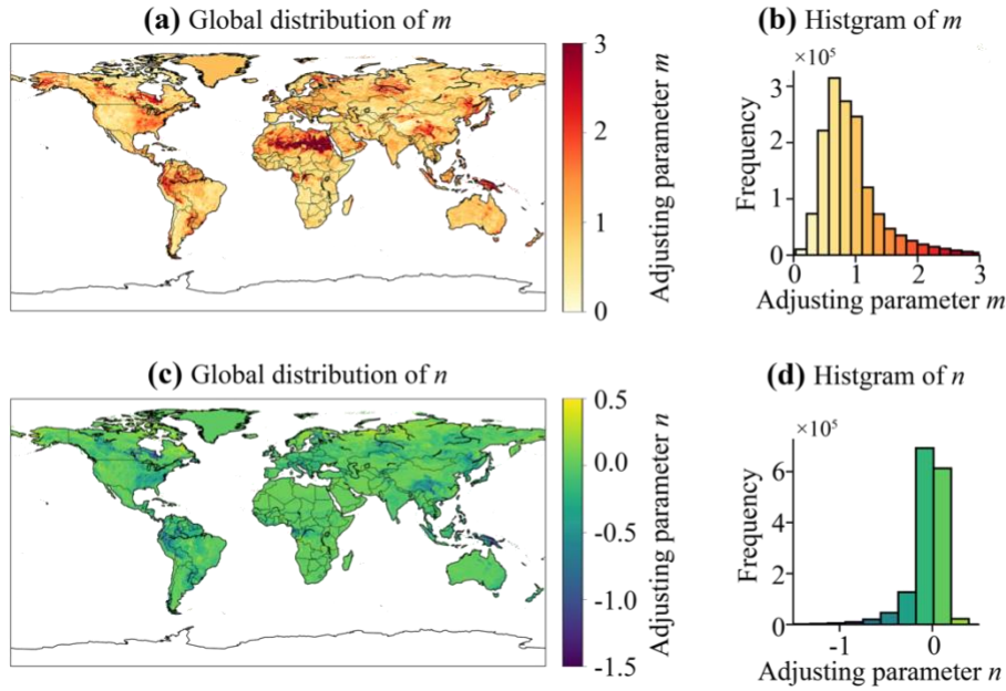
325 Figure 4. Global maps of adjusting parameter m and n used to adjust ERA5-Land dataset for SMAP L4 fusion, with histograms showing the frequency distribution of the parameters.
