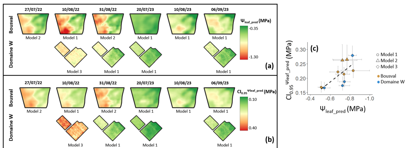
Figure 6. (a) Maps of \Psi_{\text{leaf\_pred}} predicted ( \Psi_{\text{leaf\_pred}} ) with the multiple linear regression model in both vineyards. (b) Maps of uncertainty in \Psi_{\text{leaf\_pred}} , quantified by the 95 % confidence interval on the prediction ( CI_{0.95}^{\Psi_{\text{leaf\_pred}}} ). \Psi_{\text{leaf\_pred}} at Bousval on 10 August 2022, 20 July 2023, 10 August 2023, and 6 September 2023 and at Domaine W on 31 August 2022, 20 July 2023, and 6 September 2023 was predicted with the model involving multispectral, thermal, and lidar data (model 1 in Table 5). \Psi_{\text{leaf\_pred}} at Bousval on 27 July and 31 August 2022 was predicted with the model involving multispectral and lidar data (model 2 in Table 5). \Psi_{\text{leaf\_pred}} at Domaine W on 10 August 2022 was predicted with the model involving thermal and lidar data (model 3 in Table 5). (c) The relation between \Psi_{\text{leaf\_pred}} and CI_{0.95}^{\Psi_{\text{leaf\_pred}}} . The points correspond to the median, and the horizontal and vertical bars respectively show the quartiles around \Psi_{\text{leaf\_pred}} and CI_{0.95}^{\Psi_{\text{leaf\_pred}}} . The dashed black line is the linear regression; the slope of this regression is different from 0 ( p value < 0.001).
