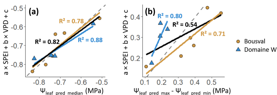
Figure 9. (a) Relation between median \Psi_{\text{leaf\_pred}} ( \Psi_{\text{leaf\_pred\_median}} ) and the linear combination of SPEI and VPD (Eq. 4 – a = 0.001 ; b = -0.13 ; c = -0.26 ). (b) Relation between the distribution of \Psi_{\text{leaf\_pred}} ( \Psi_{\text{leaf\_pred\_max}} - \Psi_{\text{leaf\_pred\_min}} ) and the linear combination of SPEI and VPD (Eq. 5 – a = -0.001 ; b = 0.08 ; c = -0.17 ). In each panel, the brown lines are the linear regressions on the brown circles, the blue lines are the linear regressions on the blue triangles, the black lines are the linear regressions on all points, and the dashed gray lines are the 1 : 1 lines.
