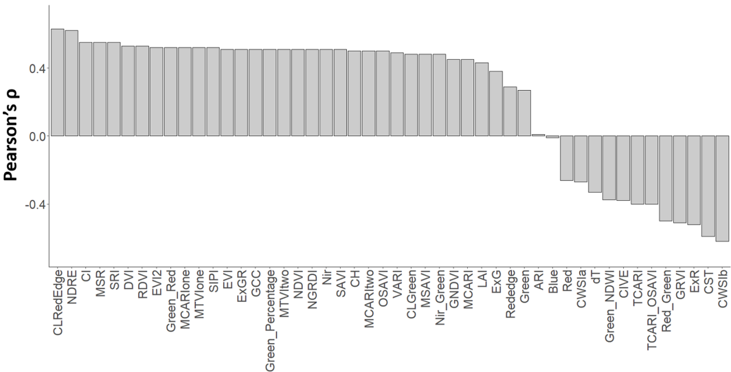
Figure 4. Pearson’s coefficient (Pearson’s \rho ) quantifying the linear correlation between measured \Psi_{\text{leaf}} ( \Psi_{\text{leaf\_meas}} ) and each vegetation index (VI) by taking all the measurements in both vineyards and at all dates.
