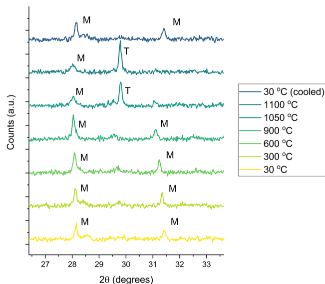
Fig. 5 | High temperature diffraction of 5 mol% Am-doped \text{ZrO}_2 . HT-PXRD of 5 mol% Am-doped \text{ZrO}_2 , where the transition from the m -( \text{Am}^{4+}_{0.011(7)}\text{Zr}^{4+}_{0.989(7)}\text{O}_2 ) phase (labelled M) can be observed to its tetragonal form (labelled T) reversibly between 900 and 1050 °C.
