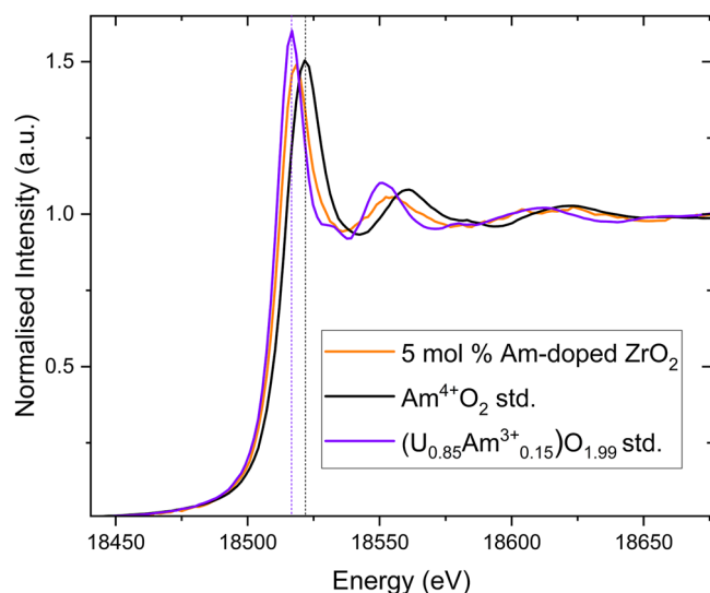
Fig. 4 | Normalised Am L_3 -edge spectra of the 5 mol% Am-doped \text{ZrO}_2 sample. Normalised Am L_3 -edge spectra of the 5 mol% Am-doped \text{ZrO}_2 sample measured with the standards \text{Am}^{4+}\text{O}_2 and (\text{U}_{0.85}\text{Am}^{3+}_{0.15})\text{O}_{1.99} . The vertical dashed black and purple lines correspond to the white line position of the \text{Am}^{4+}\text{O}_2 and (\text{U}_{0.85}\text{Am}^{3+}_{0.15})\text{O}_{1.99} standards for the \text{Am}^{4+} and \text{Am}^{3+} oxidation states, respectively.
