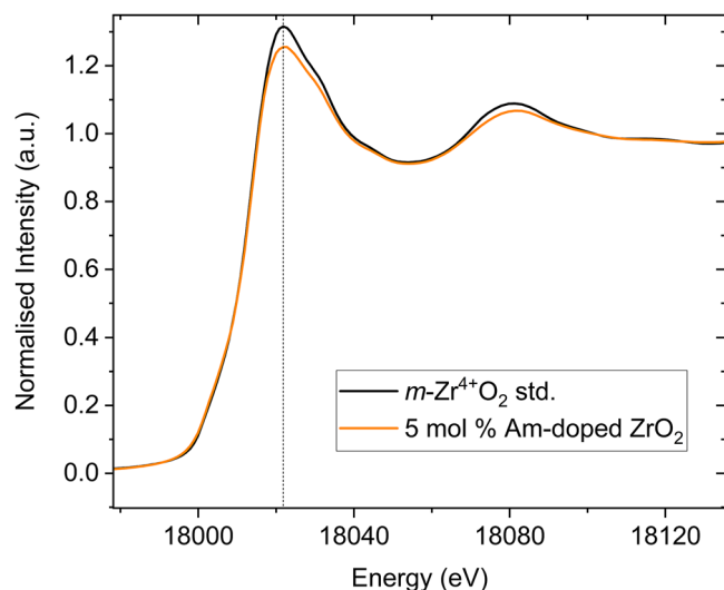
Fig. 3 | Normalised Zr K-edge XANES spectra of the 5 mol% Am-doped \text{ZrO}_2 sample. Normalised Zr K-edge XANES spectra of the 5 mol% Am-doped \text{ZrO}_2 sample with a m\text{-Zr}^{4+}\text{O}_2 standard. The vertical dashed black line corresponds to the white line position of the m\text{-Zr}^{4+}\text{O}_2 standard, representing the reference \text{Zr}^{4+} oxidation state.
