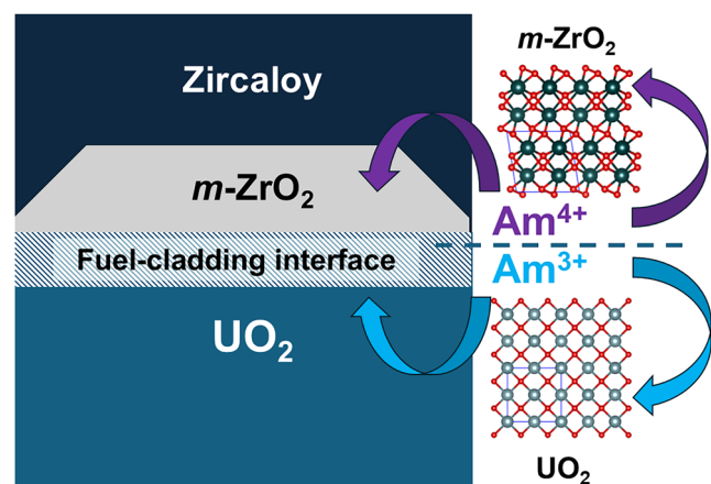
Fig. 6 | Schematic of reactions between Am redox states and m\text{-ZrO}_2 and \text{UO}_2 within Zircaloy cladded nuclear fuel at high burnup. Schematic of the inferred chemical interactions between m\text{-ZrO}_2 and Am redox states at the \text{UO}_2 fuel–Zircaloy cladding interface that can occur at higher fuel burnup, based on observations from this study.
