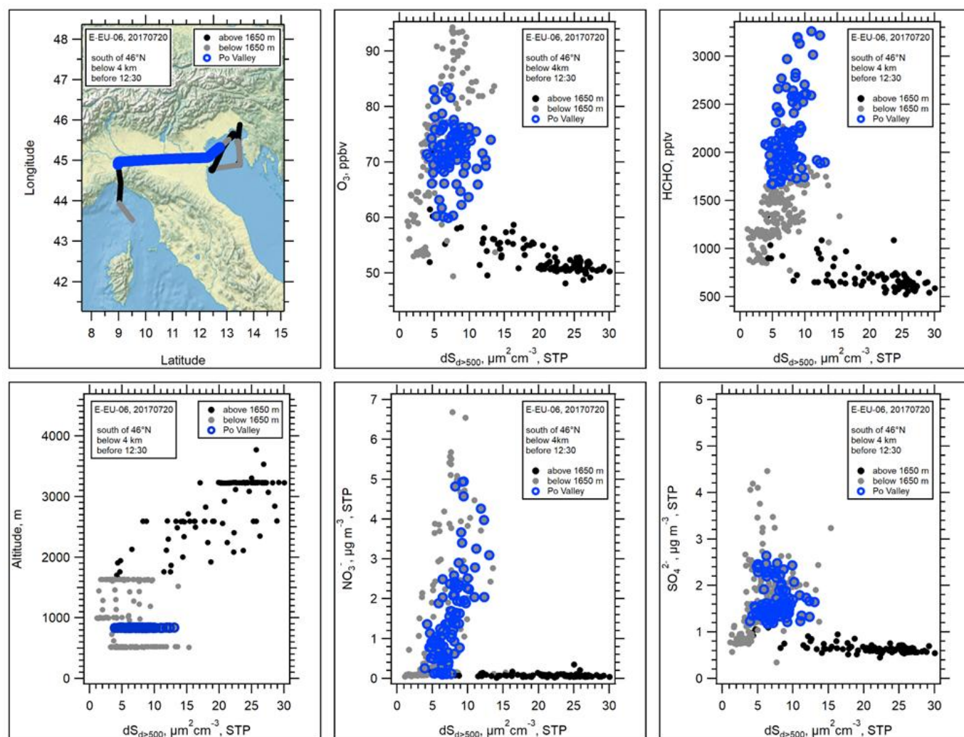
705 Figure 17: Relation between mixing ratios or mass concentrations of selected species ( O_3 , HCHO , NO_3^- , SO_4^{2-} ) and the surface area concentration of particles with diameter larger than 500 nm ( dS_{d>500nm} ) measured during E-EU-06 on July 20, 2017. On the left side, the flight location and the observed vertical distribution of particles are shown. Dots for flight altitudes below and above 1650 m are shown in grey and black respectively while the blue colour indicates the CPP crossing at 830-840 m. Public domain GIS data available in Wavemetrics IgorPro.
