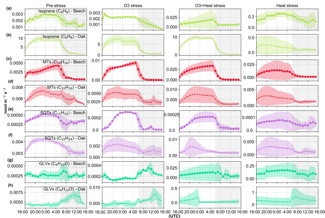
Figure 3. Diel variation in isoprene, monoterpene (MTs), sesquiterpene (SQTs), and green leaf volatile (GLVs) emissions from beech (a, c, e, g) and oak (b, d, f, h) under four conditions: pre-stress, O 3 stress, heat stress and O 3 + heat. On the x-axis, the unshaded region (16:00–06:00 UTC) corresponds to the plants’ daytime (lights on), while the grey shaded region represents the plants’ nighttime (lights off). Data points are diel averages and shaded areas around them represent the standard deviation. A version of this figure that is normalized to the maximum diel emission is presented in the Supplement (Fig. S7).
