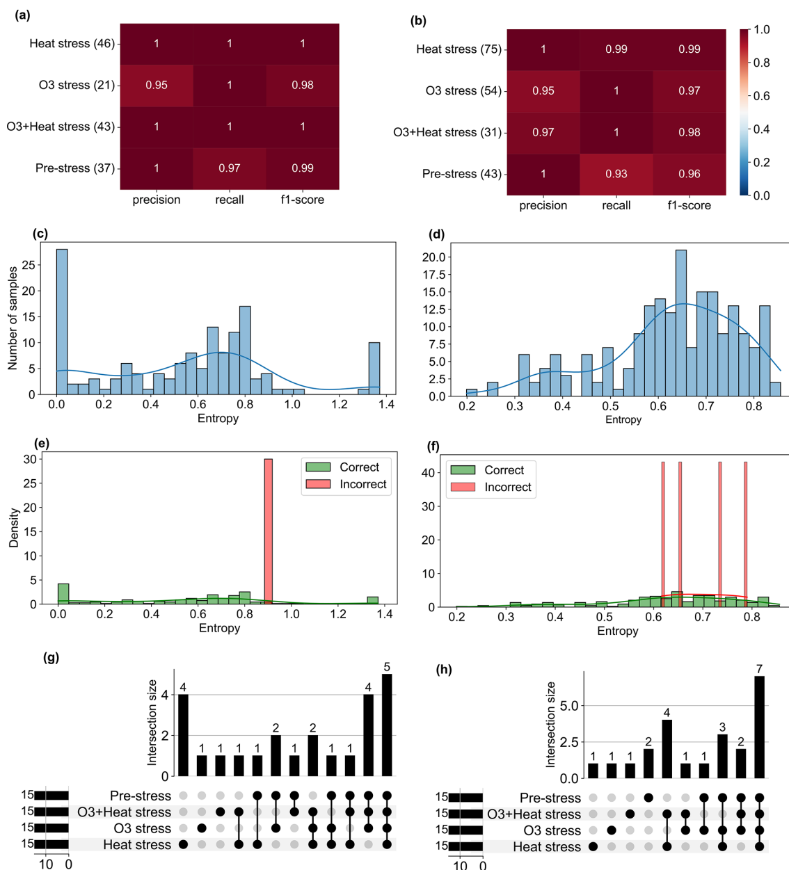
Figure 6. Performance metrics, uncertainty, and misclassification analysis of the Random Forest model for stress classification in (left) beech and (right) oak. (a–b) Precision, recall, and F_1 -score for each stress class based on the test set. Numbers in parentheses indicate the number of test samples per class. (c–d) Distribution of Shannon entropy values of predicted class probabilities across all test samples. (e–f) Entropy distributions of correctly and incorrectly classified samples. (g–h) Plots showing intersections of SHAP-identified top 15 stress markers among the four stress classes. Bars represent the number of ions unique to or shared between classes. Insets indicate total counts.
