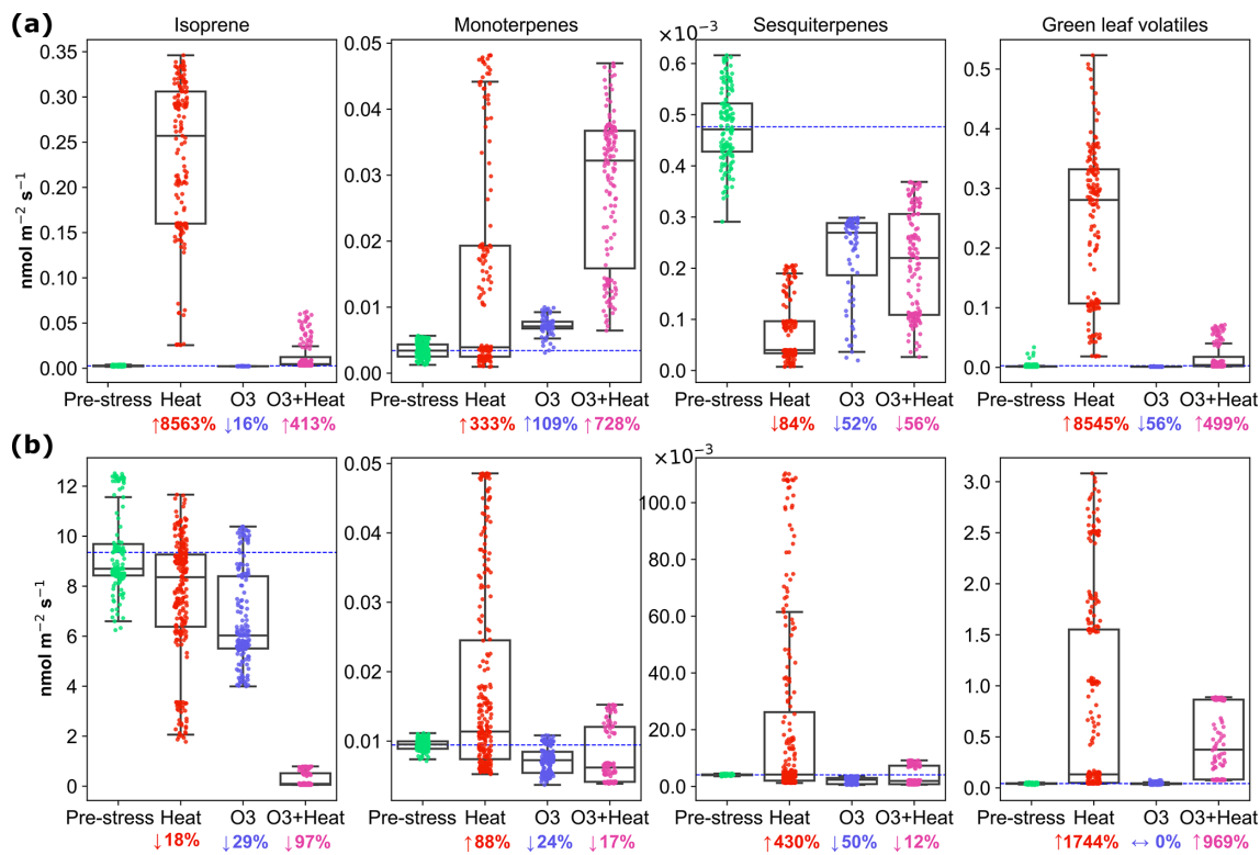
Figure 2. Emissions of isoprene, monoterpene, sesquiterpene, and green leaf volatile emissions from (a) beech and (b) oak under pre-stress, heat, O 3 , and combine stress (O 3 + heat) conditions. Boxes represent interquartile ranges, horizontal lines indicate medians, and whiskers show the data spread. The dashed horizontal blue line represents the average pre-stress emission level for reference. Percent changes compared to average pre-stress levels are indicated by ↑ = increase, ↓ = decrease, ↔ = no change.
