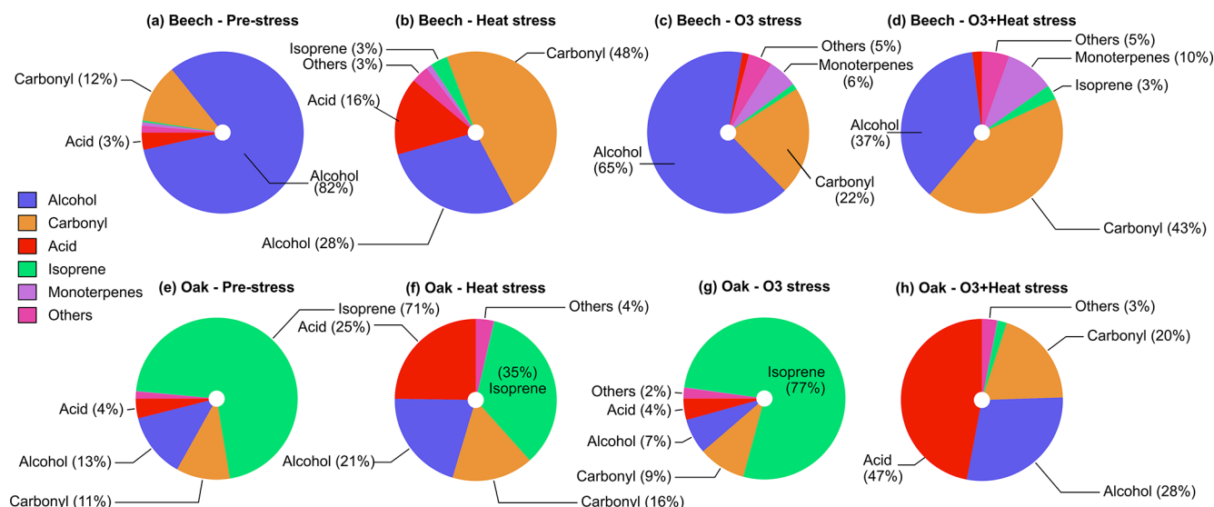
Figure 4. Composition (mole-based) of volatile organic compound classes emitted by (a–d) beech and (e–h) oak under different environmental stress conditions.
