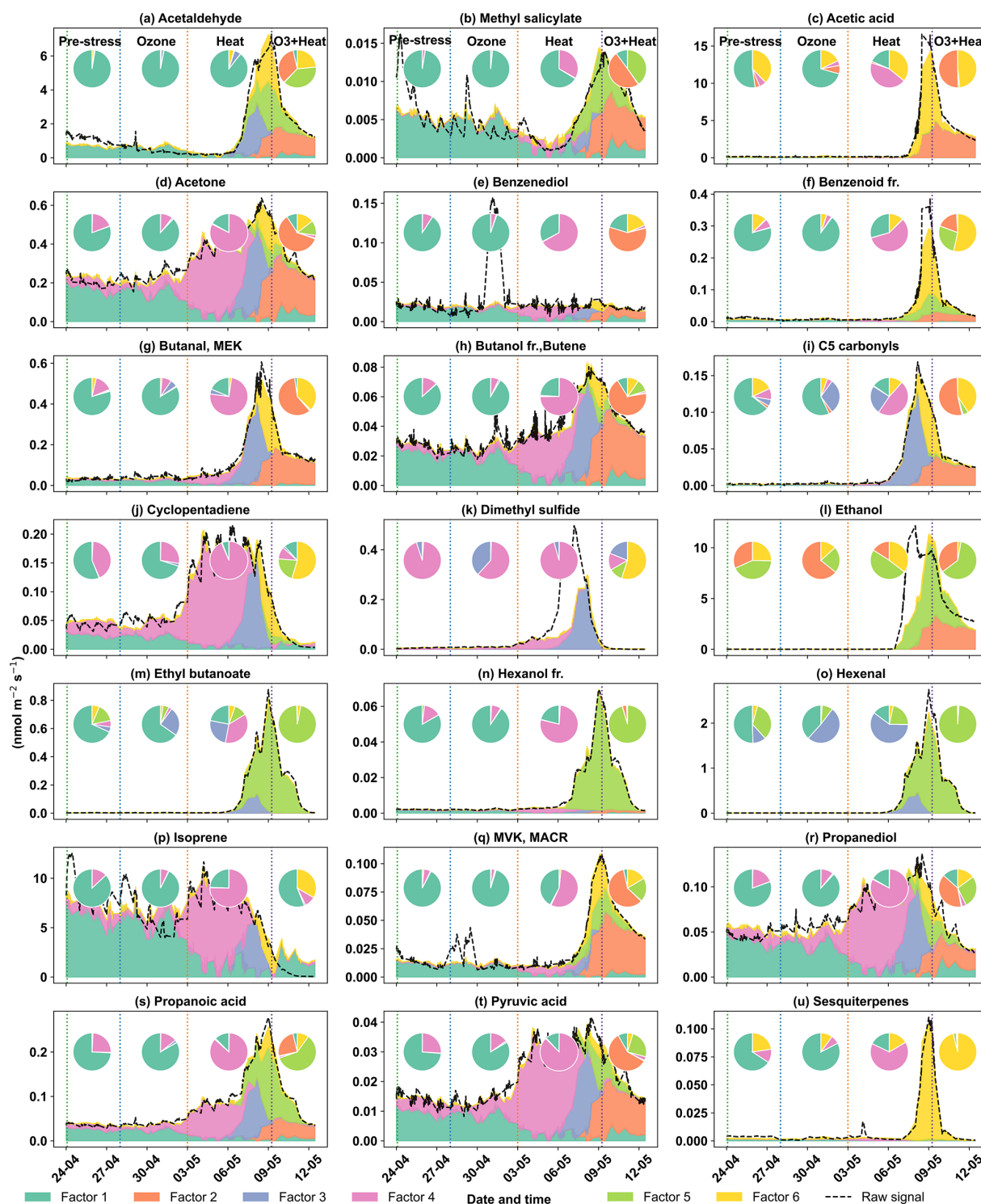
Figure B4. Stacked time series of PMF-resolved contributions for selected BVOC compounds during the Oak experiment. The black dashed lines indicate the original concentration of specific compounds, while stacked colored areas represent contributions from the six PMF-resolved factors. Each compound's emission is displayed across the four stress periods (Pre-stress, O 3 stress, O 3 + Heat stress, Heat stress), separated by vertical dashed lines. Inset pie charts show the relative contribution of each factor to compound emissions within each stress period, as a factor dominance.
