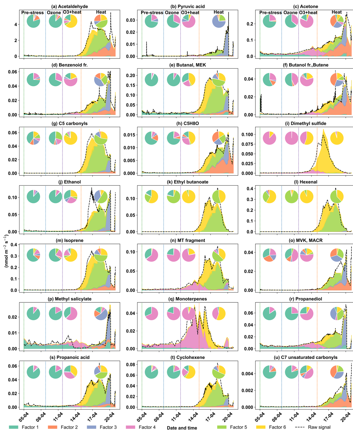
Figure B2. Stacked time series of PMF-resolved contributions for selected BVOC compounds during the Beech experiment. The black dashed lines indicate the original concentration of specific compounds, while stacked colored areas represent contributions from the six PMF-resolved factors. Each compound's emission is displayed across the four stress periods (Pre-stress, O 3 stress, O 3 + Heat stress, Heat stress), separated by vertical dashed lines. Inset pie charts show the relative contribution of each factor to compound emissions within each stress period, as a factor dominance.
