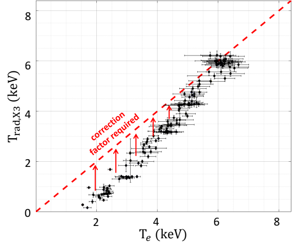
Figure 6. Comparison of X3 radiation temperature versus T_e from TS, demonstrating the influence of the optical depth on the measurement. Reproduced with permission from [23].
