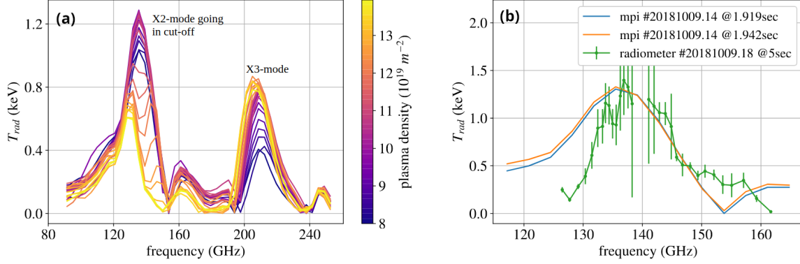
Figure 2. (a): measurement of T_{\text{rad}} for 2 nd - and 3 rd -harmonic X-mode, demonstrating the cut-off effect for increasing density in the 2 nd -harmonic. (b): the comparison of T_{\text{rad}} estimated from Michelson and ECE-radiometers, showing a good agreement. Reproduced from [11]. The Author(s). CC BY 4.0.
