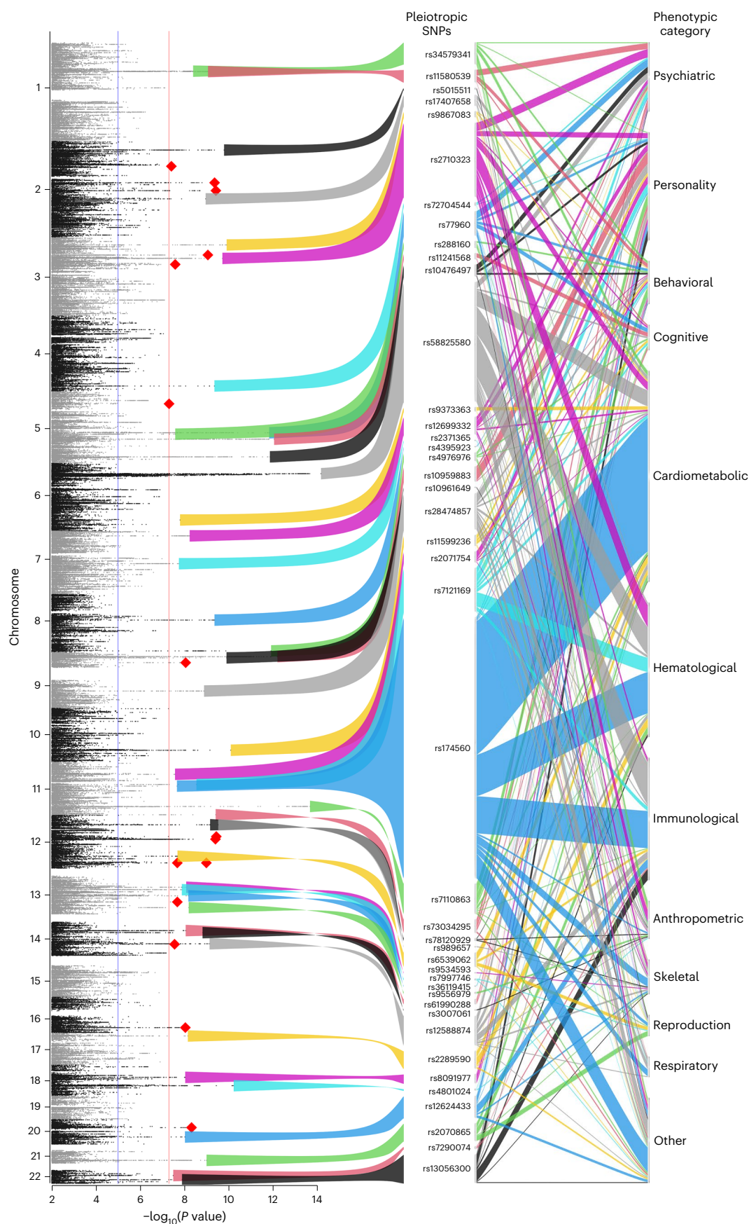
Fig. 3 | Overview of SNP associations with other phenotypes. The (rotated) Manhattan plot of the -\log_{10}(P \text{ values}) of the ANX meta-analysis (left; as in Fig. 1) and PheWAS alluvial plot of potentially pleiotropic variants (right). The colored ribbons depict variants that are associated with at least one other published
