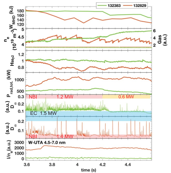
Figure 4. Impact of W limiter boron coverage on H-mode performance in EAST; Type II ELMy H-modes (132383 in green) with high B cover perform much better than Type I ELMy H-modes (132829 in red) with low boron cover (both discharges have an 8 cm separatrix—W limiter distance, P_{NBI} = 1.2\text{--}1.4 MW, P_{ECH} = 1.5 MW). Reproduced from the 50 th EPS conference with permission from [Jia2024].
