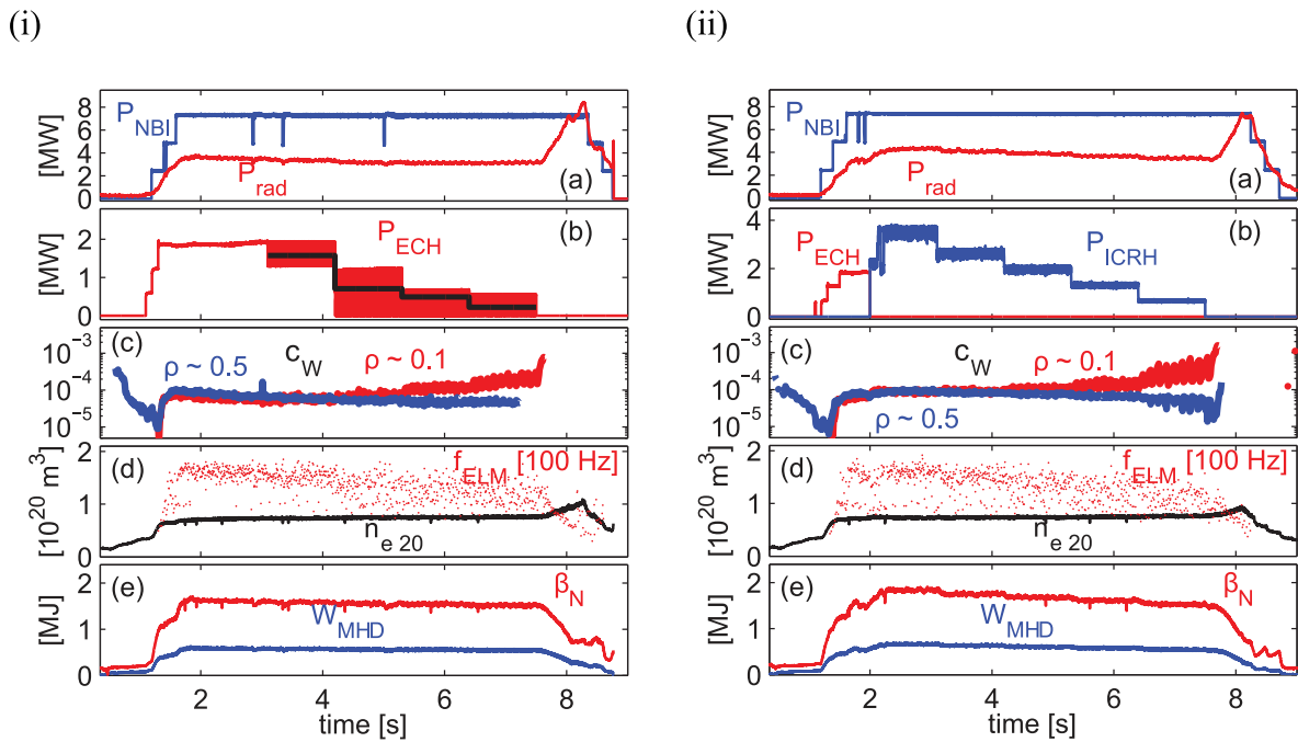
Figure 8. Time traces of ASDEX Upgrade shot (i —32408 and ii —32404) with decreasing steps of ECH and ICH, respectively: (a) total NBI and radiated powers, (b) total ECH and ICH powers, (c) W concentration c_W at normalised minor radius ( \rho = r/a ) \rho \sim 0.1 and \rho \sim 0.5 , (d) ELM frequency and line averaged density, (e) normalised \beta and total stored energy. Reproduced from [Angioni2017]. © 2017 IAEA, Vienna.
