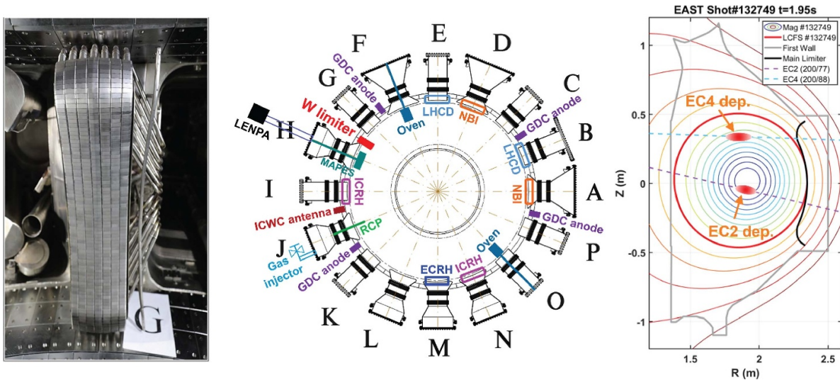
Figure 18. Left: photograph at pre-installation of the EAST actively cooled outer poloidal W limiter (based on a monoblock/plasma-facing unit design similar to the components used in the ITER divertor and the EAST upper divertor). Centre: toroidal cross-section of the EAST tokamak, indicating locations of the outer W limiter, heating systems, GDC and ICWC electrodes and selected diagnostics. Right: poloidal cross-section showing the magnetic equilibrium of the typical outer limiter circular plasma used in the EAST start-up experiments with positions of central and off-axis ECH deposition [Pitts2025, Gong2024]. Reproduced with permission from [Pitts2025]. CC BY-NC-ND 4.0.
