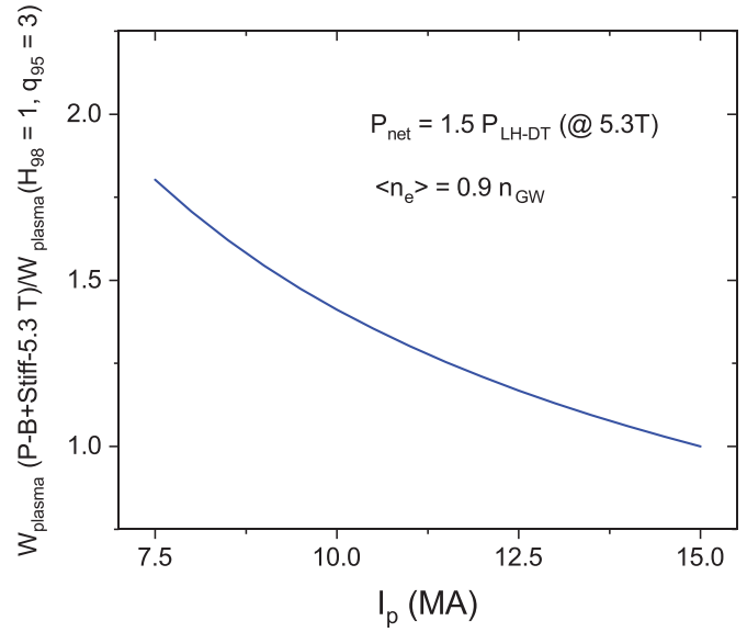
Figure 57. Ratio of the plasma energy evaluated with the H_{98y,2} scaling law with q_{95} = 3 and an alternative approach assuming an additional dependence T \sim B_t^{0.84} , versus I_p for ITER H-modes with \langle n_e \rangle \sim 0.9 n_{GW} and with P_{net} = P_{tot} - P_{rad} = 1.5 P_{LH-DT} (@ 5.3 T) .
