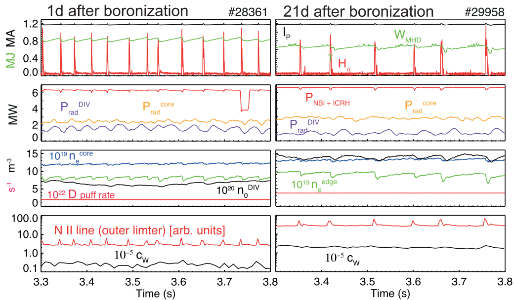
Figure 6. Comparison of ITER Baseline ASDEX Upgrade discharges heated by NBI + ICH during phases of 0.5 s duration. Discharge parameters are identical except gas puff and ‘freshness’ of boronisation. While the discharge on the left (#28361) was conducted 1 d after a boronisation, the one on the right (#29958) was executed 21 d after a boronisation. Different gas puff levels 1.9 \times 10^{22} and 3.8 \times 10^{22} atoms s^{-1} were necessary to reach stationarity for discharges #28361 and #29958, respectively, which lowers the plasma energy in discharge #29958. Reproduced from [Schweitzer2016]. © 2016 IAEA, Vienna.
