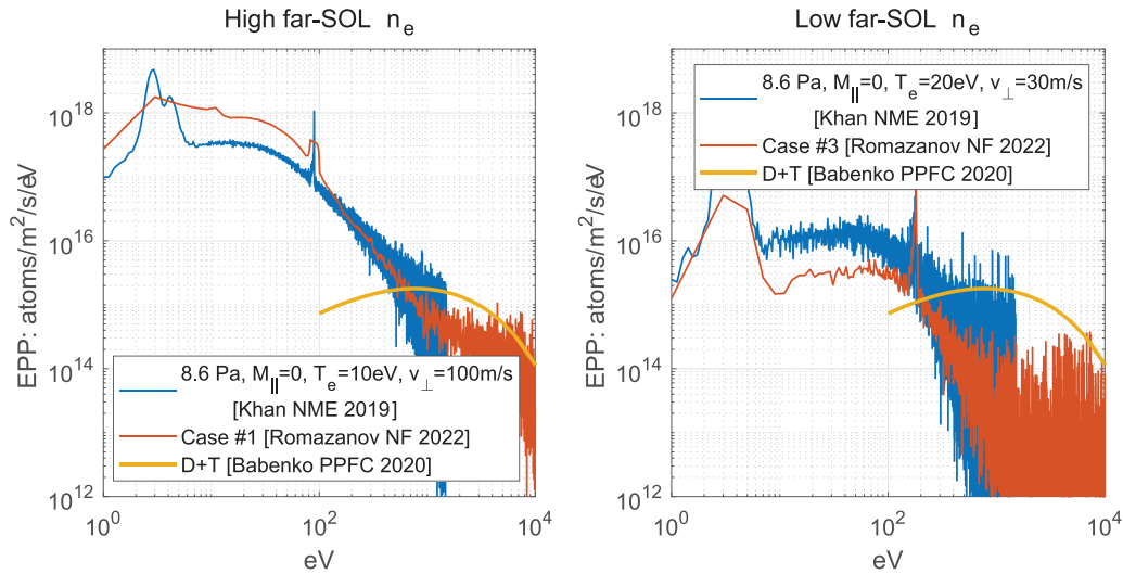
Figure 59. Eirene and DOUBLE-MC calculated CXN neutral energy spectra for ITER Q \geq 10 plasma conditions [Khan2019, Romazanov2022, Babenko2020]. The lower flux at higher energy in the EIRENE spectra is due to SOL neutral screening, which is absent in the DOUBLE-MC code since the latter does not include the SOL plasma in the evaluation of neutral wall fluxes.
