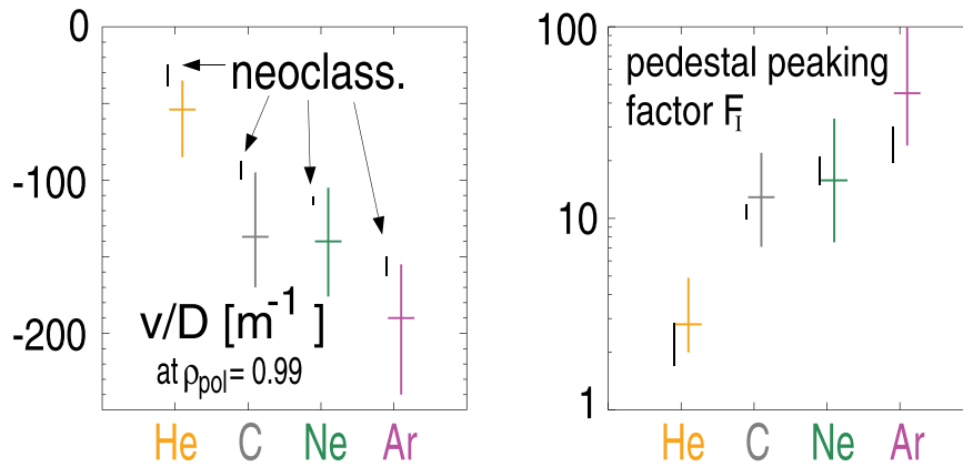
Figure 12. Measured and modelled (assuming neoclassical transport) inverse scale lengths for a range of impurities in the ASDEX upgrade pedestal and resulting pedestal peaking (namely the ratio of the impurity density at the top of the pedestal and at the separatrix). Reprinted from [Pütterich2011], Copyright (2011), with permission from Elsevier.
