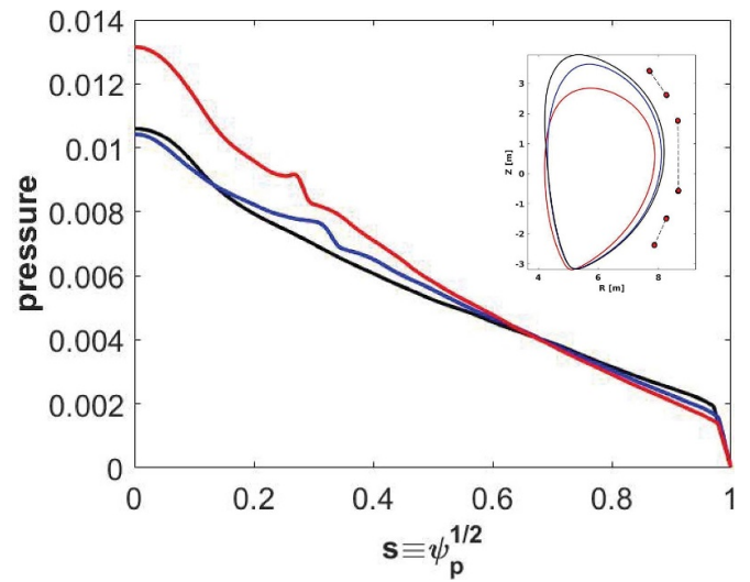
Figure 43. Plasma configurations for DINA 5 MA/2.65 T \langle n_e \rangle \sim 0.5 n_{GW} , P_{ECH} = 40 MW, DD H-mode plasma scenarios in the flat-top phase (reference baseline configuration-black, increased overall wall clearance (15 cm at the outer midplane) configuration-blue and 45 cm outer gap configuration-red) and associated normalised plasma pressure profiles (pressure normalised by B_0^2/\mu_0 , B_0 = 2.65 T) modelled versus square root normalised poloidal flux with JINTRAC including edge MHD plasma stability modelling. Reproduced from [Bai2024]. © IOP Publishing Ltd. All rights reserved. Reference baseline (IMAS SIMDB: 55666971-00d2-11f0-a5a7-9440c9e76fd0); increased overall clearance (IMAS SIMDB: b08e443a-00d3-11f0-88a3-9440c9e76fd0); 45 cm outer gap (69e5f567-00d4-11f0-b236-9440c9e76fd0).
