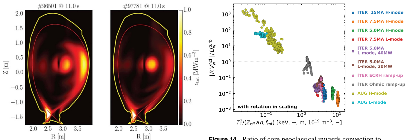
Figure 14. Ratio of core neoclassical inwards convection to turbulent diffusion in typical plasma conditions in ASDEX Upgrade (AUG) and ITER against a scaling derived on the basis of integrated transport studies. Reproduced from [Fajardo2024a]. CC BY 4.0. This scaling parameter depends on ion temperature ( T_i ), effective charge ( Z_{\text{eff}} ), minor radius ( a ), ion density ( n_i ) and a parameter ( f_{\text{rot}} ) that depends on plasma toroidal rotation, which impacts W transport due to neoclassical effects.
