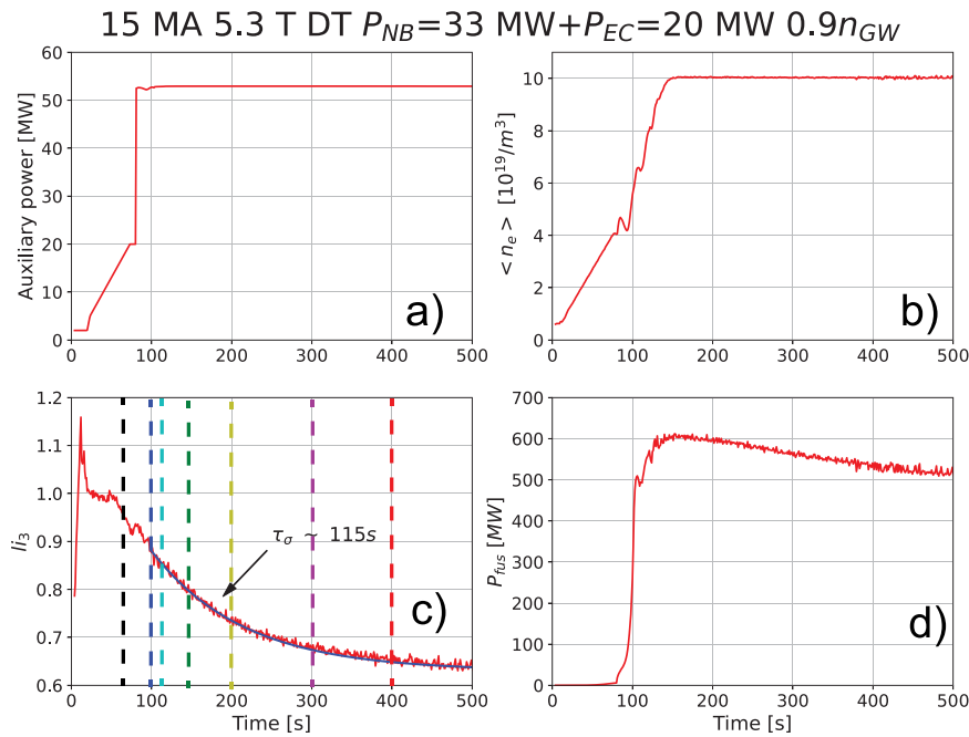
Figure 65. Time evolution of plasma parameters in JINTRAC core-edge integrated simulations of Q \geq 10 plasmas in ITER: (a) auxiliary power, (b) electron average density, (c) plasma internal inductance ( l_{i3} ) (vertical dashed lines correspond to those for which the q profile is shown in figure 64) and, (d) Fusion power [Köchli2018, Köchli2020] (IMAS SIMDB: 8c9575de-ff9e-11ef-a181-9440c9e76fd0, 9e4eaca5-ff9f-11ef-a979-9440c9e76fd0, 3d87dedc-ffa0-11ef-8eee-9440c9e76fd0).
