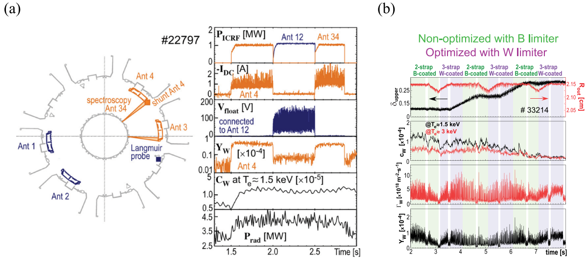
Figure 9. (a) Characterisation of the W release during ICH power input from antenna pairs 12 and 34 for shot #22797 before boronisation in ASDEX Upgrade with non-optimised (2-strap) antennas. Reproduced from [Bobkov2010]. © 2010 IAEA, Vienna. (b) Comparison of the B-coated antennas with the W-coated antennas during scans of plasma triangularity and the radial position in deuterium plasmas in ASDEX Upgrade. Every antenna pair provides P_{ICH} = 1.5 MW in the highlighted time windows on top of P_{aux} = 6.3 MW. The non-optimised (2-strap) antennas are B-coated and the optimised (3-strap) antennas are W-coated. Reproduced from [Bobkov2017]. © IOP Publishing Ltd. All rights reserved.
