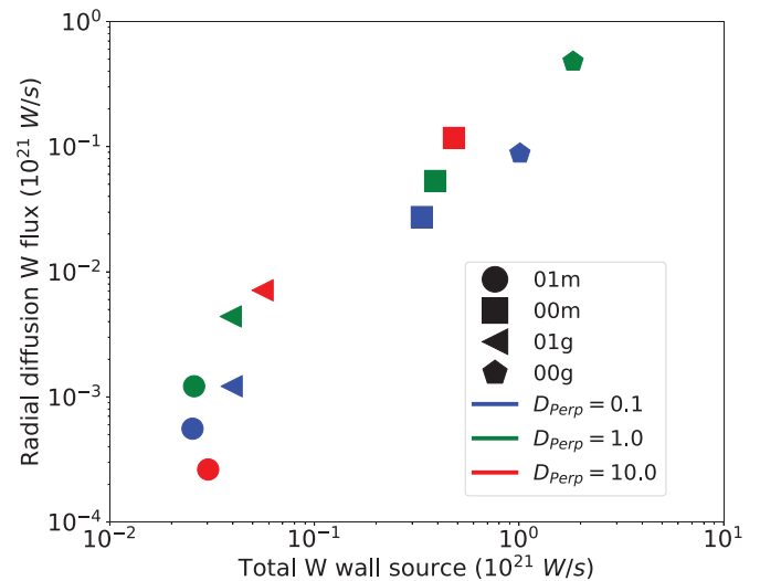
Figure 58. WallDYN modelled radial diffusion driven flux of W across the edge modelling calculation grid boundary for ITER Q \geq 10 plasmas versus total W wall source, which includes influx due to erosion and reflection from both main chamber wall and divertor for a range of far-SOL W transport diffusion coefficients. Reproduced from [Schmid2024]. CC BY 4.0.
