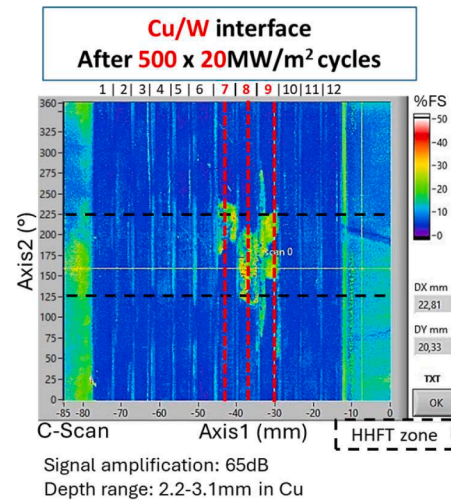
Fig. 11. Cu/W joining interface of MU II -IJS after 500 \times 20\text{MW}/\text{m}^2 cycles (2.2–3.1 mm depth range in Cu). A large discontinuity affects the loaded zone of monoblocks #7–8–9. The red dotted lines are circumferential paths used for a more detailed investigation of the morphology and depth of the defect.
