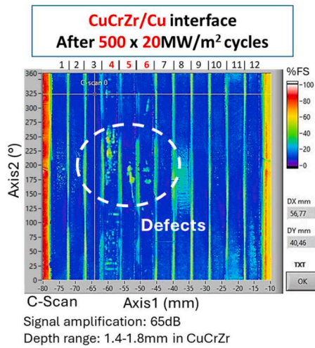
Fig. 10. CuCrZr/Cu joining interface of MU II -IJS after 500 \times 20\text{MW}/\text{m}^2 cycles. The presence of clustered discontinuities on monoblock #4–5–6 is highlighted in the C-scan (1.4–1.8 mm depth range in CuCrZr).
