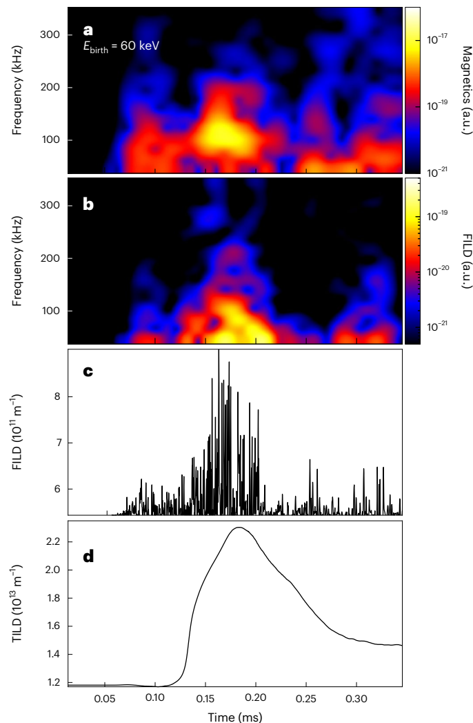
Fig. 6 | Synthetic diagnostics for the multi- n hybrid kinetic-MHD simulation. a,b , Spectrograms of radial magnetic field fluctuations ( \partial B_r / \partial t ) ( a ) and fast-ion losses ( b ) measured at the low field side (LFS) midplane measured by a synthetic FILD. c , The temporal evolution of the measured ELM-induced fast-ion losses. d , The temporal evolution of thermal particle losses to the outer divertor measured by a synthetic thermal ion loss detector (TILD). In a–d , the NBI energy is E_{\text{birth}} = 60 \text{ keV} .
