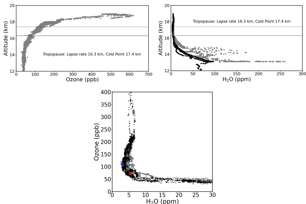
Figure 3. Measurements of ozone (top left) and water vapour (top right) versus altitude in the vicinity of the tropopause for the scientific flight on 8 August 2017. The dashed line shows the altitude of the lapse rate tropopause and the dotted line the altitude of the cold point tropopause. Tropopause information is for the first three hours of the flight (see Table 1), ozone and water vapour measurements are for the entire flight. In top right panel and in the scatter plot in the bottom panel, grey symbols indicate the FISH total water vapour measurements and black points show the gas-phase water vapour measurements by the FLASH instrument. The red symbol in the bottom panel indicates the location of the lapse rate tropopause; the blue symbol the location of the cold point tropopause.
