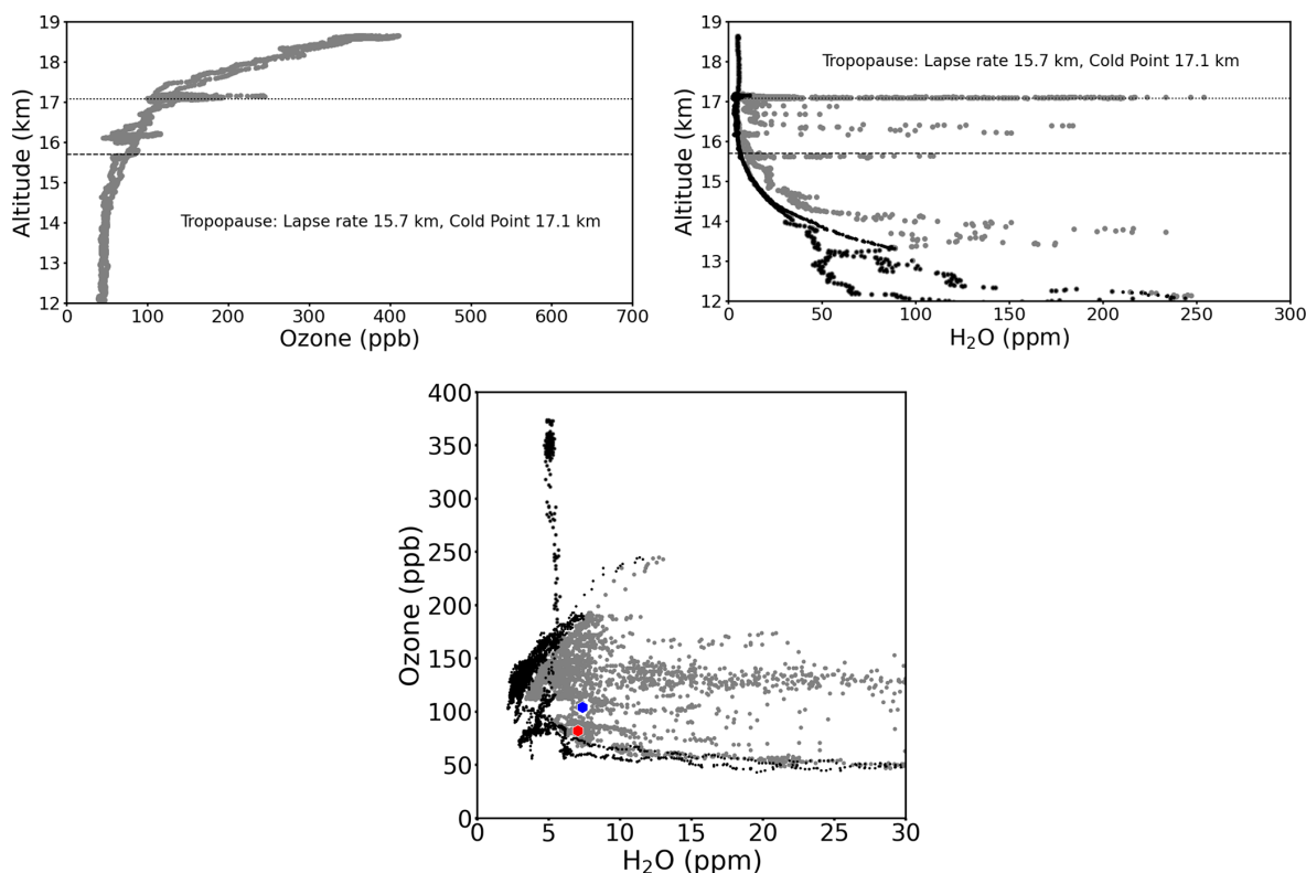
Figure 5. Measurements of ozone (top left) and water vapour (top right) versus altitude in the vicinity of the tropopause for the scientific flight on 10 August 2017. The dashed line shows the altitude of the lapse rate tropopause and the dotted line the altitude of the cold point tropopause. Tropopause information is for the first three hours of the flight (see Table 1), ozone and water vapour measurements are for the entire flight. In top right panel and in the scatter plot in the bottom panel, grey symbols indicate the FISH total water vapour measurements and black points show the gas-phase water vapour measurements by the FLASH instrument. The red symbol in the bottom panel indicates the location of the lapse rate tropopause; the blue symbol the location of the cold point tropopause.
