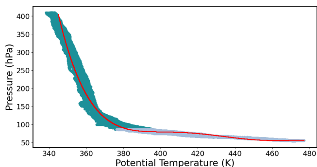
Figure A2. The relation between pressure and potential temperature for all science flights from Kathmandu (dark). Measurements above the (mean) cold point tropopause are shown in light blue. Red line shows an empirical fit to the data for potential temperature greater than 350 K.
