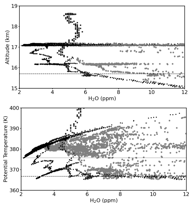
Figure 6. Water vapour versus altitude (top) and versus potential temperature (bottom) in the vicinity of the cold point and the lapse rate tropopause for the scientific flight on 10 August 2017 (similar as in Fig. 5, top right, but for a reduced range of observed water vapour values). The dotted line shows the cold point for this flight (17.1 km, top, and 375.8 K, bottom) and the dashed line the lapse rate tropopause (15.7 km, top, and 366.7 K, bottom). Grey symbols indicate the FISH total water vapour measurements and black points show the gas-phase water vapour measurements by the FLASH instrument. The aircraft measurements extend to about 420 K.
