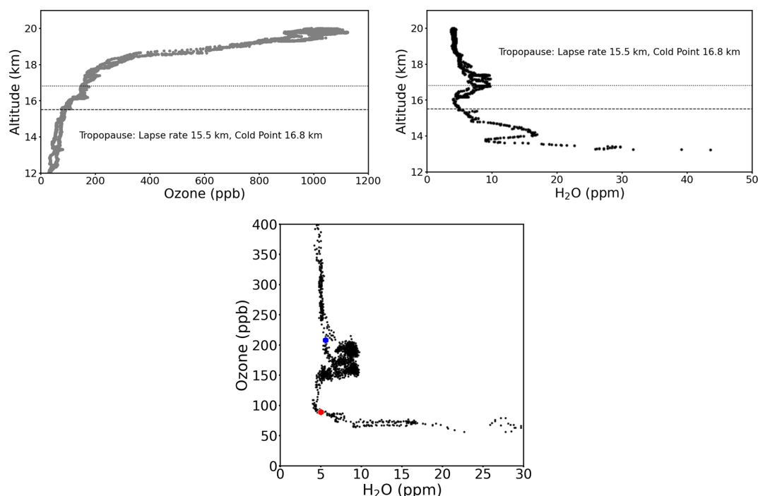
Figure 2. Measurements of molar mixing ratios of ozone (top left) and water vapour (top right) versus altitude in the vicinity of the tropopause for the scientific flight on 29 July 2017. The dashed line shows the altitude of the lapse rate tropopause and the dotted line the altitude of the cold point tropopause. Bottom panel shows a scatter plot of the aircraft measurements of ozone and water vapour on 29 July 2017. The red symbol indicates the location of the lapse rate tropopause; the blue symbol the location of the cold point tropopause. Tropopause information is for the first three hours of the flight (see Table 1), ozone and water vapour measurements are for the entire flight. In the top right and bottom panel, grey symbols indicate the FISH total water vapour measurements and black points show the FLASH gas-phase water vapour measurements. Note that for this flight the FISH and FLASH water vapour measurements are very similar (top right and bottom panel), in other words no cloud particles were observed.
