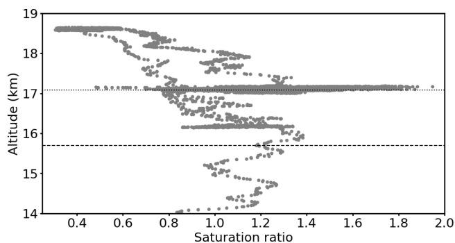
Figure 7. Saturation ratio of \text{H}_2\text{O} over ice versus altitude for the scientific flight on 10 August 2017 in the vicinity of the cold point and the lapse rate tropopause. Gas-phase \text{H}_2\text{O} measurements are from the FLASH instrument; these measurements are used to calculate the water vapour saturation ratio. The dotted line shows the cold point for this flight (17.1 km) and the dashed line the lapse rate tropopause (15.7 km). The top altitude for which FISH observed ice particles is 17.1 km. (See Supplement for a figure showing potential temperature as the vertical axis.)
