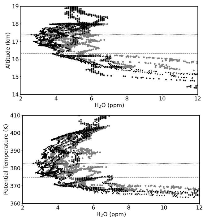
Figure 4. Water vapour versus altitude (top) and versus potential temperature (bottom) in the vicinity of the tropopause for the scientific flight on 8 August 2017 (similar as in Fig. 3, top right), but for a reduced range of observed water vapour values. The dotted line shows the cold point for this flight (17.4 km, top, and 382.6 K, bottom) and the dashed line the lapse rate tropopause (16.3 km, top, and 374.8 K, bottom). Grey symbols indicate the FISH total water vapour measurements and black points show the gas-phase water vapour measurements by the FLASH instrument. The aircraft measurements extend to about 440 K.
