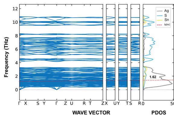
Fig. 3 Computed phonon band structure along the partial phonon density of states for the room-temperature phase of the \text{Ag}_8\text{SnS}_6 canfieldite. Here, the dotted red line at 1.62 \text{ THz} corresponds to the acoustic Debye frequency ( \omega_{\text{AC}} ).
