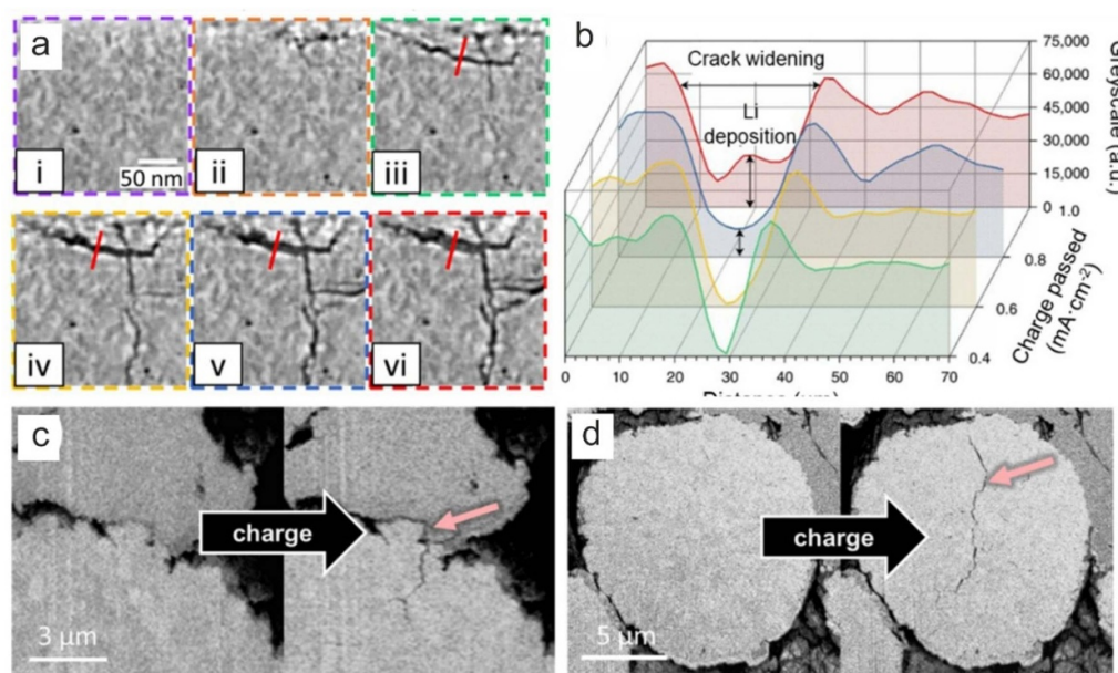
Figure 17. (a) In situ phase-contrast X-ray computed tomography (XCT) of virtual cross-sections during a single plating event in a LiLPSCl/Li cell; (b) analysis of lithium deposition showing that cracks propagate ahead of Li. (a), (b) Reproduced from [332] with permission from Springer Nature. Operando focused ion beam (FIB)-SEM cross-section of a composite containing LiNi 0.6 Mn 0.2 Co 0.2 O 2 (NMC622) and amorphous Li 3 PS 4 (LPS), highlighting (c) decohesion of the active material from the ionic network and (d) intergranular fracturing of the polycrystalline active material. (c), (d) Reprinted (adapted) with permission from [335]. Copyright (2024) American Chemical Society.
