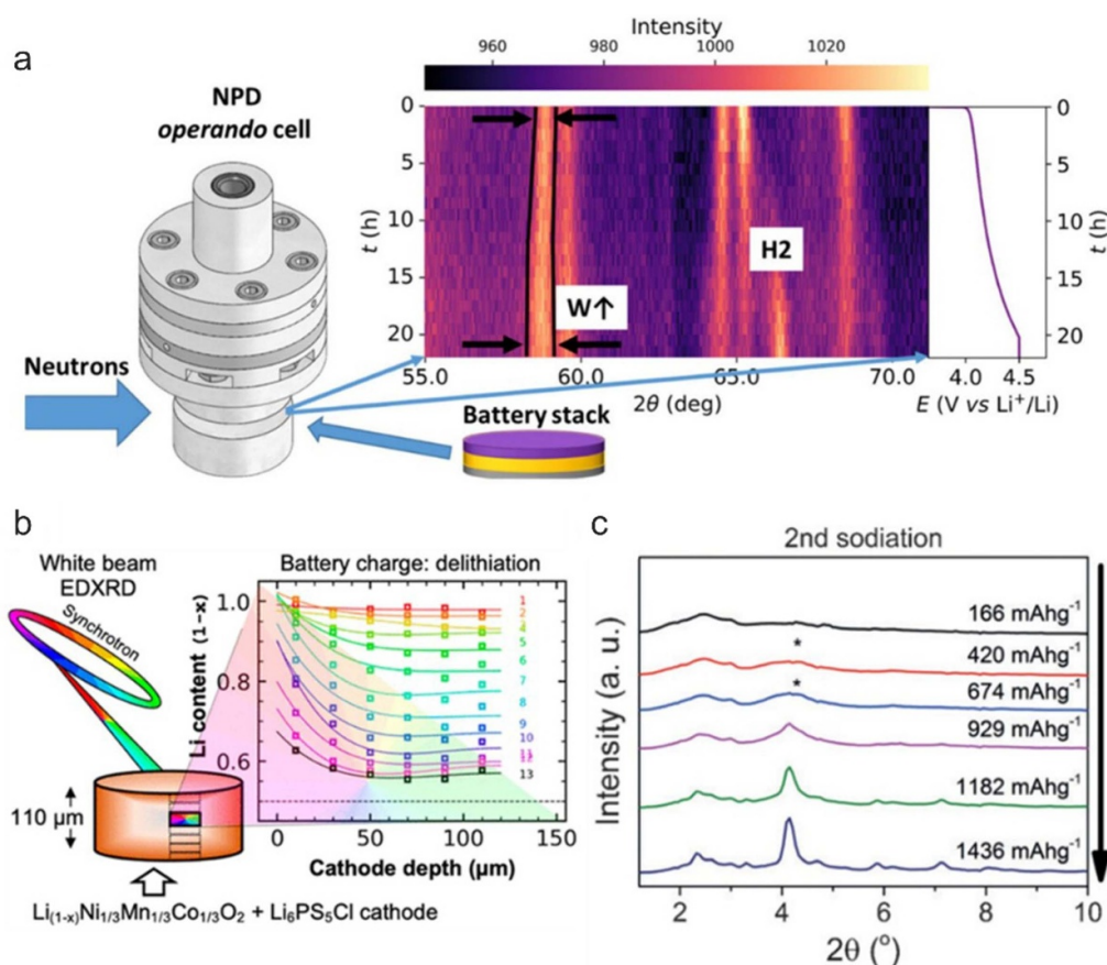
Figure 18. (a) Operando TiZr NPD during the charging of LiNi_{0.5}Mn_{0.3}Co_{0.2}O_2 (NMC532), showing the broadening of NMC532 reflections and the formation of the H_2 phase. Reprinted with permission from [340]. Copyright (2025) American Chemical Society. (b) Depth-resolved operando XRD of an LiNi_{0.33}Mn_{0.33}Co_{0.33}O_2 (NMC111) electrode at a synchrotron, revealing the development of a de-lithiation gradient. Reproduced from [345]. CC BY 4.0. (c) Reconstructed XRD-CT data from a single voxel ( 1.2 \times 1.2 \mu m^2 ) in a Na_3P electrode during operando sodiation. The asterisks denote P nanoparticles [346]. John Wiley & Sons. © 2017 Wiley-VCH Verlag GmbH & Co. KGaA, Weinheim.
