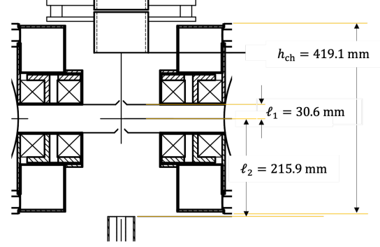
FIG. 10. Side view of the RHIC target chamber to illustrate the interaction volume (see also Fig. 2). The atomic beam enters from the top. The height of the target chamber is h_{\text{ch}} = 419.1 mm. The distance between the exit of the rf transition unit in the ABS and the RHIC beam amounts to \ell_1 = 30.6 mm. The beam is assumed to have a transverse radius of \approx 5 mm as it travels downward into the BRP.
