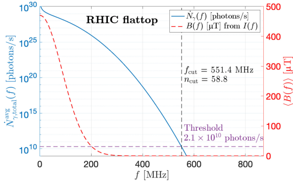
FIG. 11. Photon emission rate \dot{N}_{\gamma,\text{total}}^{\text{avg}}(f) from Eq. (39) (left axis, blue line) and corresponding rf magnetic field amplitude \langle B(f) \rangle from Eq. (37) (right axis, dashed line), derived from the analytical Gaussian RHIC bunch envelope. The dashed horizontal line marks the threshold of 2.1 \times 10^{10} photons/s required to depolarize 1% of the atoms in the beam. The vertical line marks the cutoff frequency f_{\text{cut}} = 551.4 MHz and harmonic number n_{\text{cut}} = 58.8 where the photon rate drops below the depolarization threshold.
