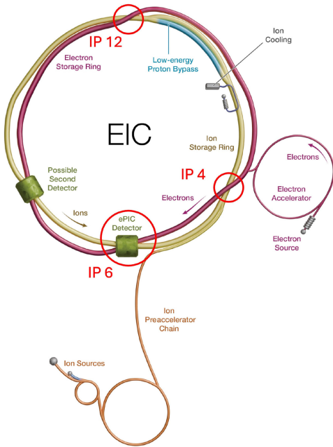
FIG. 1. Aerial view of the electron-ion collider (EIC) layout at Brookhaven National Laboratory. The primary detector, ePIC, is located at interaction point IP 6 (6 o'clock position). For the EIC, the absolute HJET polarimeter and one fast proton-carbon (pC) polarimeter will be installed at IP 4 (4 o'clock), while an additional pC polarimeter is foreseen near IP 6. During RHIC operation, the HJET and two pC polarimeters (one for each beam) were located at IP 12 (12 o'clock). (Figure reflects the project planning status as of May 2025.)
