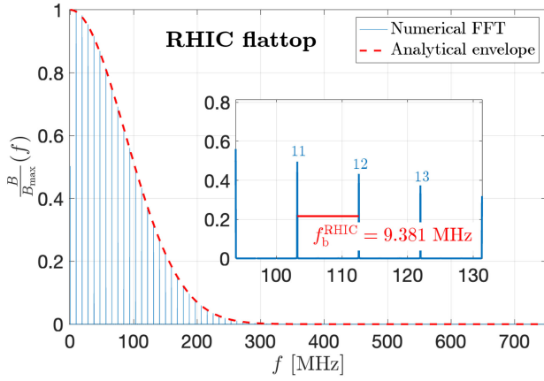
FIG. 8. Comparison of the numerically obtained one-sided normalized FFT amplitude spectrum (blue) of the rf magnetic field B(f) with the analytical envelope (dashed red) from Eq. (18) for the conditions on RHIC flattop. The frequency axis is shown in MHz. Harmonic numbers n = f/f_b are labeled near the peaks. The numerically computed bunch repetition frequency f_b^{\text{RHIC}} in the inset agrees well with the analytically calculated one from Table II.
