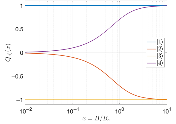
FIG. 5. Nuclear target polarization of hydrogen hyperfine states as a function of the dimensionless magnetic field parameter x = B/B_c , as given by Eq. (12). States |1\rangle and |3\rangle maintain constant nuclear polarizations of +1 and -1 , respectively, at all field strengths. The mixed states |2\rangle and |4\rangle exhibit field-dependent polarizations that evolve from 0 in the weak-field limit ( x \rightarrow 0 ) to \pm 1 in the strong-field limit ( x \rightarrow \infty ).
