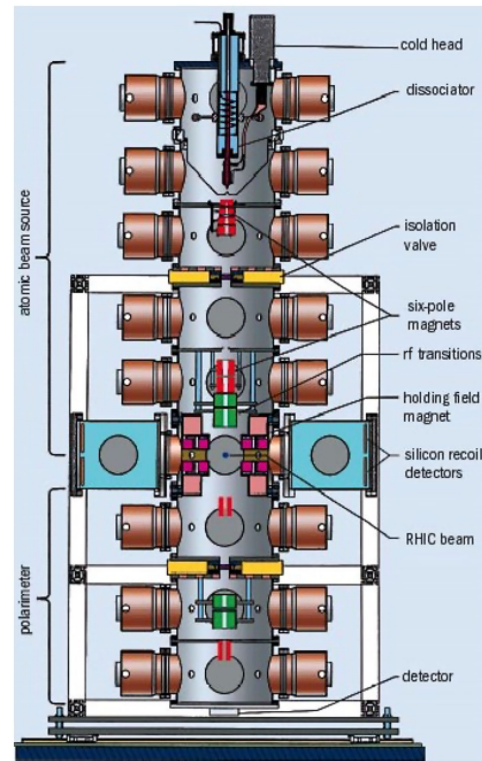
FIG. 2. Schematic layout of the HJET polarimeter, taken from Ref. [17], showing the atomic beam source, the scattering chamber, and the Breit-Rabi polarimeter. The detector geometry and coordinate system are detailed in Fig. 3.
