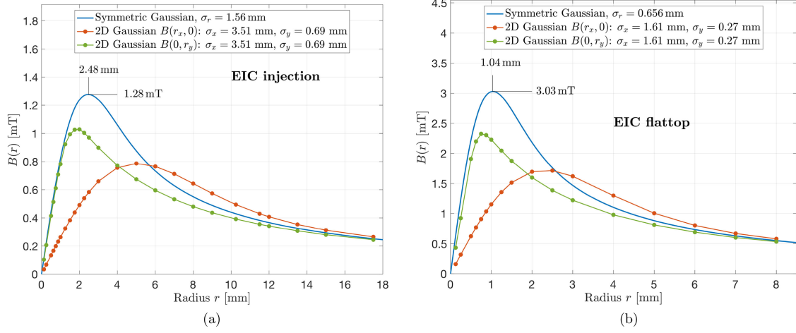
FIG. 15. Magnetic field distribution for the EIC at injection (23.5 GeV) (a) and flattop (275 GeV) (b). The blue curves show the analytical radial field profile B(r) for a symmetric Gaussian beam with rms width \sigma_r , reaching the peak fields indicated. Red and green markers show numerical calculations using the Green's function method for an asymmetric Gaussian beam with \sigma_x and \sigma_y , plotted along the horizontal and vertical axes as B(r_x, 0) and B(0, r_y) , respectively.
