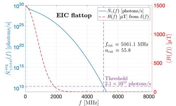
FIG. 16. Photon emission rate \dot{N}_{\gamma, \text{total}}^{\text{avg}}(f) from Eq. (39) (left axis, blue line) and corresponding rf magnetic field amplitude \langle B(f) \rangle from Eq. (37) (right axis, dashed line) for EIC flattop operation (275 GeV). The dashed horizontal line marks the threshold of 2.1 \times 10^{10} \text{ s}^{-1} required to depolarize about 1% of the atoms in the beam. The vertical line marks the cutoff frequency f_{\text{cut}} = 5061.1 MHz and harmonic number n_{\text{cut}} = 55.8 where the photon rate drops below the depolarization threshold.
