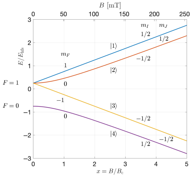
FIG. 4. Hyperfine energy levels of hydrogen |1\rangle to |4\rangle labeled with their quantum numbers F, m_F, m_I, m_J vs magnetic field, using Eq. (11) with E_{\text{hfs}} from Eq. (9) and B_c from Eq. (10). The bottom axis is in units of x = B/B_c , the top axis gives B in mT.
