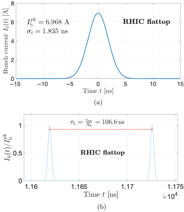
FIG. 7. Temporal current profiles of RHIC bunches on flattop at 255 GeV. Panel (a) Single Gaussian bunch current profile I_b(t) from Eq. (14) with Gaussian width t and bunch charge Q , as listed in Table II. Panel (b) Two consecutive Gaussian bunches, separated by the nominal bunch spacing \tau_b .
