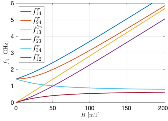
FIG. 6. Magnetic-field dependence of the transition frequencies f_{ij}(B) between the hydrogen hyperfine states, calculated using Eq. (13). The transitions are labeled as f_{ij}^\pi , f_{ij}^\sigma , or f_{ij}^{2\gamma} according to their selection rules and field orientation. All frequencies are shown in GHz as a function of the magnetic field up to 4B_c .
