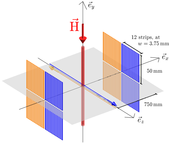
FIG. 3. Sketch of the detector setup at the HJET at RHIC. The atomic \vec{H} beam enters from above and intersects the hadron beams orthogonally. Recoil protons are detected using silicon strip detectors placed symmetrically to the left and right of the vertically separated blue and yellow beams. 8 Si strip detectors are used with 12 vertical strips, each with a pitch of w = 3.75 mm and 500 \mu\text{m} thickness. The coordinate system is indicated with \vec{e}_x \parallel to ring plane, \vec{e}_y \perp to ring plane, and \vec{e}_z along the beam momentum.
