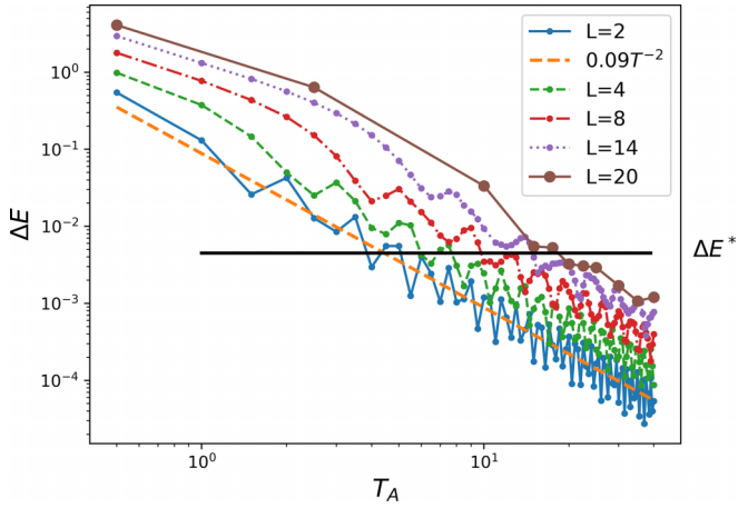
FIG. 2. \Delta E as a function of T_A for a linear annealing schedule with U/t_H = 4 .
