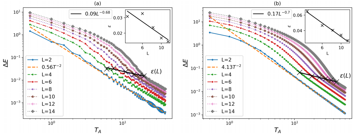
FIG. 3. \Delta E as a function of T_A for a linear annealing schedule with (a) U/t_H = 8 and (b) U/t_H = 16 . The crosses indicate onsets \epsilon(L) , which are plotted as a function of L in the inset.
