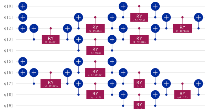
FIG. 6. Circuit that prepares the ground state of Eq. (7) for L = 5 , N_\uparrow = 3 , and N_\downarrow = 2 .
