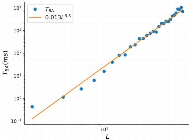
FIG. 8. The computation time T_{BA} to solve the Bethe-ansatz equations as a function of L for Hubbard Hamiltonians with 2N_\downarrow = N = L and U = 4t_H .
