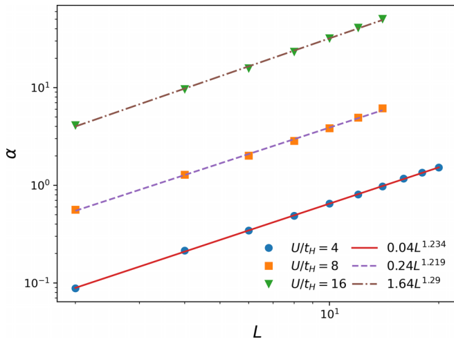
FIG. 4. \alpha(L) as a function of L for a linear annealing schedule and U/t_H = 4, 8, 16 .
