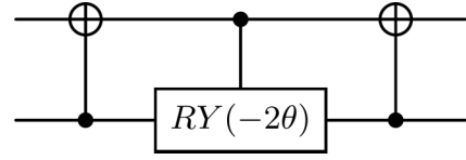
FIG. 5. Quantum circuit for implementing a Givens rotation on neighboring qubits.
