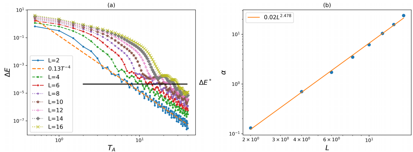
FIG. 9. (a) \Delta E as a function of T_A and (b) \alpha(L) as a function of L for a sinusoidal annealing schedule with U/t_H = 4 .
