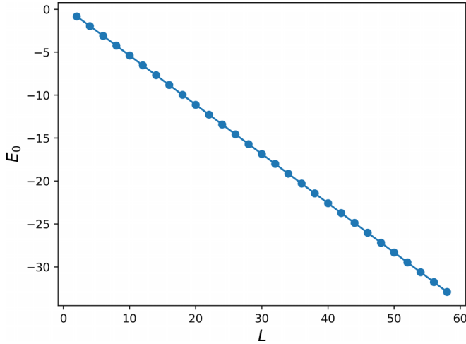
FIG. 7. E_0 as a function of L for Hubbard Hamiltonians with 2N_\downarrow = N = L and U = 4t_H .
