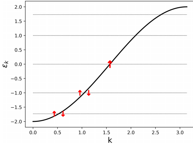
FIG. 1. Dispersion relation and the ground-state occupation of the energy levels of the initial Hamiltonian for L = 5 , N_{\uparrow} = 3 , and N_{\downarrow} = 2 .
