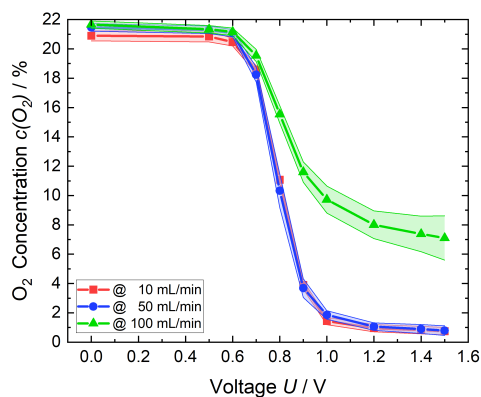
Fig. 5.17. Remaining O_2 content (line) and the resulting error (colored area) of each air flow rate.
