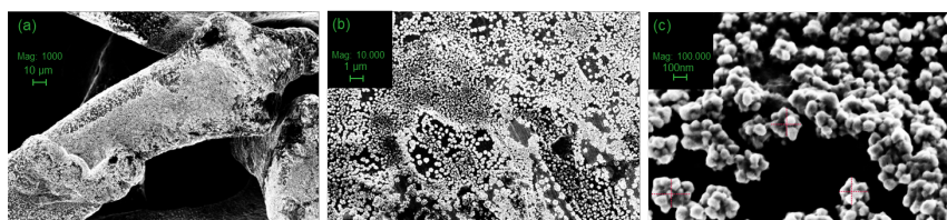
Fig. 6.3. SEM images of the Au particles. (a) Magnification of 1000, (b) magnification of 10.000 and (c) magnification of 100.000.
