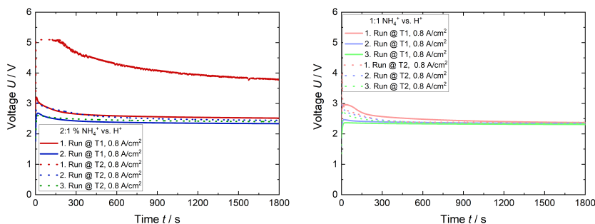
(a) Ratio of 2:1 \text{NH}_4^+ vs. \text{H}^+ .
