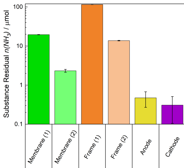
Fig. 7.15. Detected amount of \text{NH}_3 in the cell components, a logarithmic scale is chosen to show small amounts present in some components. The frame area of the membrane and the active area of the membrane were re-inserted into a fresh solution, because not all of the \text{NH}_4^+ -ions within these areas were expelled in the first solution.
