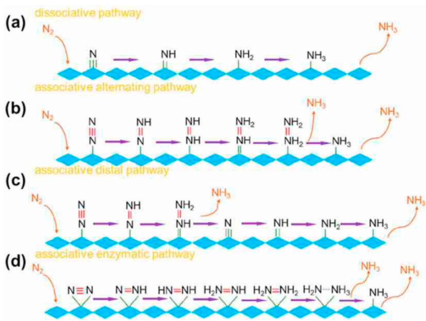
Fig. 2.1. The different reaction mechanisms on heterogeneous catalysts of the NH_3 synthesis. (a) Dissociative mechanism, where the triple bond of nitrogen is broken before hydrogenation. (b) Alternating mechanism, the N atoms of N_2 are alternately hydrogenated. (c) Distal pathway, the N atom removed from the adsorption site is first sequentially hydrogenated. (d) Enzymatic pathway, the adsorption of N_2 onto the surface of the catalyst results in a side-on mode instead of the end-on mode. Adapted with permission from [79], American Chemical Society.
