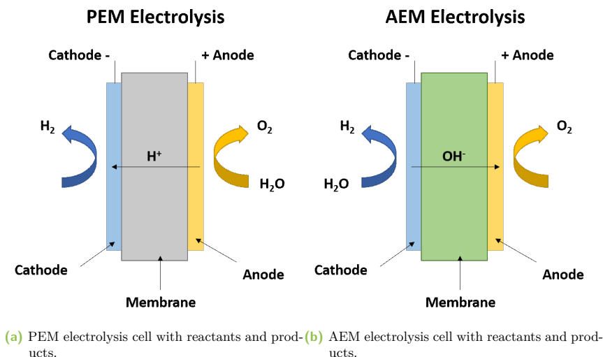
Fig. 5.1. Water electrolysis cells in acid and alkaline environment [149].
