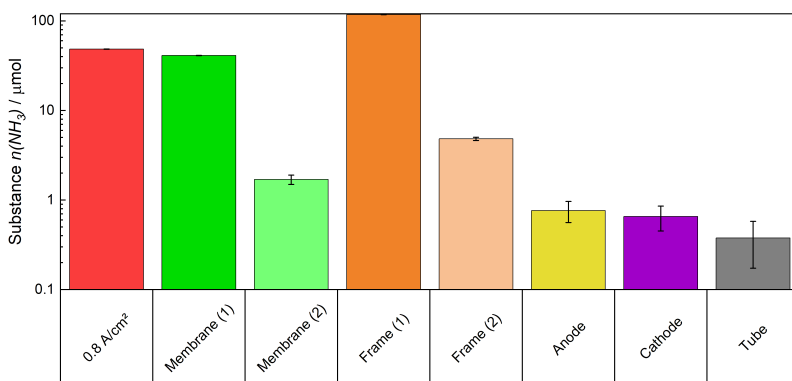
Fig. 7.16. \text{NH}_3 expelled electrochemically (red) and the detected amounts of \text{NH}_3 expelled from the cell components. A logarithmic scale is chosen to show small amounts present in some components. The frame area of the membrane and the active area of the membrane were re-inserted into a fresh solution, because not all of the \text{NH}_4^+ -ions within these areas were expelled in the first solution.
