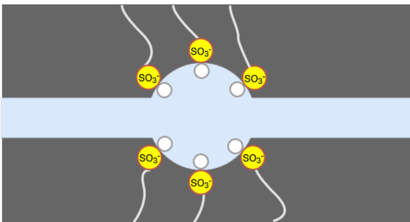
Fig. 1.9. Schematic illustration of the microstructure of Nafion. The sulphit ions ( \text{SO}_4^{2-} ) are bound to [\text{CF}_2]_n , resulting in \text{SO}_3^- . \text{SO}_3^- is firmly bound within the membrane. The protons (white circles) are mobile and can be exchanged with other cations within the membrane.
