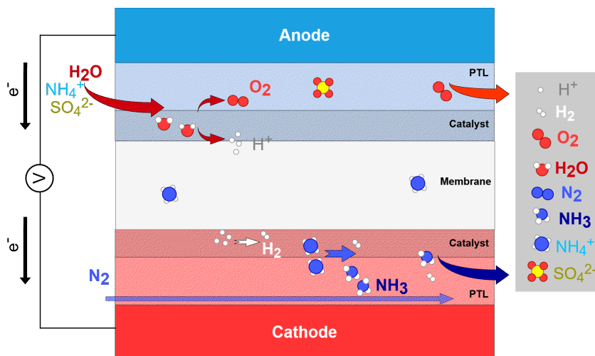
Fig. 8.1. Schematic illustration of the \text{NH}_3 recycling process through the membrane. \text{H}_2\text{O} , which contains dissolved \text{NH}_4^+ and \text{SO}_4^{2-} is introduced into the PTL of the anode. The \text{NH}_4^+ -ions can diffuse through the membrane, because Nafion is cation conductive. The \text{SO}_4^{2-} can not diffuse through the membrane, the remain on the anode side. In the catalyst layer \text{H}_2\text{O} is oxidized to \text{O}_2 and \text{H}^+ . The produced \text{O}_2 exits the cell at the anode outlet. The generated \text{H}^+ either remain on the anode side, diffuses through the membrane and is reduced to \text{H}_2 or it interacts with the \text{NH}_4^+ -ions, which were introduced into the membrane, within the membrane. The diffused \text{NH}_4^+ -ions deprotonate at the cathode. \text{NH}_3 is produced and the resulting \text{H}^+ are reduced to \text{H}_2 with the supplied e^- from the cathode. \text{N}_2 is used as carrier gas to remove \text{NH}_3 and \text{H}_2 from the cell. The coloring of the atoms is done according to the CPK color model.
