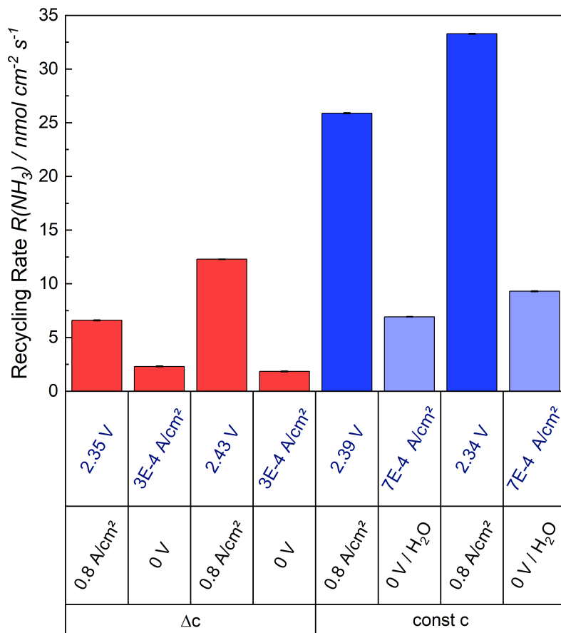
Fig. 8.8. Resulting recycling rates while the (\text{NH}_4)_2\text{SO}_4 solution was recirculated (red), leads to \Delta c and while the solution was not recirculated (blue), c was constant. In black the applied potentials and current density are written and in dark blue the corresponding measured values.
