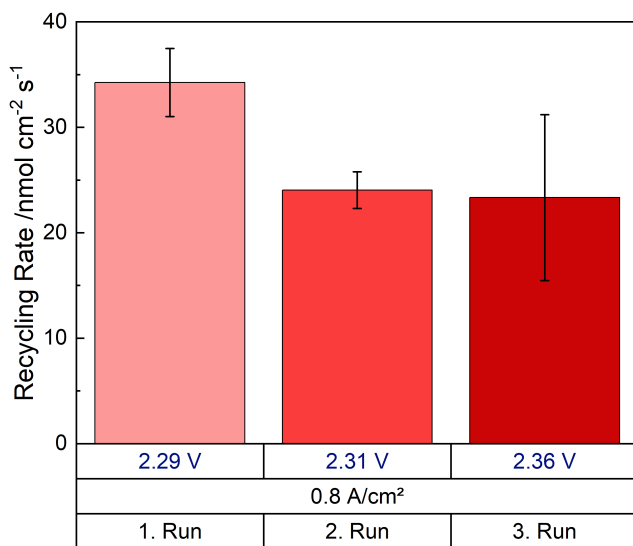
Fig. 8.11. The average \text{NH}_3 recycling rates with the respective error bars of for the three runs of the studied cells are shown in different shades of red. In black the applied current density is written and in dark blue the corresponding measured potentials.
