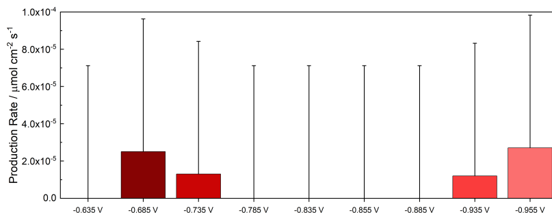
Fig. 6.14. Calculated production rates of \text{NH}_3 production and the corresponding error bars that are determined while \text{N}_2 was supplied at the specific conditions in the H-cell.
