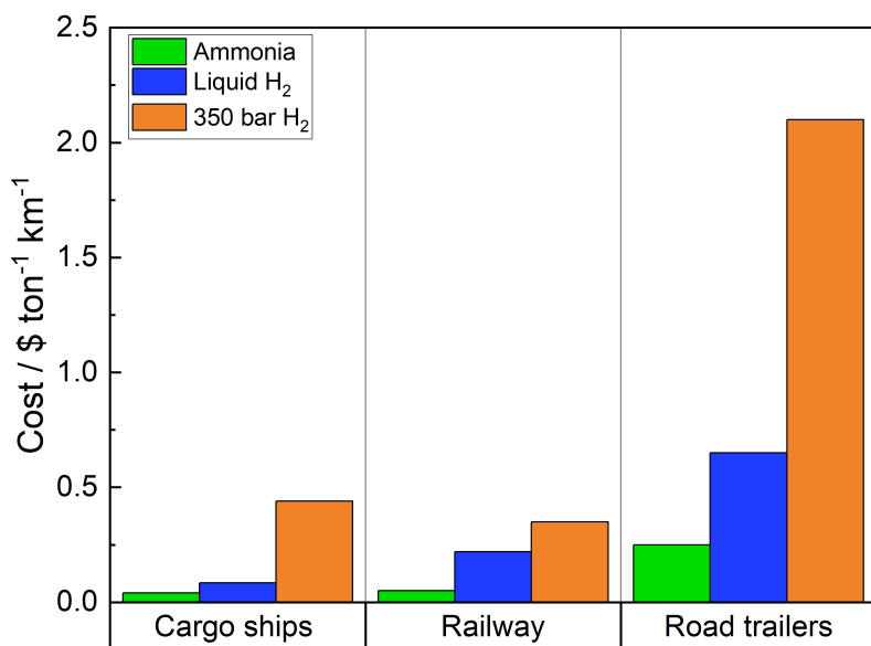
Fig. 1.3. Transportation cost of the energy carriers NH 3 , liquid H 2 , and compressed H 2 for a distance of 1 km and a weight of 1 t. The different transportation possibilities cargo ships, railway, road trailers are compared. Adapted and based on [18]. Found in [17].
