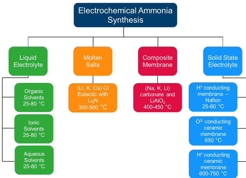
Fig. 1.6. Different electrochemical \text{NH}_3 synthesis systems with respect to different electrolytes and temperature ranges. Adapted with permission from [40], Elsevier.
