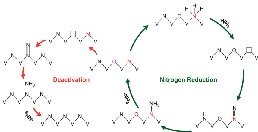
Fig. 2.2. Illustration of the activation and deactivation of the catalytic reaction pathway for the NRR via Mars-van Krevelen mechanism. Adapted with permission from [58], American Chemical Society.
