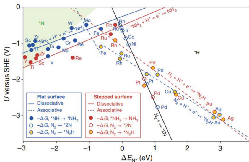
Fig. 2.4. Volcano diagrams evaluating the onset potential ( U ) on metal surfaces for the reduction of N_2 . The solid lines illustrates the dissociative mechanisms, and the dashed lines the associative. A catalyst reaction on a flat surface area is indicated in blue and a stepped surface area in red. An overlap of the red and blue lines is indicated by the black line. The surfaces of catalysts, which are likely covered by adsorbed nitrogen are in the green shaded area and the ones covered by hydrogen are in the white area [67, 76]. Adapted with permission from [76], John Wiley and Sons.
