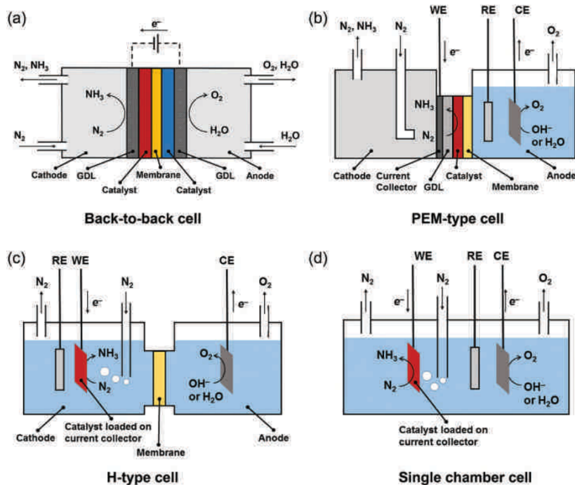
Fig. 2.6. Schematic illustration of the different reactor configuration for electrochemical NRR, (a) back-to-back cell, (b) PEM-type cell, (c) H-type cell, and (d) single chamber cell. Adapted with permission from [78], John Wiley and Sons.
