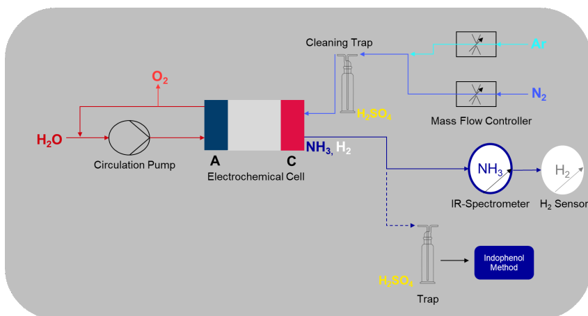
Fig. 3.2. Illustration of the test bench utilizing H 2 O as reactant. H 2 O is introduced on the anode side via a circulation pump. Due to the supply of H 2 O humidifier cells are not required. At the anode O 2 is as well produced. On the cathode side either N 2 or Ar are supplied via mass flow controllers. The gas streams through a cleaning trap before entering the cell. The synthesized NH 3 is determined with the indophenol method or with an IR-spectrometer. H 2 is determined with a hydrogen sensor.
