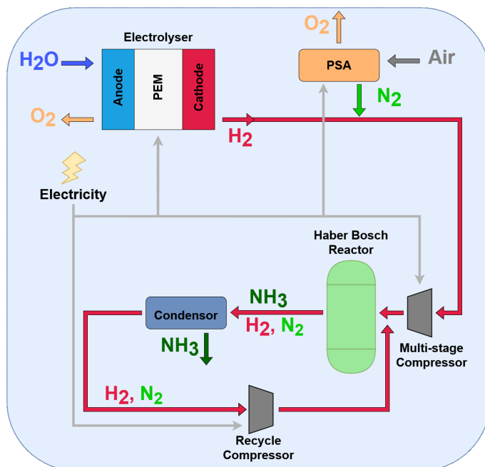
Fig. 4.4. Schematic illustration of the electrified Haber-Bosch process. A water electrolyzer is utilized to produce \text{H}_2 from \text{H}_2\text{O} . The further part of the process is the same as the process of the Haber-Bosch process. Own illustration based on the illustration of [144].
