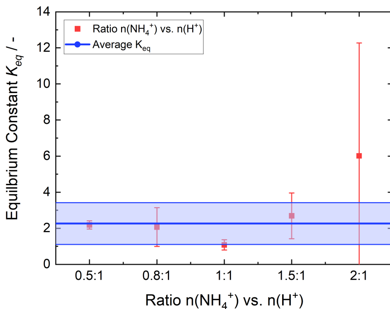
Fig. 7.3. Equilibrium constants of the different ratios of NH_4^+ vs. H^+ (red squares) and their corresponding error bars. The average value of K_{eq} is shown as the blue line. The colored area is the error of the average value. The value of the ratio 2:1 is not considered for the average value.
