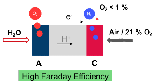
Fig. 5.19. Parameters that lead to a relative O_2 depletion and N_2 enrichment on the cathode side are marked in green, those that have no influence on the O_2 content are marked in yellow and the parameter that leads to a relative increase in the O_2 content on the cathode side is marked in red in the table. The illustration of the cell shows, that the O_2 content of an air gas stream can be reduced to less than 1 % of remaining O_2 , while achieving a high FE close to 100 %.
