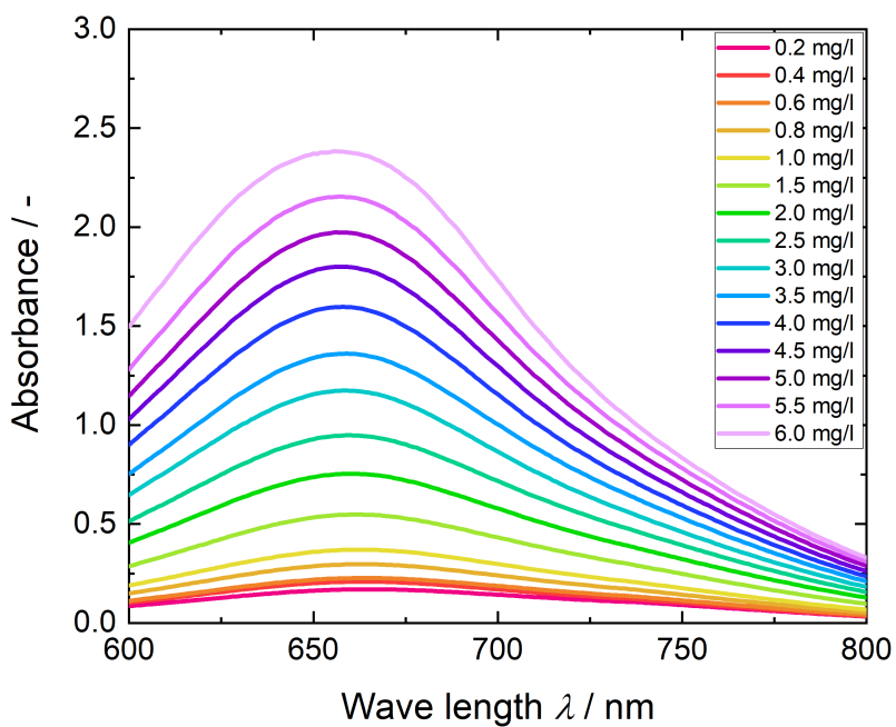
Fig. 3.6. Indophenol blue absorbance spectrum of the calibration samples from 0.2 to 6 mg L -1 .
