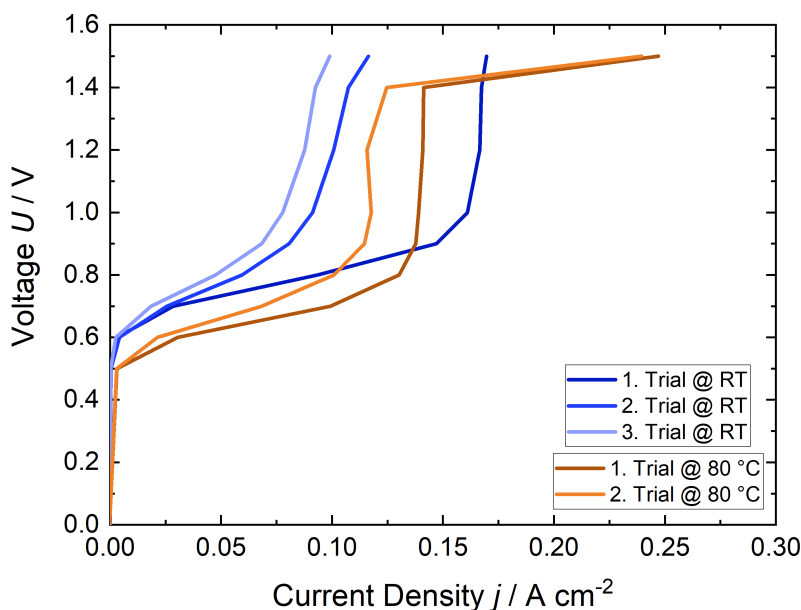
Fig. 5.11. Polarisation curves showing the effect of temperature increase and the resulting influence of degradation while applying an air flow rate of 50 mL/min at RT (blue lines) and 80 °C (orange lines).
