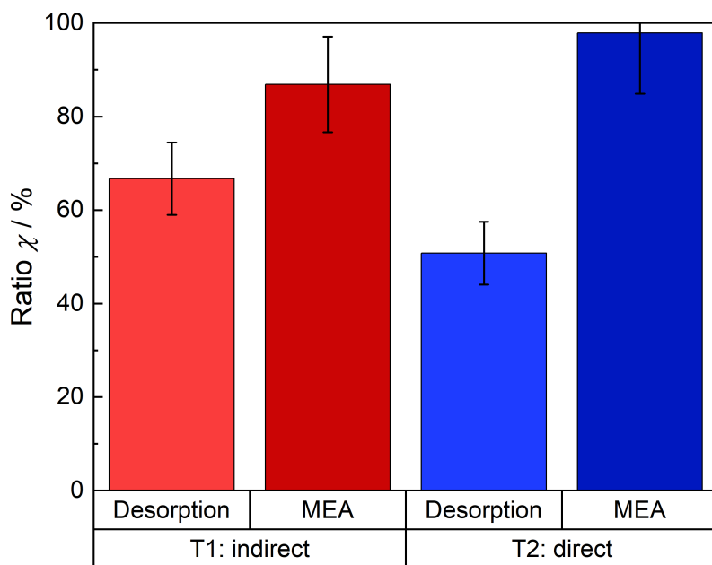
Fig. 7.17. \text{NH}_3 expelled electrochemical (red and blue bar) and the total amount of \text{NH}_3 that was found, electrochemical plus the quantity which were expelled afterwards in the \text{H}_2\text{SO}_4 solutions from the cell components (dark red and blue).
