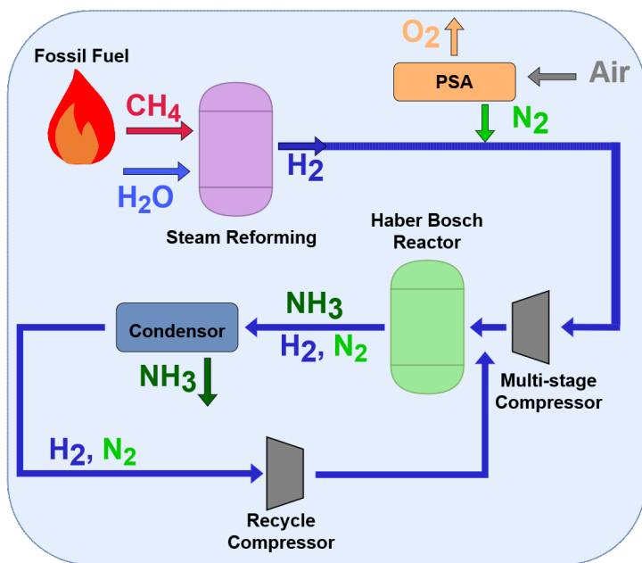
Fig. 4.1. Simplified illustration of the Haber-Bosch process. Fossil fuels and water are used to generate \text{H}_2 in the steam reformer. \text{N}_2 from air is enriched with PSA. The reactants, \text{H}_2 and \text{N}_2 are then introduced into the Haber-Bosch reactor. \text{NH}_3 is synthesized in the Haber-Bosch reactor. \text{NH}_3 is condensed and the reactant gases that do not react are fed back into the reactor. Own illustration based on the illustration of [144].
