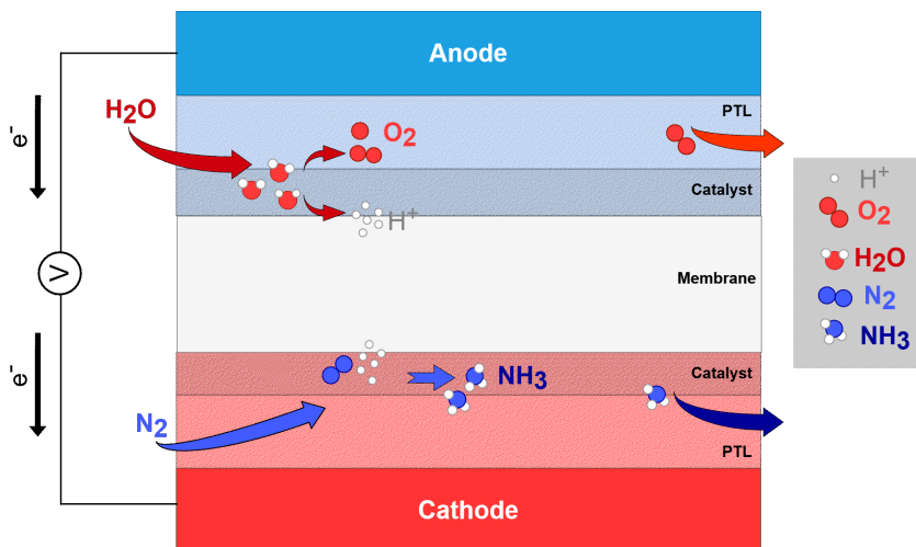
Fig. 6.2. Schematic illustration of the direct electrochemical \text{NH}_3 synthesis and the movement of molecules and ions in an acid and neutral cell. \text{H}_2\text{O} is introduced into the GDL of the anode. In the catalyst layer it oxidizes to \text{O}_2 and \text{H}^+ . The produced \text{O}_2 exits the cell on the anode side and the \text{H}^+ diffuses through the membrane. \text{N}_2 is reduced at cathode and reacts with the incoming \text{H}^+ to \text{NH}_3 in the catalyst layer. This process is facilitated by the electrical energy. The resulting \text{NH}_3 exits the cell on the cathode side. The coloring of the atoms is done according to the CPK color model.
