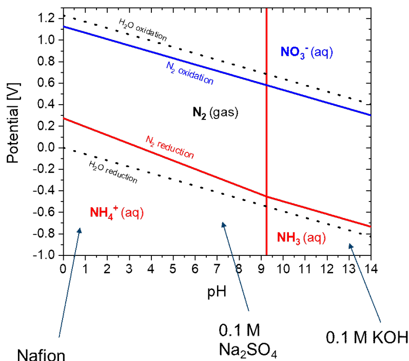
Fig. 4.6. Pourbaix diagram for N 2 and H 2 O. The red solid line represents the NRR to NH 4 + or NH 3 . The blue solid line represents the N 2 oxidation to NO 3 - . The black dotted lines denote the H 2 O reduction and oxidation.
