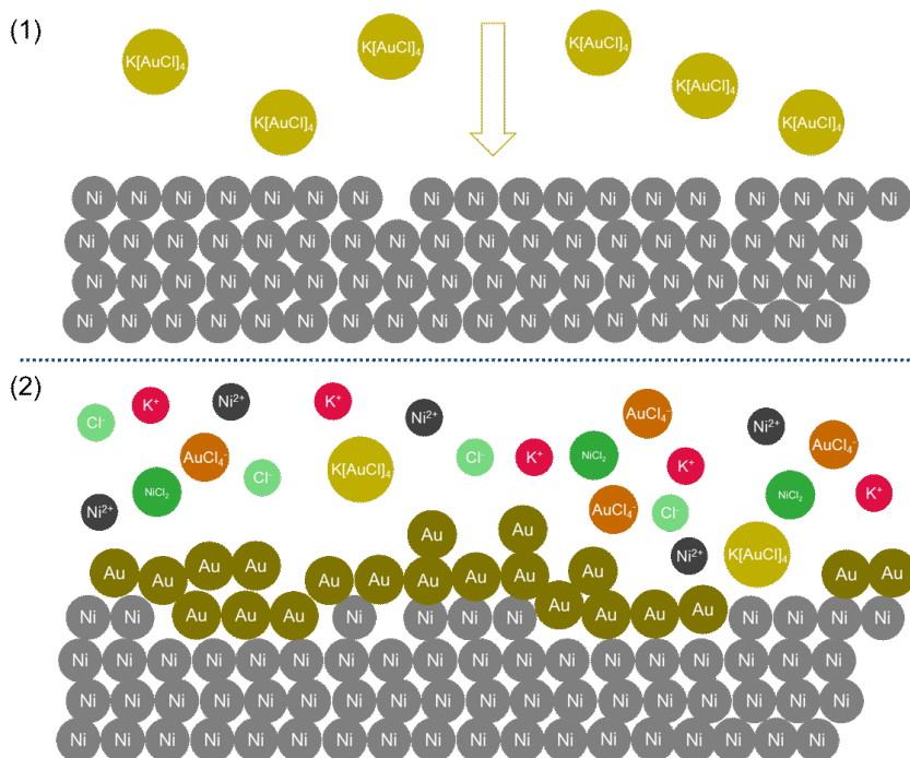
Fig. 3.9. Schematic illustration of the spontaneous galvanic displacement deposition process. Nickel is displaced with gold particles.
