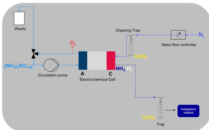
Fig. 8.2. Schematic illustration of the test setup.
