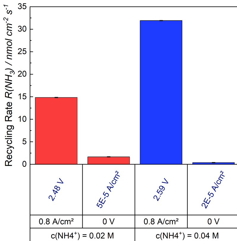
Fig. 8.4. Recycling rates of the \text{NH}_4^+ concentration of 0.02 M (red) and 0.04 M (blue) in the (\text{NH}_4)_2\text{SO}_4 solution. In black the applied potentials and current density are written and in dark blue the corresponding measured values.
