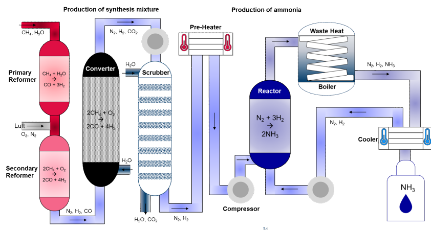
Fig. 1.4. Illustration of the process steps of the Haber-Bosch process, the industrial synthetic \text{NH}_3 production. Starting with the production of the synthesis mixture until the production of \text{NH}_3 in the blue reactor.
