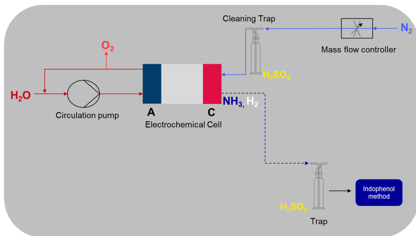
Fig. 7.6. Schematic illustration of the test bench. \text{H}_2\text{O} is supplied and \text{O}_2 is produced at the anode. \text{NH}_3 is expelled from the membrane and \text{H}_2 is produced at the cathode.
