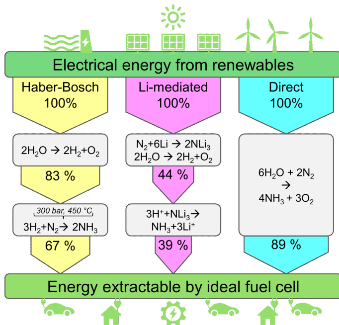
Fig. 4.7. Graphical illustration of the energy losses that occur during the electrochemical conversion of electrical energy into \text{NH}_3 and the thermodynamic efficiency of the three \text{NH}_3 synthesis pathways.
