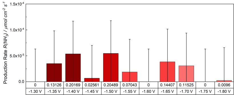
Fig. 6.17. Calculated rates of \text{NH}_3 production and the corresponding error bars that were determined while \text{N}_2 was supplied at the specific conditions.
