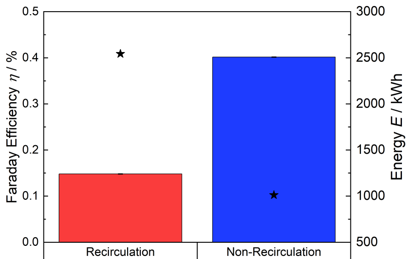
Fig. 8.10. FE of NH_3 regarding recirculation (red) and non-recirculation (blue) (left y-axis). The energy consumption for recycling 1 kg are shown as black stars (right y-axis).
