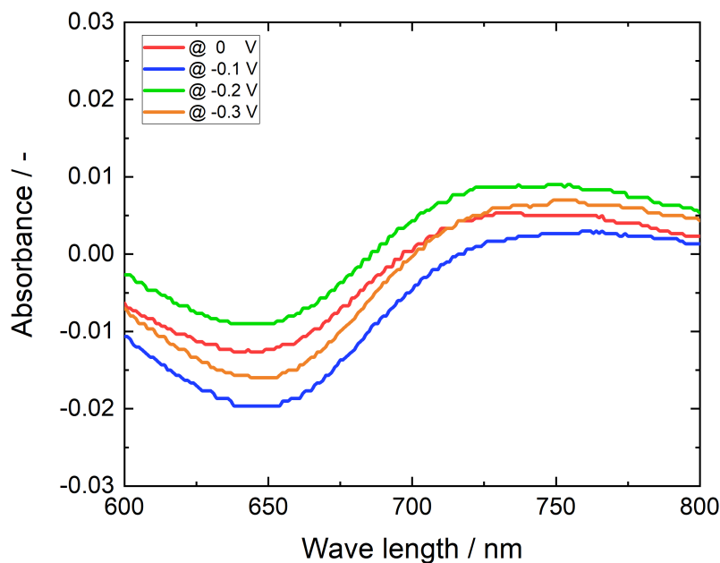
Fig. 6.6. Absorbance spectra of the VIS spectrometer for the different applied potentials while introducing H_2 at the anode.
