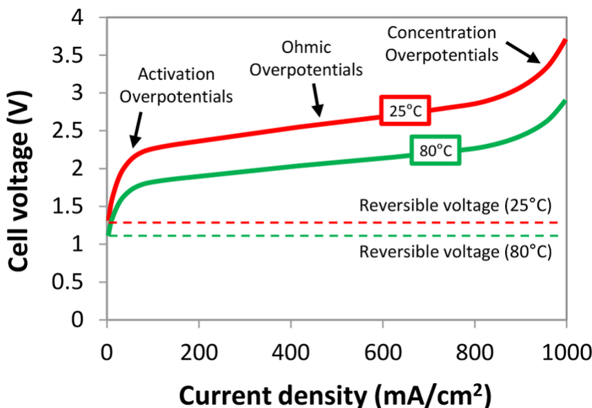
Fig. 3.10. Polarisation curves of H 2 O electrolysis at 25 (red line) and 80 °C (green line). The resulting overpotentials activation, ohmic, and concentration are marked. The reversible cell potential of both temperatures are drawn as dashed lines with the respective color [130].
