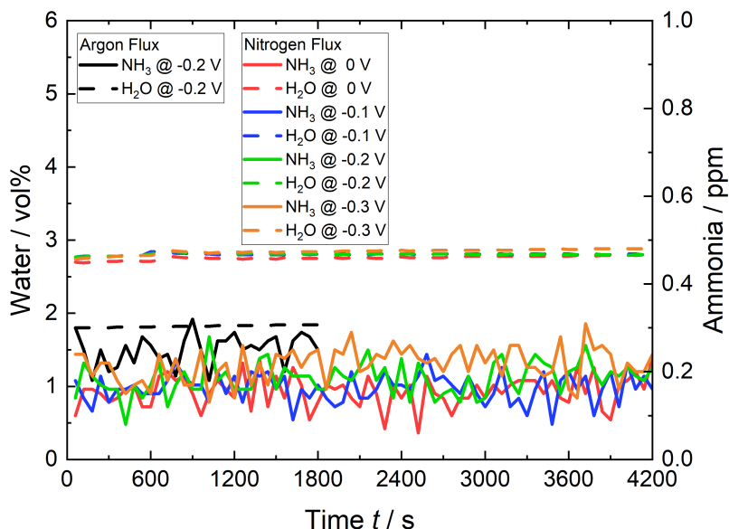
Fig. 6.5. Detected \text{NH}_3 (solid lines) and \text{H}_2\text{O} (dashed lines) in their corresponding concentration with the FTIR spectrometer. The black lines are measured during the Ar supply and the colored ones during \text{N}_2 supply.
