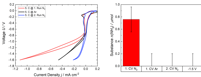
(a) Last CV cycles of the trials.
