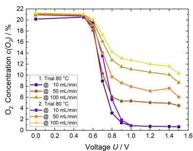
(b) O_2 depletion at 80 °C.
