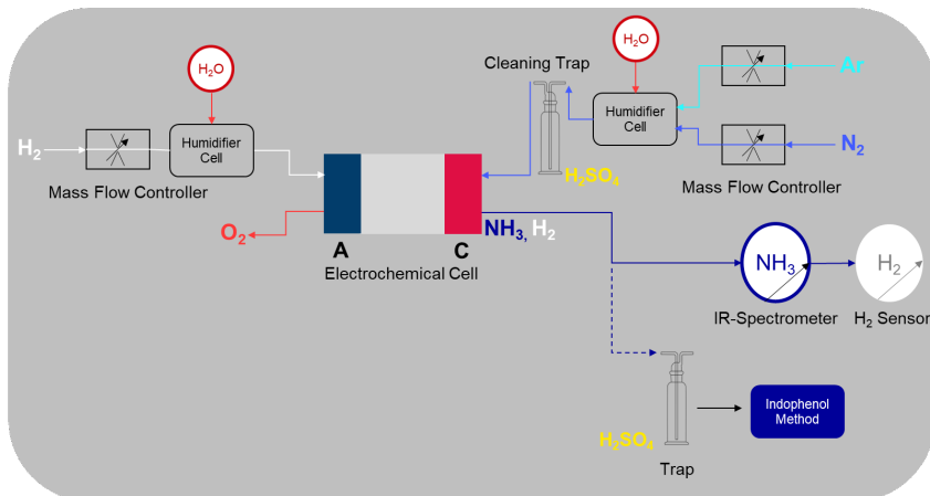
Fig. 3.1. Illustration of the test bench utilizing H_2 as reactant. H_2 is supplied via a mass flow controller on the anode side. The gas is humidified with a humidifier cell. Due to the chemical reaction O_2 is produced at the anode. On the cathode side either N_2 or Ar are supplied via mass flow controllers. The gases are also humidified. The humidification is needed for the membrane. The gas streams through a cleaning trap before entering the cell. The synthesized NH_3 is determined with the indophenol method or with an IR-spectrometer. H_2 is determined with a hydrogen sensor.
