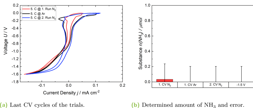
Fig. 6.8. (a) CV results of the experiments. In red and blue the results during N_2 supply and in black during Ar supply. (b) The corresponding detected NH_3 and the error bars of the second MEA cell employing KOH as electrolyte.
