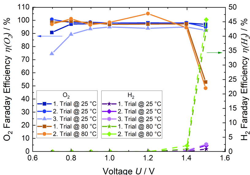
Fig. 5.12. FE of O_2 depletion (solid line) and H_2 evolution (dashed line) for all measurements while applying an air flow rate of 50 mL/min.
