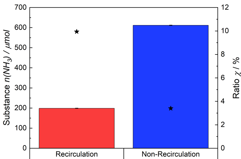
Fig. 8.9. Totalled recycled quantity of \text{NH}_3 of recirculation (red) and non-recirculation (blue) (left y-axis). The ratios of recycled quantity to the initial amount of \text{NH}_4^+ are shown as black stars (right y-axis).
