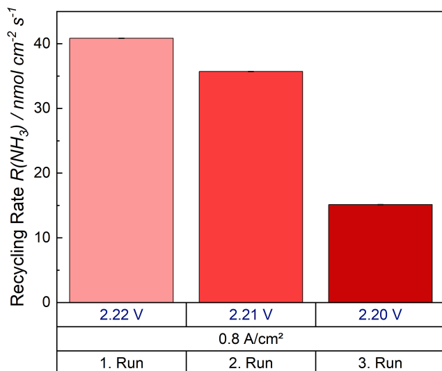
Fig. 8.14. Recycling rates of three runs of an MEA cell, while a \text{NH}_4\text{NO}_3 solution was introduced and recirculated on the anode. In black the applied current density is written and in dark blue the corresponding measured potentials.
