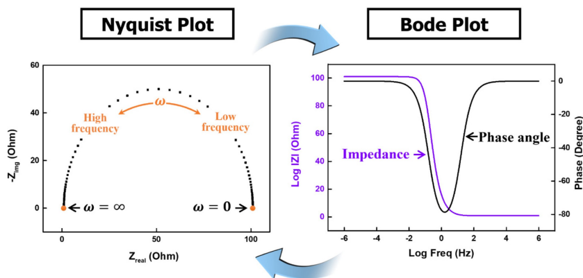
Fig. 3.12. The Nquist plot is shown on the left side and the Bode plot on the right side. They can be converted into each other [142].
