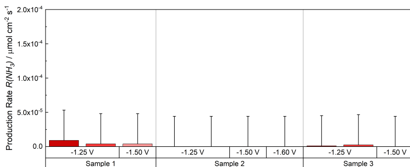
Fig. 6.10. Calculated rates of NH_3 production and the corresponding error bars that are determined while N_2 was supplied at the specific conditions.
