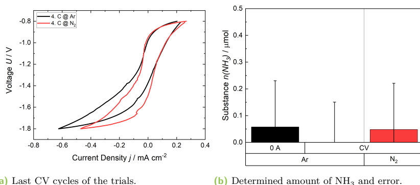
Fig. 6.18. CV results and the corresponding detected NH 3 employing Na 2 SO 4 as electrolyte. In red the results during N 2 supply and in black and grey during Ar supply.
