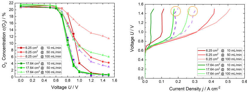
(a) O_2 depletion of active cell areas of 6.25 \text{ cm}^2 (b) Current density of active cell areas of 6.25 \text{ cm}^2 and 17.64 \text{ cm}^2 .
