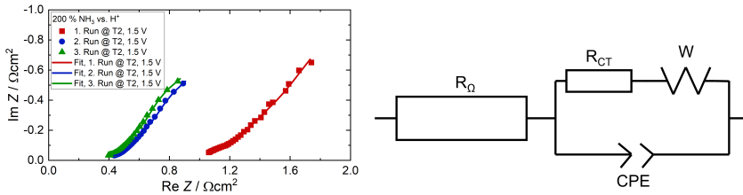
(a) EIS and fits
