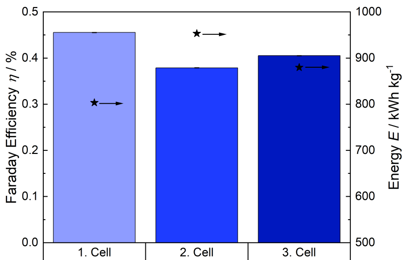
Fig. 8.13. The Faraday efficiencies of NH_3 recycling of the three cells are shown in the three shades of blue (left y-axis). The energy consumption for recycling 1 kg of NH_3 by the respective cells is shown as black stars (right y-axis).
