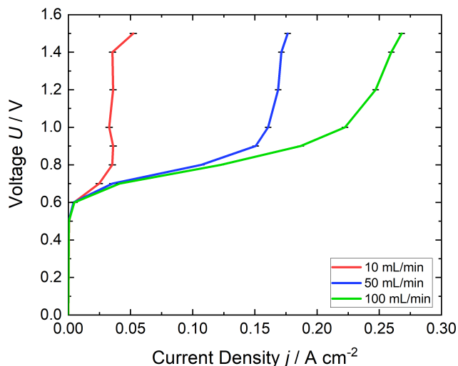
Fig. 5.13. Polarisation curves of the MEA at different air flow rates.
