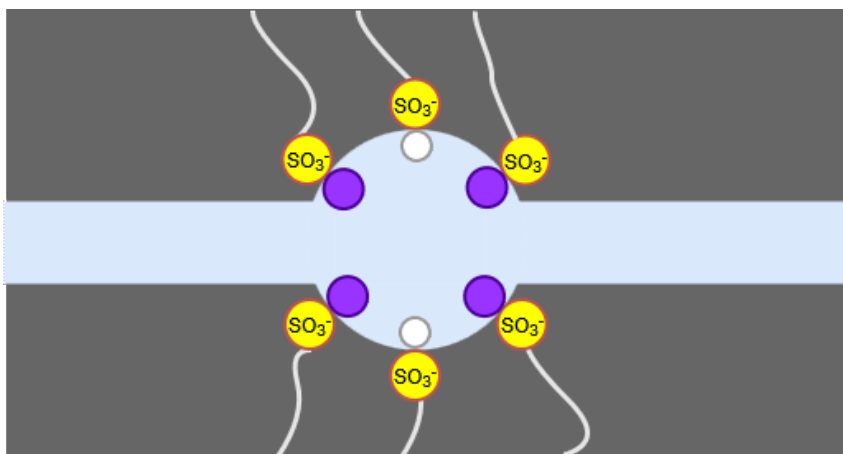
Fig. 6.4. Illustration of the ion exchanged Nafion membrane. The \text{H}^+ , which are bounded to \text{SO}_3^- are exchanged with \text{Na}^+ during the immersion of the Nafion membrane into a \text{NaOH} solution. Nafio is transferred into its \text{Na}^+ -form.
