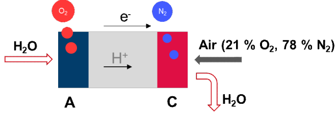
Fig. 5.3. Illustration of the oxygen depletion cell with the incoming \text{H}_2\text{O} and air. Resulting in \text{O}_2 production on anode side and \text{N}_2 accumulation and \text{O}_2 depletion on cathode side.
