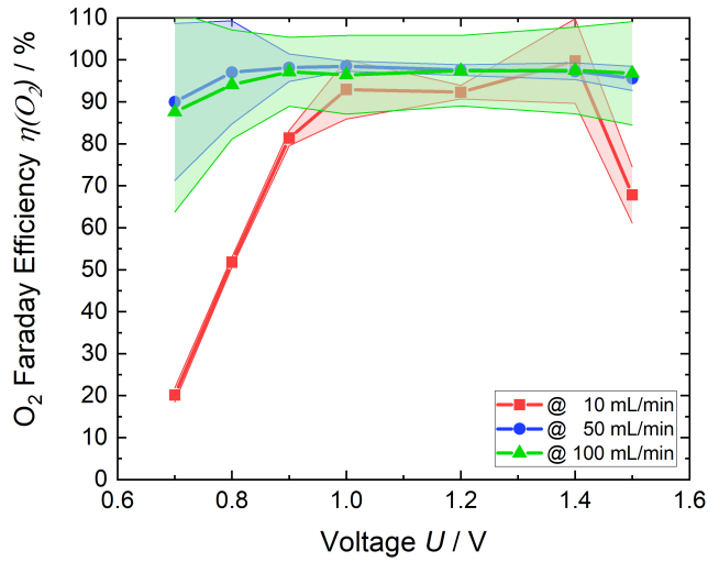
Fig. 5.18. Faraday efficiency of O 2 (lines with dots) and respective error (colored area) of each air flow rate.
