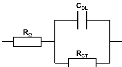
Fig. 3.11. Randle circuit for describing electrochemical systems. The randle cell consist of an ohmic resistance ( R_{\Omega} ), which is in serial connection with a capacitor, which is connected in parallel with a resistor. The capacitor ( C_{DL} ) describes the electrochemical double layer and the resistance ( R_{CT} ) the charge transfer resistance.
