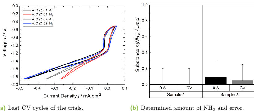
Fig. 6.12. CV results and the corresponding detected NH 3 of the trials employing Na 2 SO 4 as electrolyte. In red and blue the results during N 2 supply and in black and grey during Ar supply.
