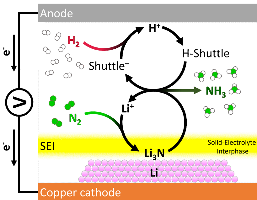
Fig. 1.7. Illustration of the necessary steps of the Li mediated eNRR. \text{Li}^+ are dissociated in the electrolyte. Under an electrical potential Li is deposited. Li dissociates \text{N}_2 to produce \text{Li}_3\text{N} . Under supply of a \text{H}^+ -source and e^- -transport \text{NH}_3 is formed. Own illustration based on the illustration of [47].
