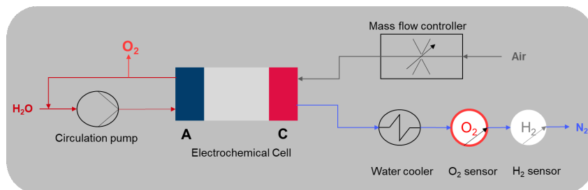
Fig. 5.5. Illustration of the \text{O}_2 depletion test set-up. \text{H}_2\text{O} is introduced with a circulation pump on the anode side. Due to the applied electrical potential \text{O}_2 is produced and \text{H}^+ are generated. At the cathode the \text{H}^+ reacts with the incoming \text{O}_2 from air to \text{H}_2\text{O} . The produced \text{H}_2\text{O} is condensed with a water cooler and the remaining \text{O}_2 in the gas stream is measured with the \text{O}_2 sensor. Additionally, if \text{H}_2 is generated, it can be determined with the \text{H}_2 sensor.
