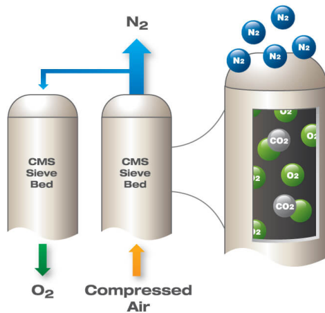
Fig. 5.2. Illustration of the pressure swing adsorption method, which is based on physical adsorption. The carbon molecular sieves adsorb O_2 at high pressure, leading to the separation of O_2 and N_2 . At the same time, in the other tower vessel the previous captured O_2 desorbs by reducing the pressure to ambient pressure. The figure is taken from [167].
