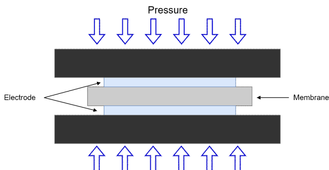
Fig. 5.6. Sketch of the hot pressing process. An applied pressure presses the catalyst layer onto the membrane, leading to a reduction of ohmic resistance, thus better ion conductivity.
