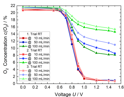
(a) O_2 depletion at room temperature.
