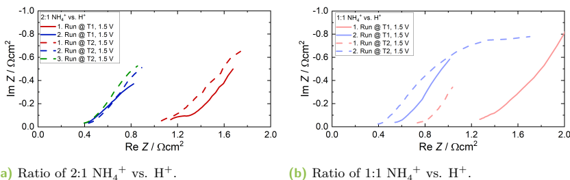
Fig. 7.12. Recorded impedance spectra at 1.5 V and RT. The spectra of the first trials are depicted as the solid lines and the second trials as dashed lines. The spectra of the first runs are shown in red, that for the second run in blue and that for the third run in green.
