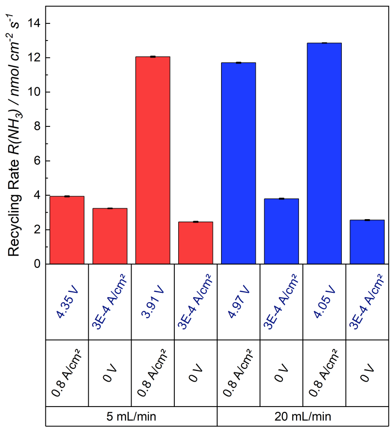
Fig. 8.5. Recycling rates of the applied solution flow rates 5 mL/min (red) and 20 mL/min (blue) in the (\text{NH}_4)_2\text{SO}_4 solution. In black the applied potentials and current density are written and in dark blue the corresponding measured values.
