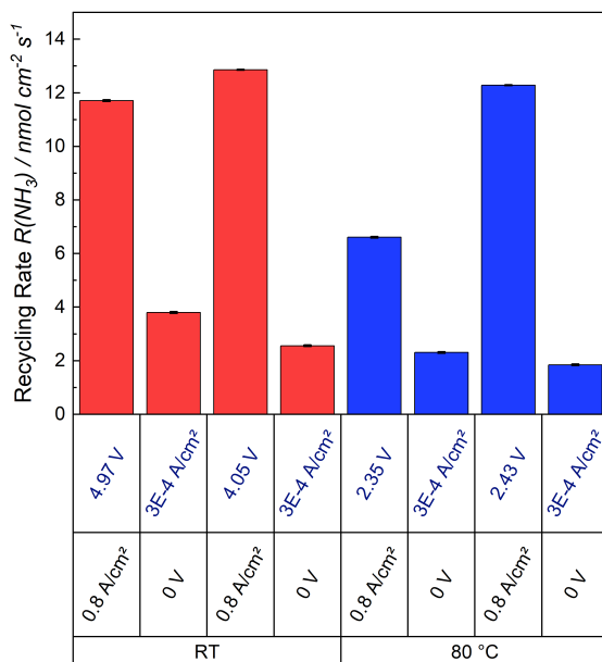
Fig. 8.6. Recycling rates at RT (red) and 80 °C (blue). In black the applied potentials and current density are written and in dark blue the corresponding measured values.
