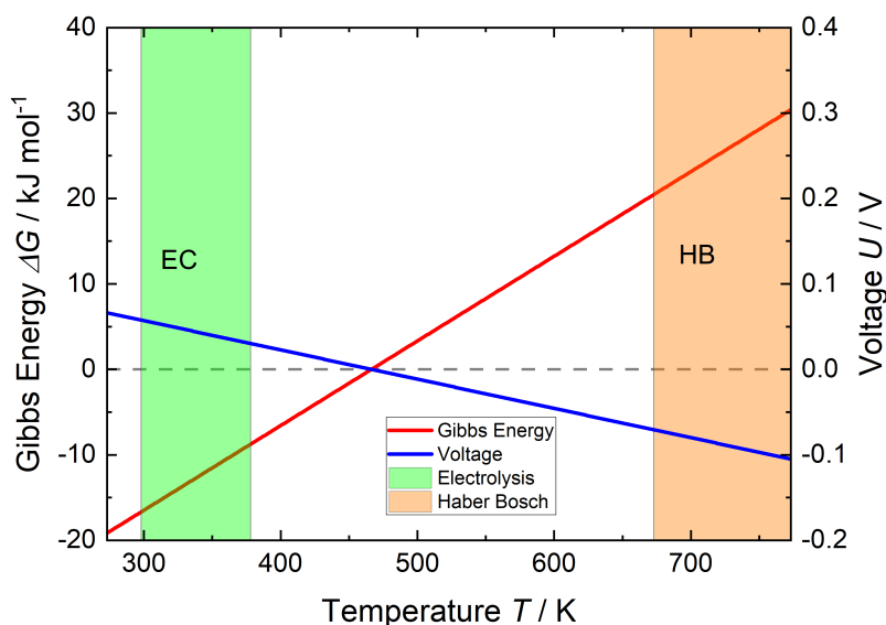
Fig. 4.2. Gibbs energy (red line, left y-axis) and voltage (blue line, right y-axis) considering constant enthalpy and entropy in dependency of temperature. The temperature ranges in which the electrochemical \text{NH}_3 synthesis (green area) and the Haber-Bosch process (orange area) operate are highlighted. The dashed grey line indicates the change from an exothermic to an endothermic process.
