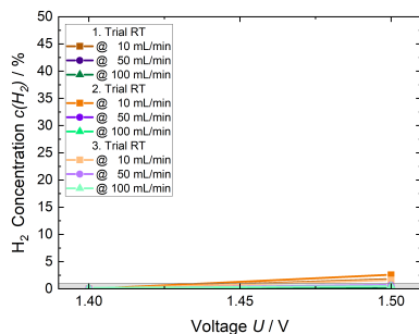
(c) H_2 evolution at room temperature.
