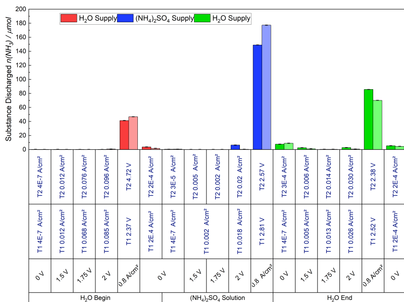
Fig. 8.3. Discharge of \text{NH}_3 during the supply of \text{H}_2\text{O} (red and green bars) and (\text{NH}_4)_2\text{SO}_4 solution (blue bars). Two trials were carried out, ensuring reproducibility. In black the applied potentials and current density are written and in dark blue the corresponding measured values.
