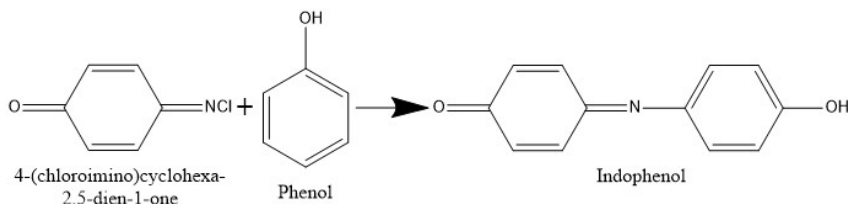
Fig. 3.5. The reaction to indophenol blue.
