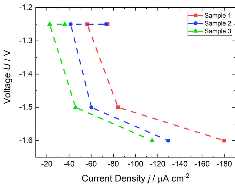
Fig. 6.11. Polarisation curves of the three samples, which were used for electrochemical \text{NH}_3 production. These three samples, three MEA cells, had identical materials and were operated under equivalent conditions.
