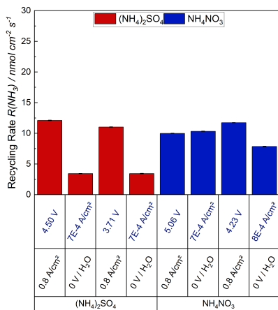
(a) Recycling Rate @ 5 mL/min, RT
