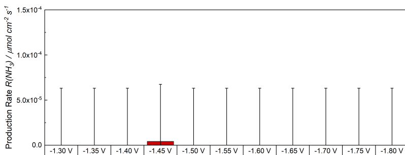
Fig. 6.19. Calculated rates of NH 3 production and the corresponding error bars that were determined while N 2 was supplied at the specific conditions.
