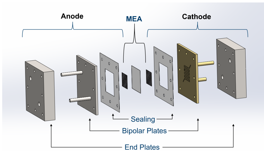
Fig. 3.3. The end plate, which are made of stainless steel enables the electrical contact of the cell components and applies mechanical compression to the cell. The flow fields in the bipolar plates channels the reactants into the cell and exports the products out of the cell. The anode bipolar plate is coated in platinumium and the cathode one in gold. The flat sheet sealing is PTFE, which is adapted to the thickness of the porous transport layers of the MEA. In the center of the cell is the MEA, which consist of PTLs on anode and cathode side, catalyst layers and the membrane. The catalyst layers can be coated on either the PTLs or the membrane.
