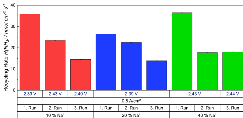
Fig. 8.17. The recycling rates in dependency of the added amount of \text{Na}^+ . The solution of the red shaped production rates contained 10 %, the solution of the blue depicted rates 20 %, and the green one 40 % \text{Na}^+ .
