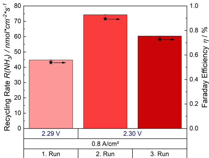
Fig. 8.15. Recorded recycling rates of \text{NH}_3 during non-recirculation / constant concentration of \text{NH}_4^+ in the introduced solution (left y-axis). The Faraday efficiency of the runs is shown as black stars (right y-axis). In black the applied current density is written and in dark blue the corresponding measured potentials.
