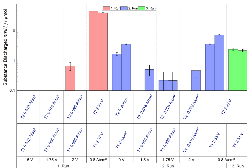
Fig. 7.8. Expelled amount of \text{NH}_3 of the 1:1 ratio, a logarithmic scale is used. The red color represents the measurement protocol of the first run, the blue the second, and the green the third run. The applied potentials / current densities are written in black, while the measured potentials / current densities are written in blue.
