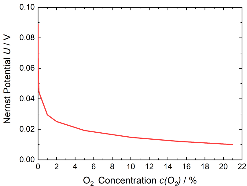
Fig. 5.4. The Nernst potential is plotted as a function of the O_2 concentration of the gas mixture at the cathode.
