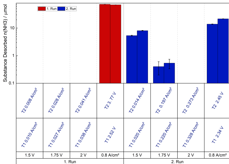
Fig. 7.7. Expelled amount of \text{NH}_3 of the 2:1 ratio, a logarithmic scale is used. The red color represents the measurement protocol of the first run and the blue of the second run. The applied potentials / current densities are written in black, while the measured potentials / current densities are written in blue.
