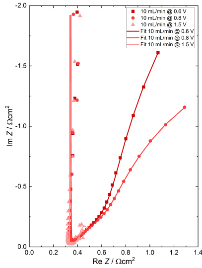
Fig. 5.14. EIS of an air flow rate of 10 mL/min and their respective fits.
