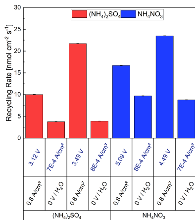
(b) Recycling Rate @ 20 mL/min, RT
