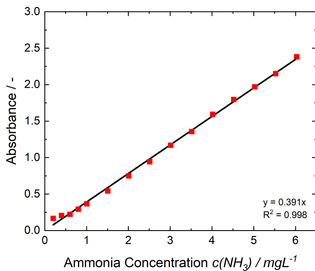
Fig. 3.8. Calibration line of the \text{NH}_3 samples of the known concentration in range from 0 to 6 \text{ mgL}^{-1} . The red dots are the measured absorbance of the calibration samples.
