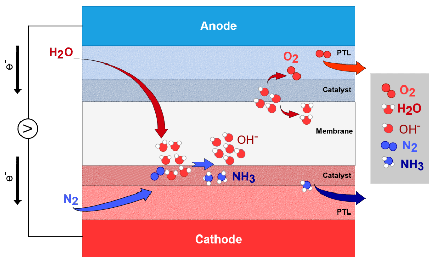
Fig. 4.5. Schematic illustration of the direct electrochemical \text{NH}_3 synthesis and the movement of molecules and ions in an alkaline cell. \text{H}_2\text{O} is introduced into the PTL of the anode, where it diffuses through the membrane. \text{N}_2 , which is supplied at the cathode, reacts with \text{H}_2\text{O} and the electrons to \text{NH}_3 and \text{OH}^- in the catalyst layer. This process is facilitated by the applied electrical energy. The resulting \text{NH}_3 exits the cell on the cathode side. Concurrently, \text{OH}^- diffuses through the membrane and oxidizes to \text{O}_2 and \text{H}_2\text{O} . The produced \text{O}_2 exits the cell on the anode side. The coloring of the atoms is done according to the CPK color model.
