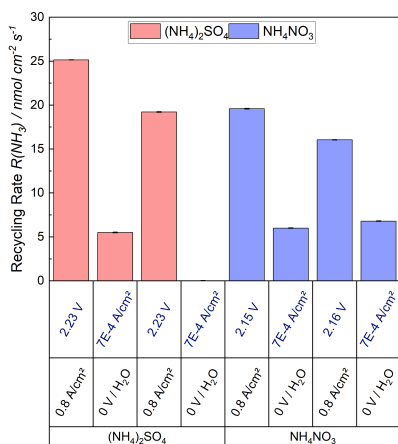
(c) Recycling Rate @ 5 mL/min, 80 °C
