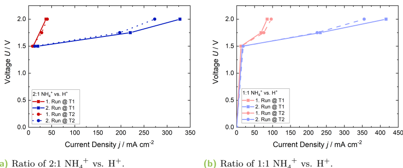
Fig. 7.11. Polarisation curves for both trials at RT. The first trials are depicted as the solid lines with square dots and the second trials as dashed lines with circular dots. The measured current densities for the first runs are shown in red, that for the second run in blue.
