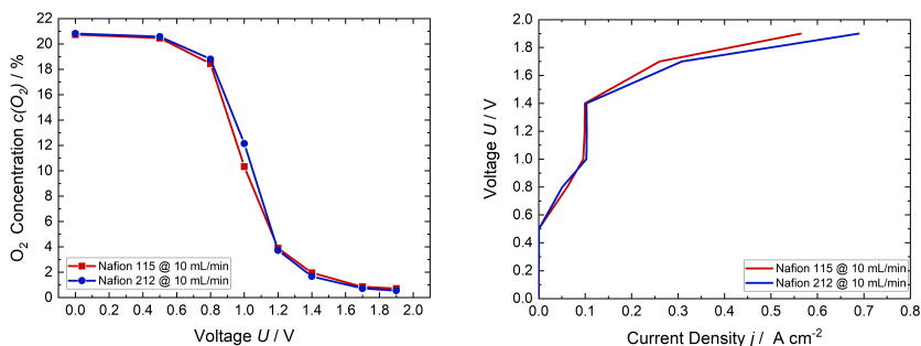
(a) \text{O}_2 depletion of Nafion 115 (red) and Nafion 212 (blue). (b) Current density of Nafion 115 (red) and Nafion 212 (blue).
