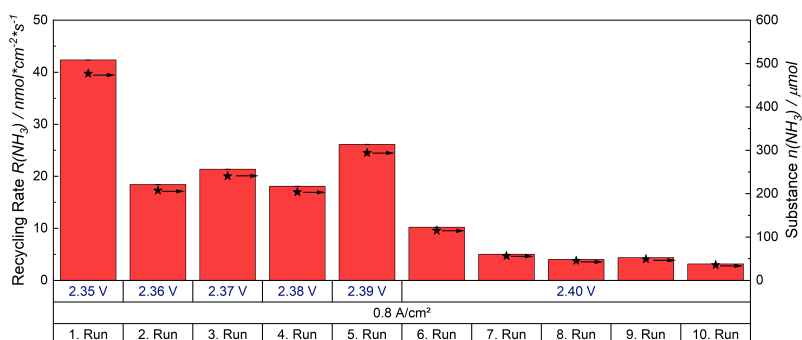
Fig. 8.16. Recorded recycling rates of each run (red bars, left y-axis). The corresponding substance of \text{NH}_3 , which was recycled each run (black stars, right y-axis). In black the applied current density is written and in dark blue the corresponding measured potentials.
