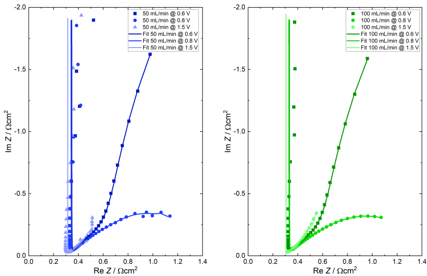
(a) EIS of an air flow rate of 50 mL/min and their (b) EIS of an air flow rate of 100 mL/min and their respective fits.
