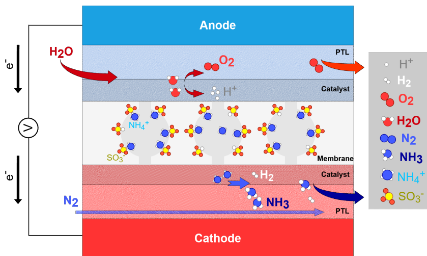
Fig. 7.5. Schematic illustration of the exchange and desorption process of \text{NH}_4^+ within the membrane. \text{H}_2\text{O} is introduced into the PTL of the anode. In the catalyst layer it oxidizes to \text{O}_2 and \text{H}^+ . The produced \text{O}_2 exits the cell on the anode side. The generated \text{H}^+ interacts with \text{NH}_4^+ within the membrane. \text{NH}_4^+ is displaced with \text{H}^+ . \text{NH}_4^+ desorbs from the membrane. At the cathode, \text{NH}_4^+ deprotonates, producing \text{NH}_3 . The dissociated \text{H}^+ is reduced to \text{H}_2 with the supplied \text{e}^- from the cathode. \text{N}_2 is used as carrier gas to remove \text{NH}_3 and \text{H}_2 from the cell. The coloring of the atoms is done according to the CPK color model.
