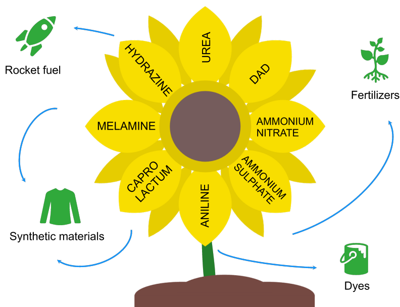
Fig. 1.1. Schematic illustration of nitrogen compounds synthesized from \text{NH}_3 and their respective field of application involving, fertilizers, rocket fuel, dyes and synthetic materials.
