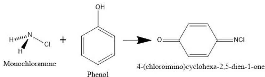
Fig. 3.4. The reaction of monochloramine with phenol.
