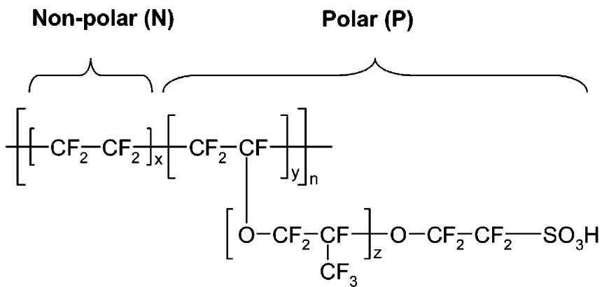
Fig. 1.8. Nafion structural formula. Nafion consist of a non-polar and polar part. The sulphit ion is incorporated into the chemical structure of Nafion. The attached H^+ ensure charge neutrality in the membrane. Adapted with permission from [62], American Chemical Society.
