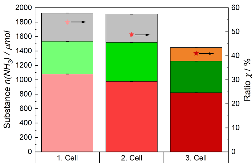
Fig. 8.12. Totaled recycled quantities of \text{NH}_3 of each cell is shown in the different red shades. In green the remaining quantity of \text{NH}_4^+ of each solution is illustrated. In grey the assumed adsorbed quantity of \text{NH}_4^+ within the membrane and in orange the detected quantity of \text{NH}_4^+ which was still in the the same membrane are shown (left y-axis). The ratios of recycled quantity to the initial amount of \text{NH}_4^+ in the solution are shown as the corresponding red stars (right y-axis).
