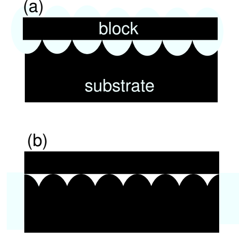
FIG. 1: Contact between a rigid block with a flat surface and a rigid substrate with periodic surface structures. The two substrate surfaces in (a) and (b) have the same surface roughness power spectrum. Note that the empty volume between the surfaces is much larger in the case (a) than in case (b).
