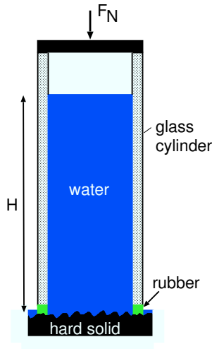
FIG. 2: Experimental set-up for measuring the leak-rate of seals. A glass (or PMMA) cylinder with a rubber ring attached to one end is squeezed against a hard substrate with well-defined surface roughness. The cylinder is filled with water, and the leak-rate of the water at the rubber-countersurface is detected by the change in the height of the water in the cylinder.
