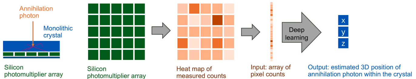
Fig. 4. Intrinsic detector resolution with monolithic scintillation crystals. Deep learning-based prediction of the 3D photon interaction position within the crystal from the measured light distribution pattern.
