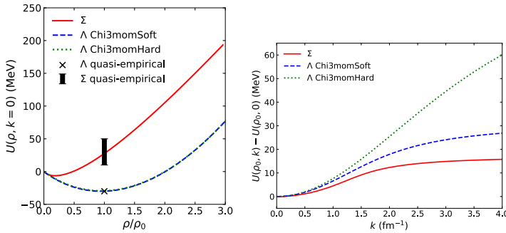
Figure 1. Density dependence (left panel) and momentum dependence (right panel) of the \Lambda and \Sigma single-particle potentials in symmetric nuclear matter. The momentum dependence is subtracted by its value at k = 0 . The single-particle potentials are fitted to the results obtained for two- and three-body forces based on chiral EFT. The solid lines correspond to the \Sigma single-particle potential. The dashed and dotted lines represent the \Lambda single-particle potentials with different momentum dependencies above k > 1 \text{ fm}^{-1} . The quasi-empirical values at \rho_0 are taken from Ref. [8].
