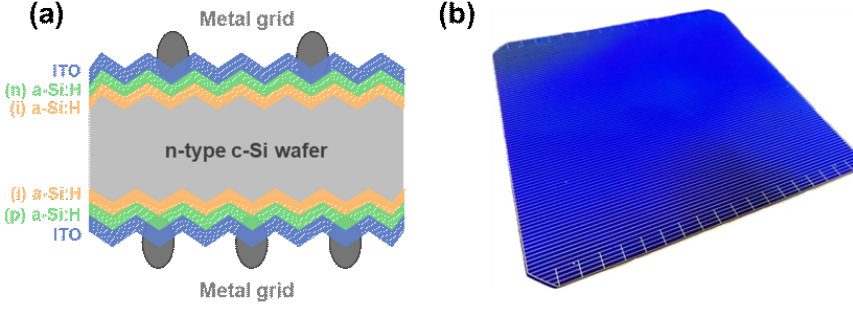
Figure 2.1: (a) Schematic structure of an n-type rear-emitter silicon heterojunction (SHJ) solar cell; (b) Image of the actual SHJ solar cell developed in FZJ [47].
