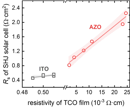
Figure 4.10: Relationship between the series resistance ( R_s ) of ITO- and AZO-incorporated SHJ solar cells and the resistivity ( \rho ) of the corresponding TCO films.
