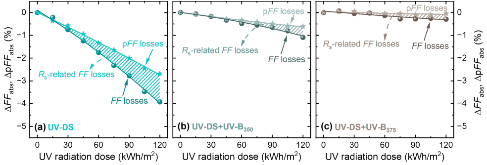
Figure 6.21: Changes in pseudo fill factor (pFF) and fill factor (FF) of lightweight SHJ solar modules with (a) UV-DS, (b) UV-DS+UV-B 350 and (c) UV-DS+UV-B 375 , as a function of UV radiation dose. \Delta pFF_{abs} and \Delta FF_{abs} denote the absolute changes in pFF and FF, respectively.
