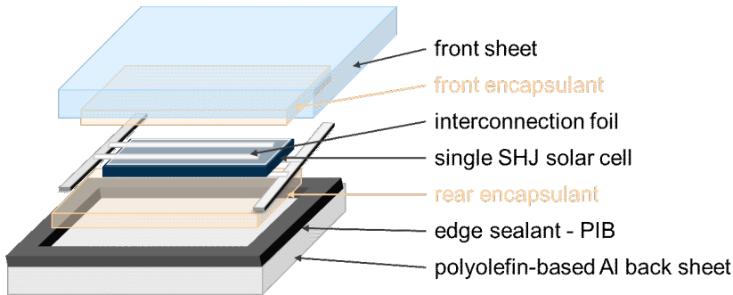
Figure 6.5: Schematic of the lightweight SHJ single-cell solar module.
