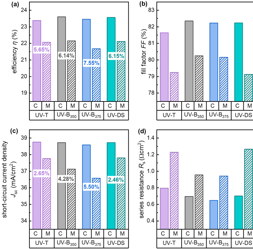
Figure 6.6: CTM loss from (a) efficiency ( \eta ), (b) fill factor ( FF ), (c) short-circuit current density ( J_{sc} ), and (d) series resistance ( R_s ) of lightweight SHJ solar modules incorporating encapsulants with different UV-transmission properties. 'C' denotes solar cell, and 'M' denotes solar module.
