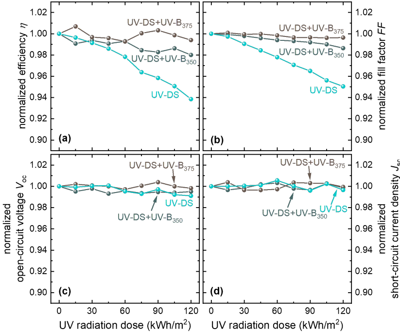
Figure 6.19: Normalized values of (a) efficiency ( \eta ), (b) fill factor ( FF ), (c) open-circuit voltage ( V_{oc} ) and (d) short-circuit current density ( J_{sc} ) as a function of UV radiation dose for lightweight SHJ solar modules with UV-DS, UV-DS+UV-B 350 , and UV-DS+UV-B 375 as the front encapsulant.
