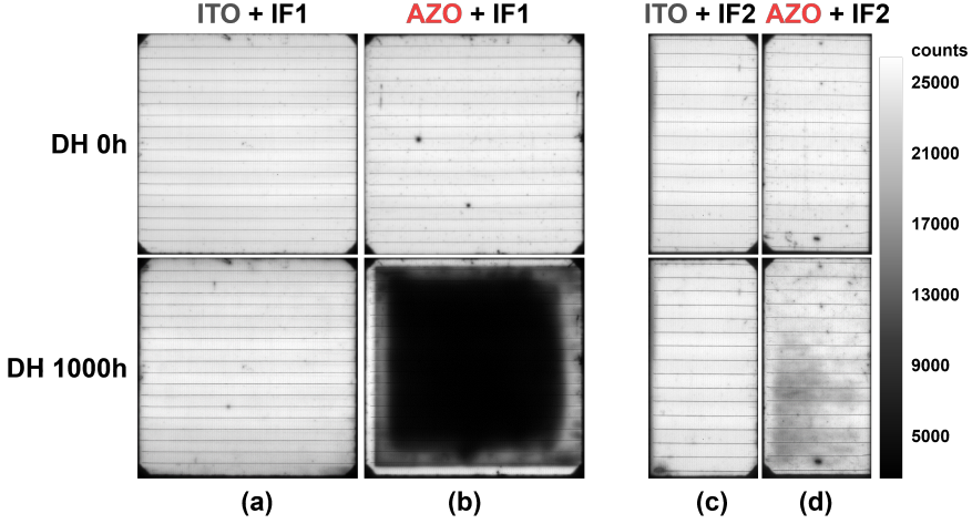
Figure 4.27: EL images under low current injection ( J = 2.03 \text{ mA/cm}^2 ) of ITO- and AZO-incorporated FS/BS solar modules in combination with two different interconnection foils (IF1 and IF2), before and after 1000 h of DH. (a) ITO + IF1, (b) AZO + IF1, (c) ITO + IF2, and (d) AZO + IF2.
