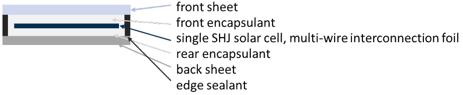
Figure 3.7: Schematic cross-section of the lightweight SHJ single-cell solar module (optimized design).
