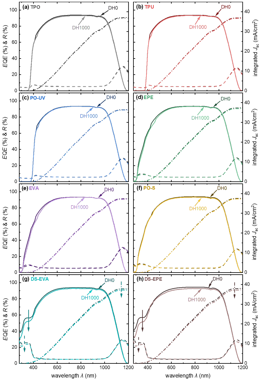
Figure 5.18: EQE (solid line), reflectance (dashed line), and integrated short-circuit current density ( J_{sc} ) (dashed dot line) of the modules encapsulated with different encapsulants: (a) TPO, (b) TPU, (c) PO-UV, (d) EPE, (e) EVA, (f) PO-S, (g) DS-EVA, and (h) DS-EPE before and after 1000 h of the DH test.
