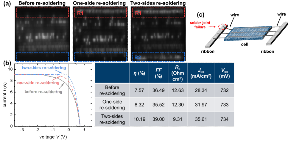
Figure 5.9: (a) EL images of the EPE solar module before and after two re-solderings. The dark band defects are marked by red and blue dashed rectangles. R1 stands for the first re-soldering. R2 stands for the second re-soldering, which means that the two sides were re-soldered. (b) Light I - V curves of the EPE solar module before and after two re-solderings and the corresponding I - V characteristics. (c) Schematic of the solder joint failure between wire and ribbon.
