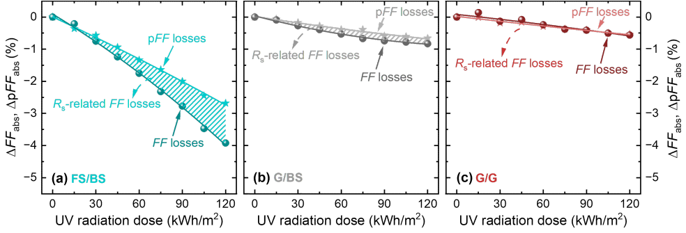
Figure 6.16: Changes in pseudo fill factor (pFF) and fill factor (FF) of solar modules with UV-DS encapsulant in different solar module structures: (a) front sheet/back sheet (FS/BS), (b) glass/back sheet (G/BS), and (c) glass/glass (G/G), as a function of UV radiation dose. \Delta pFF_{\text{abs}} and \Delta FF_{\text{abs}} denote the absolute changes in pFF and FF, respectively.
