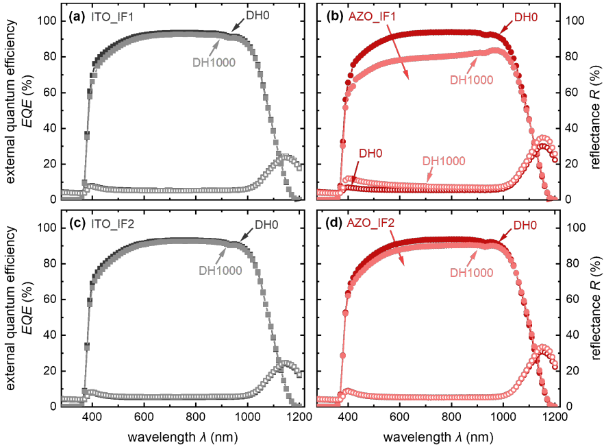
Figure 4.29: EQE (solid symbols) and reflectance (hollow symbols) of ITO- and AZO-incorporated FS/BS solar modules in combination with two different interconnection foils (IF1 and IF2), before and after 1000 h of DH. (a) ITO + IF1, (b) AZO + IF1, (c) ITO + IF2, and (d) AZO + IF2.
