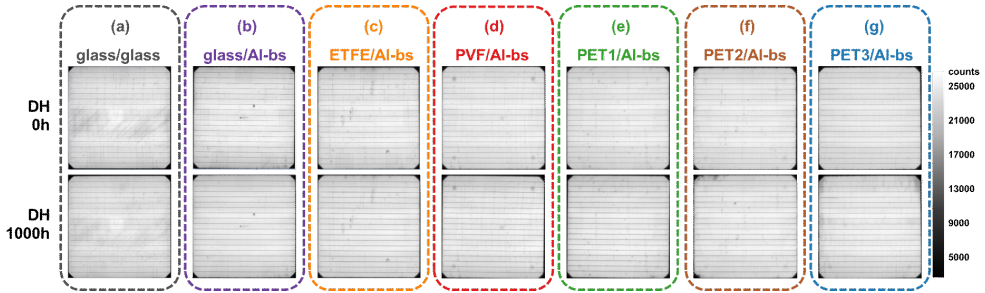
Figure 5.25: EL images (low current injection, J = 2.05 \text{ mA/cm}^2 ) of the solar modules with different front sheets before (0 h) and after 1000 h of the DH test.
