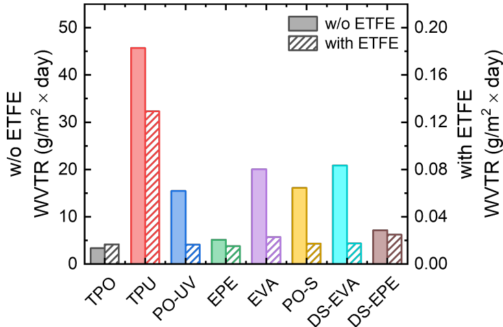
Figure 5.2: WVTR of different encapsulants in plain laminated foil form and in combination with ETFE foil.
