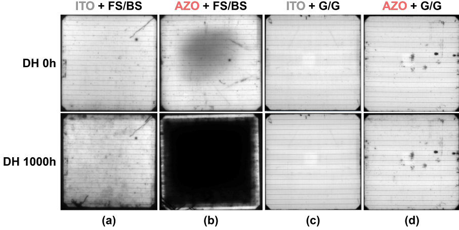
Figure 4.4: EL images under low current injection ( J = 2.03 \text{ mA/cm}^2 ) of SHJ solar modules with ITO and AZO layer in different configurations: (a) ITO-incorporated SHJ solar module with front sheet/back sheet (FS/BS), (b) AZO-incorporated SHJ solar module with front sheet/back sheet (FS/BS), (c) ITO-incorporated SHJ solar module with glass/glass (G/G), and (d) AZO-incorporated SHJ solar module with glass/glass (G/G), taken before and after 1000 h of the DH test.
