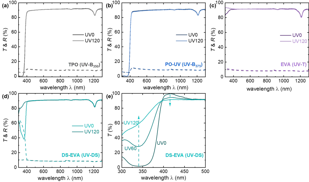
Figure 6.3: Transmittance ( T ) (solid line) and reflectance ( R ) (dashed line) spectra of different encapsulants: (a) TPO, (b) PO-UV, (c) EVA, (d) DS-EVA, and (e) DS-EVA, measured using an in-house-built setup, before and after UV exposure with a total dose of 120 kWh/m 2 . (f) DS-EVA encapsulant is covered with ETFE foil on both the front and rear sides.
