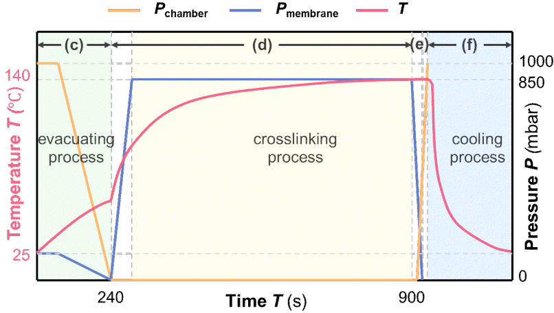
Figure 3.6: Temperature and pressure profiles of the lamination process used in the fabrication of the solar modules in this study. (c),(d),(e), and (f) refer to the steps shown in Figure 3.5.
