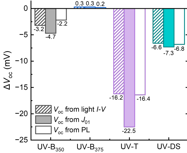
Figure 6.10: V_{oc} changes calculated from light I - V , J_{01} , and PL intensity for solar modules with: (a) UV-B 350 , (b) UV-B 375 , (c) UV-T, and (d) UV-DS, before and after 120 kWh/m 2 of UV exposure.
