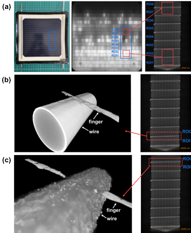
Figure 5.11: X-ray computed tomography (XCT) of the degraded EPE solar module: (a) X-ray scanning of two areas, ROI1-ROI2 and ROI7-ROI8, which contain two distinct EL intensities. (b) Reconstructed image showing intact interaction of the finger with the wire in the ROI1-ROI2 area. (c) Reconstructed image showing finger breakage in the ROI7-ROI8 area. The XCT images were taken by Zeiss Xradia Versa 620, voxel size is 740 nm, X-ray tube voltage is 100 kV, exposure time per projection is 15 s, and the number of projections is 1200.
