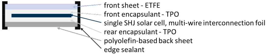
Figure 4.13: Schematic cross-section of a lightweight SHJ single-cell solar module with front sheet/back sheet (FS/BS) structure.
