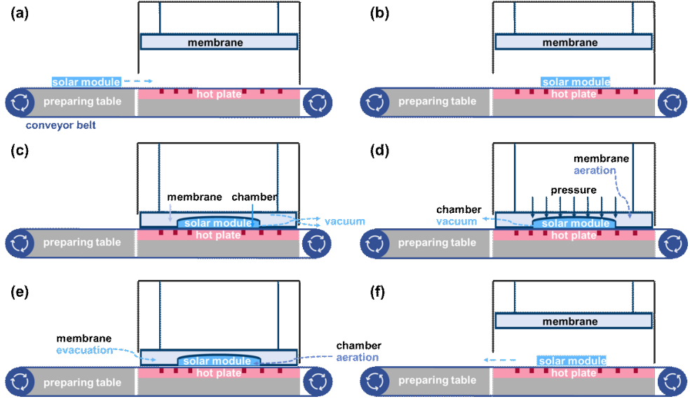
Figure 3.5: Schematic diagram of the lamination process: (a) Preparing the solar module on the preparing table; (b) Loading the solar module into the laminator; (c) The hot plate heats the solar module, the air in the membrane and chamber is evacuated to create a vacuum; (d) The chamber is evacuated and the membrane is aerated to apply pressure to the solar module. This pressure is maintained for a sufficient time to allow the encapsulant to crosslink; (e) The chamber is aerated, and the pressure in the membrane is gradually released; (f) The lamination process is complete; The solar module is then unloaded and allowed to cool naturally.
