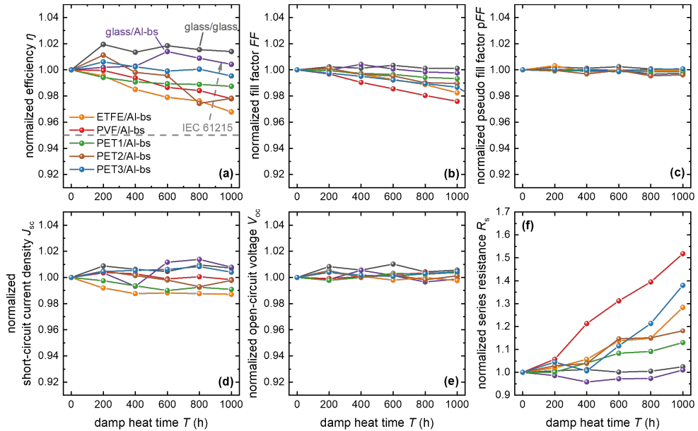
Figure 5.23: Normalized values of (a) efficiency ( \eta ), (b) fill factor ( FF ), (c) pseudo fill factor ( pFF ), (d) short-circuit current density ( J_{sc} ), (e) open-circuit voltage ( V_{oc} ), and (f) series resistance ( R_s ) as a function of damp-heat time for solar modules encapsulated with different front sheets.
