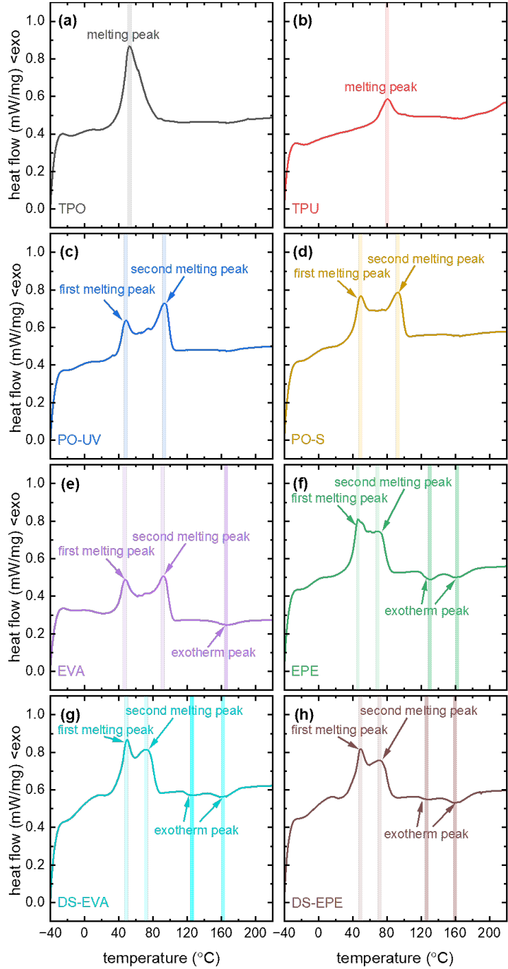
Figure 5.3: Differential scanning calorimetry (DSC) thermograms (first heating run) of the different pristine encapsulants.
