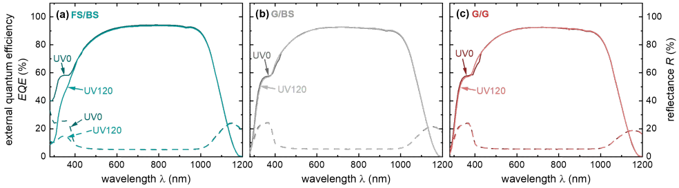
Figure 6.17: EQE (solid line) and reflectance (dashed line) of solar modules using UV-DS encapsulants in different solar module structures: (a) front sheet/back sheet (FS/BS), (b) glass/back sheet (G/BS) and (c) glass/glass (G/G), measured before and after 120 kWh/m 2 of UV exposure.
