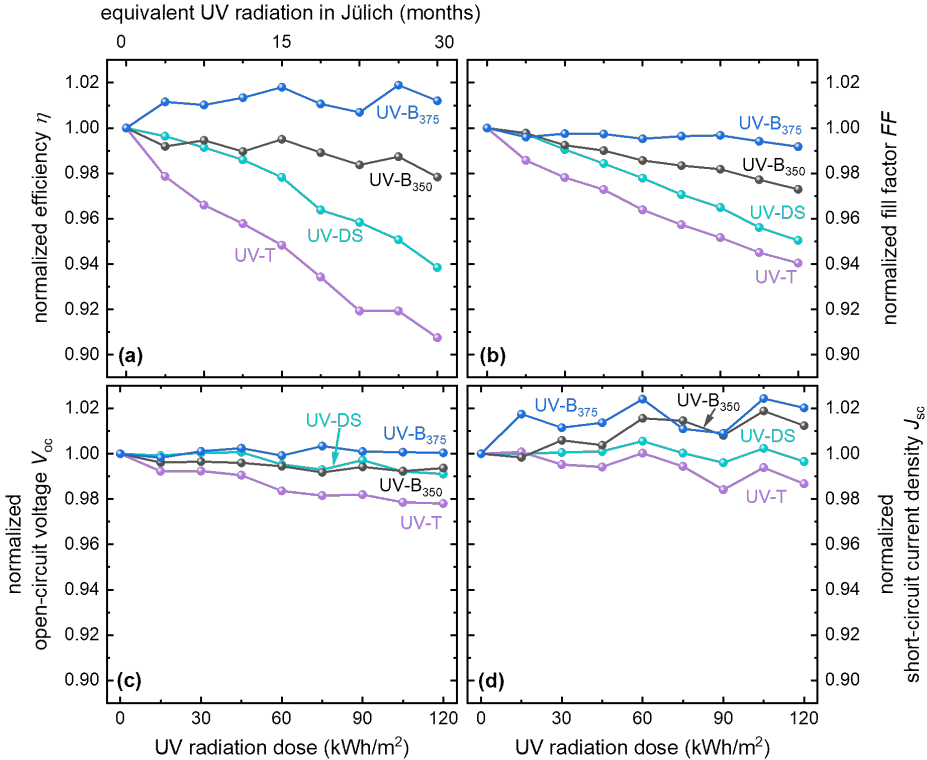
Figure 6.7: Normalized values of (a) efficiency ( \eta ), (b) fill factor ( FF ), (c) open-circuit voltage ( V_{oc} ), and (d) short-circuit current density ( J_{sc} ) as a function of UV radiation dose for lightweight SHJ solar modules incorporating encapsulants with different UV-transmission properties.
