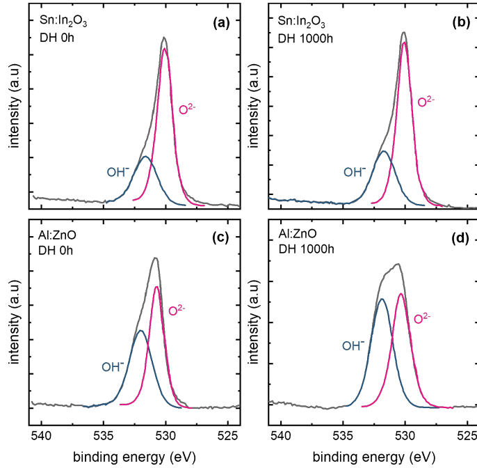
Figure 4.11: XPS analysis of AZO and ITO films before and after the 1000 h of the DH test: (a) ITO before DH, (b) ITO after DH, (c) AZO before DH, and (d) AZO after DH.
