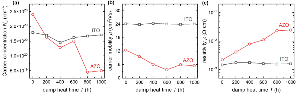
Figure 4.9: Evolution of (a) carrier (electron) density ( n_e ), (b) carrier (electron) mobility ( \mu_e ), and (c) resistivity ( \rho ) of 60-nm-thick AZO and 70-nm-thick ITO films deposited on Corning glass substrates during the DH test, measured using Hall-effect characterization.
