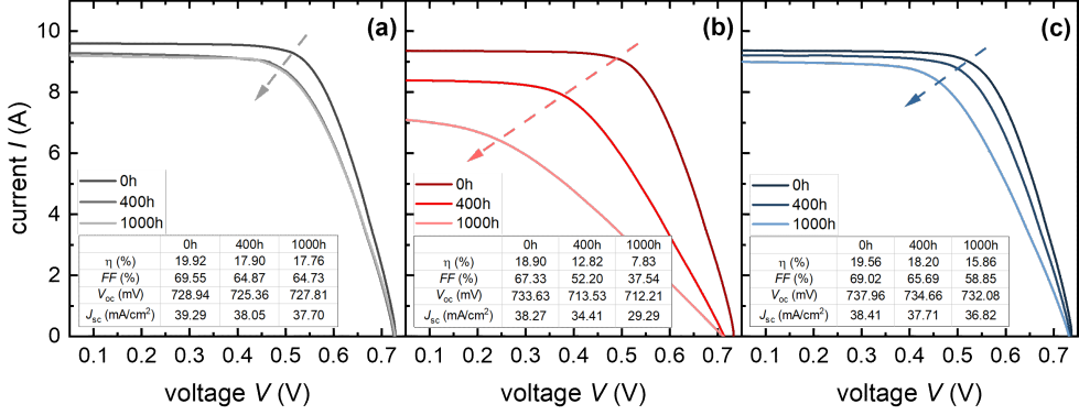
Figure 4.17: I - V curves of (a) ITO-, (b) AZO-, and (c) ITO/AZO/ITO-incorporated SHJ solar modules, measured before (0 h), after 400 h, and after 1000 h of DH exposure.
