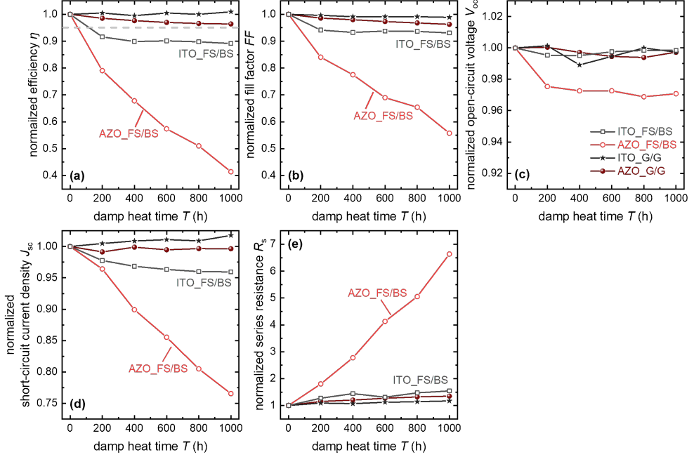
Figure 4.3: Normalized values of (a) efficiency ( \eta ), (b) fill factor ( FF ), (c) open-circuit voltage ( V_{oc} ), (d) short-circuit current density ( J_{sc} ), and (e) series resistance ( R_s ) as a function of damp-heat exposure time for ITO- and AZO-incorporated SHJ solar modules in front sheet/back sheet (FS/BS) or glass/glass (G/G) configurations.
