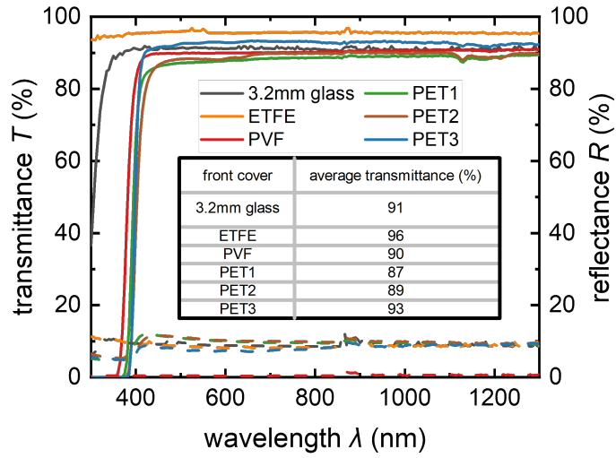
Figure 5.20: The transmittance ( T , solid line) and reflectance ( R , dashed line) of different front sheet materials.
