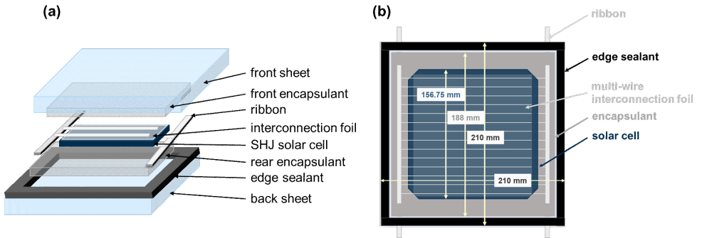
Figure 3.8: (a) Cross-section and layer-stack of the solar module and (b) top-view of the solar module, with optimized design.
