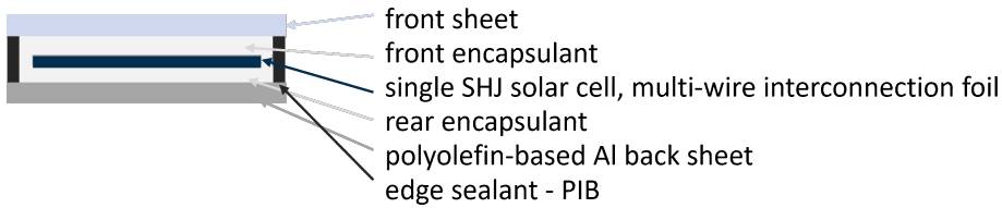
Figure 5.5: Schematic cross-section of the lightweight SHJ single-cell solar module.
