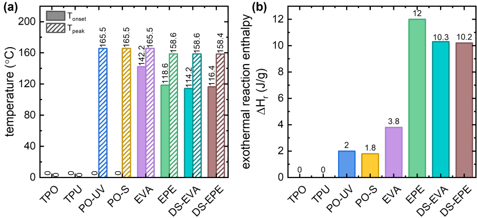
Figure 5.4: Differential scanning calorimetry (DSC), (a) T_{\text{onset}} (temperature at which chemical crosslinking commences) and T_{\text{peak}} (chemical crosslinking peak temperature); (b) Exothermal reaction enthalpy of different encapsulants.
