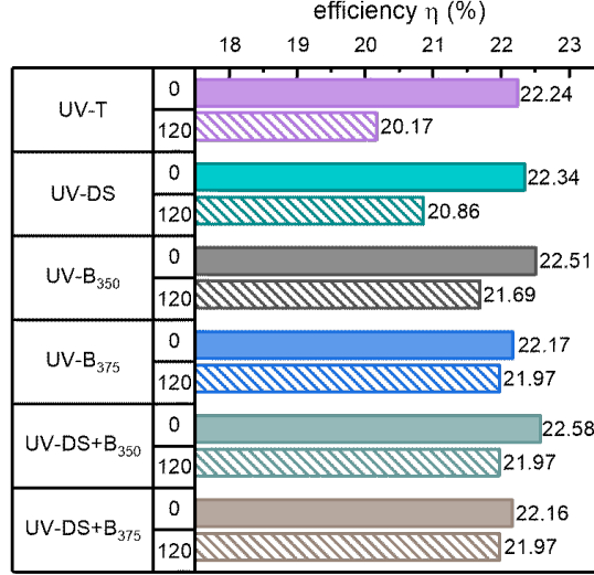
Figure 6.23: Solar module efficiencies before and after 120 kWh/m 2 of UV exposure, with currents for efficiency calculation derived from EQE measurements.
