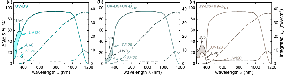
Figure 6.22: EQE (solid line) and reflectance ( R ) (dashed line) and integrated short-circuit current density ( J_{sc} ) (dashed dot line) of lightweight SHJ solar modules with (a) UV-DS, (b) UV-DS+UV-B 350 , and (c) UV-DS+UV-B 375 , measured before and after 120 kWh/m 2 of UV exposure.
