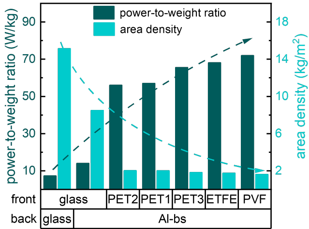
Figure 5.21: Power-to-weight ratio and area density of solar modules with different configurations.
