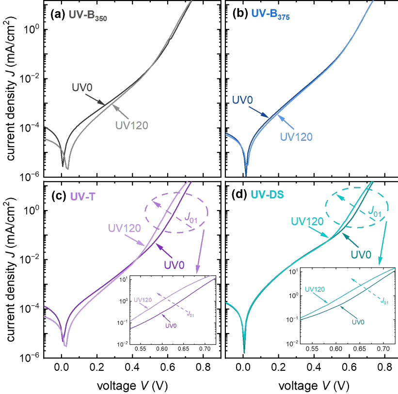
Figure 6.8: Dark J - V curves of the lightweight SHJ solar modules incorporating encapsulants with different UV-transmission properties: (a) UV-B 350 , (b) UV-B 375 , (c) UV-T, and (d) UV-DS, before and after 120 kWh/m 2 of UV exposure.
