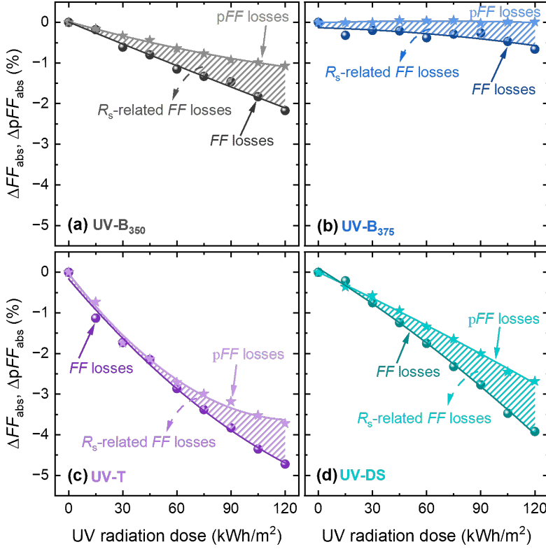
Figure 6.12: Changes in pseudo fill factor (pFF) and fill factor (FF) of lightweight SHJ solar modules incorporating encapsulants with different UV-transmission properties: (a) UV-B 350 , (b) UV-B 375 , (c) UV-T, and (d) UV-DS, as a function of UV radiation dose. \Delta pFF_{abs} and \Delta FF_{abs} denote the absolute changes in pFF and FF, respectively.
