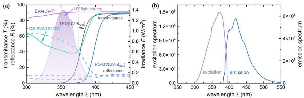
Figure 6.2: (a) Transmittance (solid line, T ) and reflectance (dashed line, R ) spectra of encapsulants with different UV-transmission properties in the range of 300 - 450 nm. The shaded curve shows the spectrum of the UV light source. (b) Excitation and emission spectra of the downshifting encapsulant foil (Source: from Cybrid).
