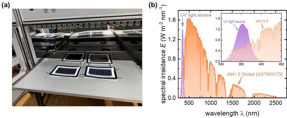
Figure 3.11: (a) Solar module samples in the UV chamber; (b) Spectrum of UV light source and sun spectrum at AM1.5G.
