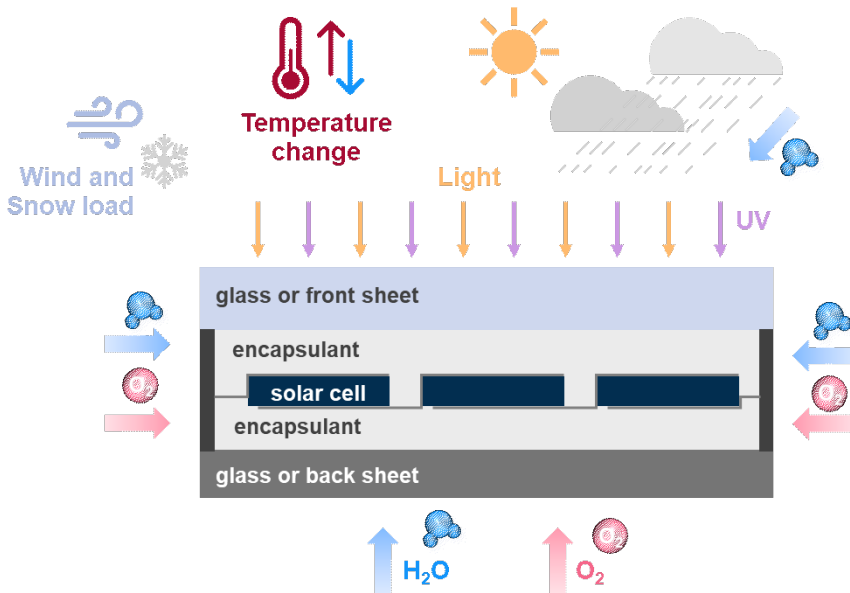
Figure 2.4: Key environmental stressors for solar modules during field operation.
