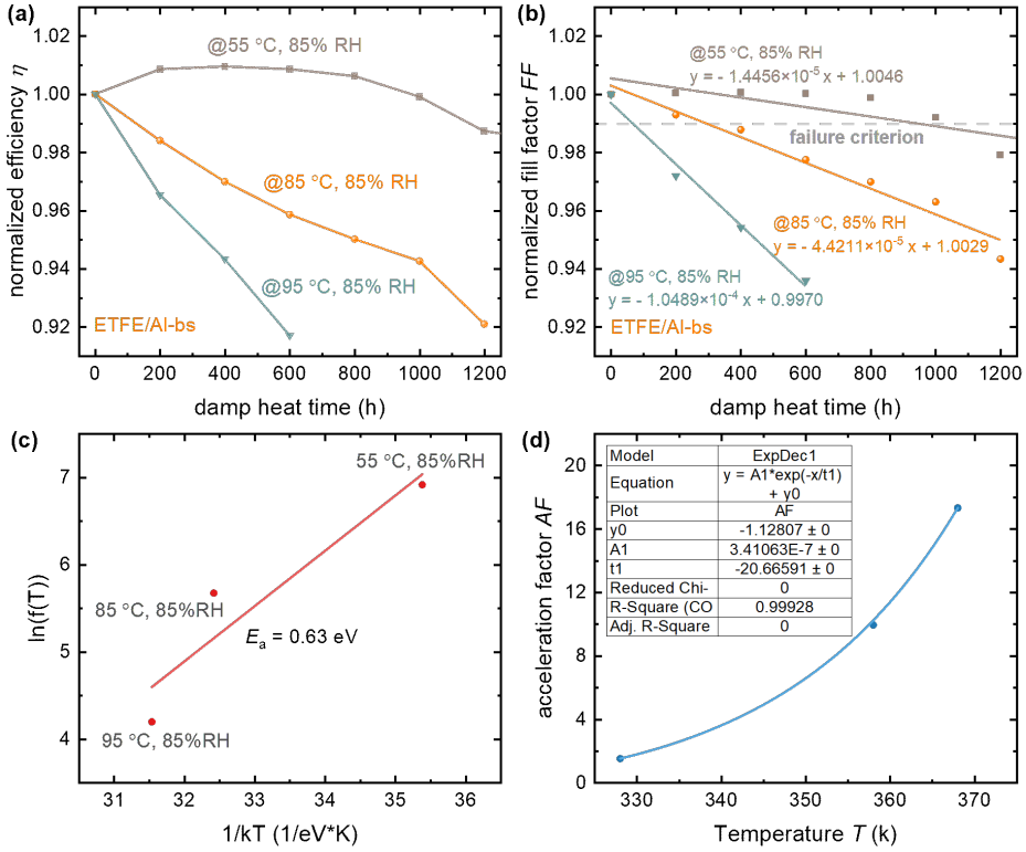
Figure 5.27: (a) Evolution of normalized efficiency ( \eta ) during DH test under different temperature conditions. (b) Linear fitting of FF degradation during DH test at various temperatures. (c) Lifetime variation of the ETFE/Al-bs solar module under different DH conditions, with E_a calculated based on the Arrhenius equation. (d) Exponential fitting of AF derived from different DH conditions.
