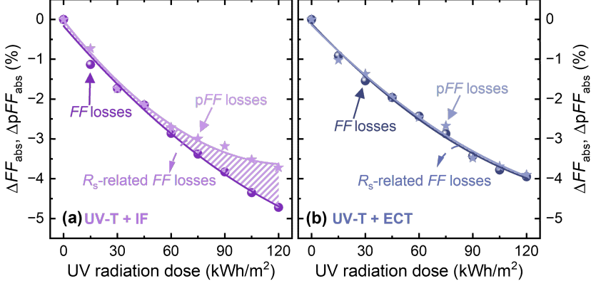
Figure 6.13: Changes in pseudo fill factor ( pFF ) and fill factor ( FF ) of the UV-T lightweight SHJ solar modules with different interconnection methods: (a) interconnection foil (IF1) and (b) electrically conductive adhesive tape (ECT), as a function of UV radiation dose. \Delta pFF_{abs} and \Delta FF_{abs} denote the absolute changes in pFF and FF , respectively.
