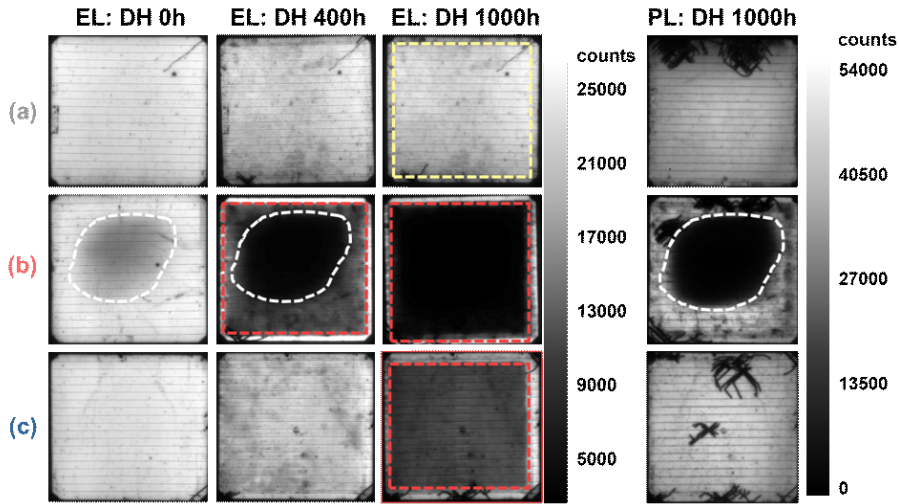
Figure 4.18: EL images under low current injection ( J = 2.03 \text{ mA/cm}^2 ) of (a) ITO-, (b) AZO-, and (c) ITO/AZO/ITO-incorporated SHJ solar modules before, after 400 h, and after 1000 h of DH test. The severe cracking observed in the PL image after 1000 h of DH test resulted from mechanical damage during transport after the I - V and EL measurements.
