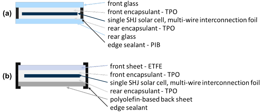
Figure 4.2: Schematic cross-section of the (a) glass/glass SHJ single-cell solar module, (b) front sheet/back sheet SHJ single-cell solar module.
