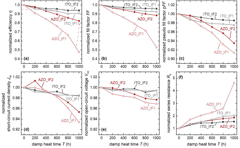
Figure 4.25: Normalized values of (a) efficiency ( \eta ), (b) fill factor ( FF ), (c) pseudo fill factor ( pFF ), (d) short-circuit current density ( J_{sc} ), (e) open-circuit voltage ( V_{oc} ), and (f) series resistance ( R_s ) as a function of damp-heat time for solar modules in combination with two different interconnection foils.
