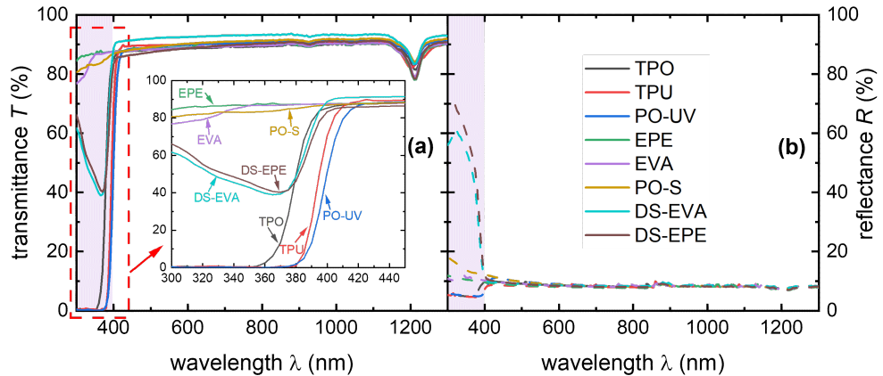
Figure 5.1: Optical properties of different encapsulants, (a) transmittance ( T ) and (b) reflectance ( R ). The inset graph shows the transmittance in the wavelength range from 300 - 450 nm.
