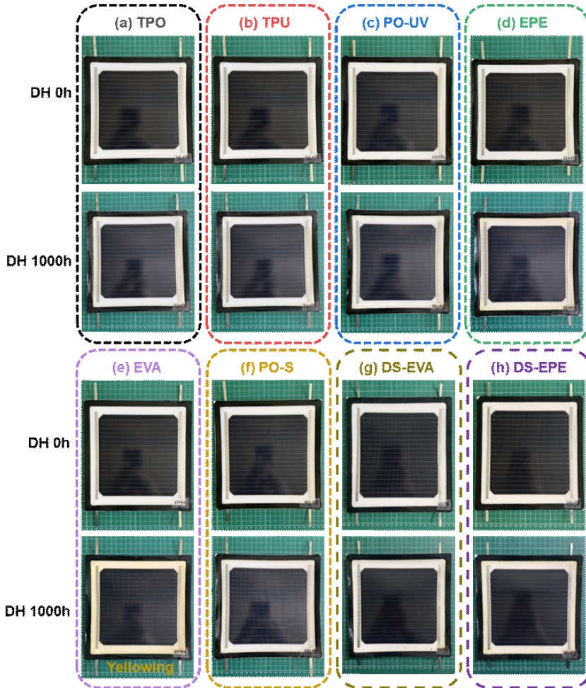
Figure 5.12: Visual images of modules encapsulated with different encapsulants (a) TPO, (b) TPU, (c) PO-UV, (d) EPE, (e) EVA, (f) PO-S, (g) DS-EVA, and (h) DS-EPE before and after 1000 h of the DH test.
