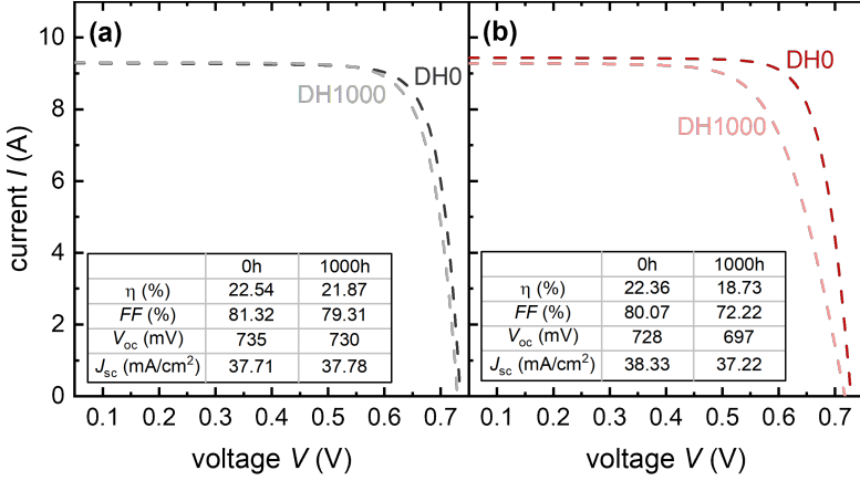
Figure 4.6: I - V curves of each solar cell sample: (a) ITO, (b) AZO, before and after 1000 h of the DH test.
