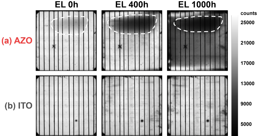
Figure 4.7: EL images under high current injection ( J = 32.49 mA/cm 2 ) of the SHJ solar cells with (a) AZO and (b) ITO layers, taken before, after 400 h, and after 1000 h of the DH test.
