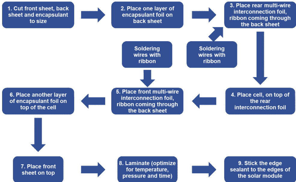
Figure 3.4: Fabrication process of lightweight SHJ single-cell solar modules (preliminary design).
