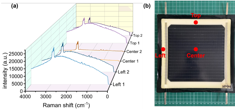
Figure 5.15: (a) Raw Raman spectra of EVA encapsulants at different locations (left, center, and top) in the EVA module after 1000 h of the DH test. (b) Indicating the left, center, and top positions in the solar module.
