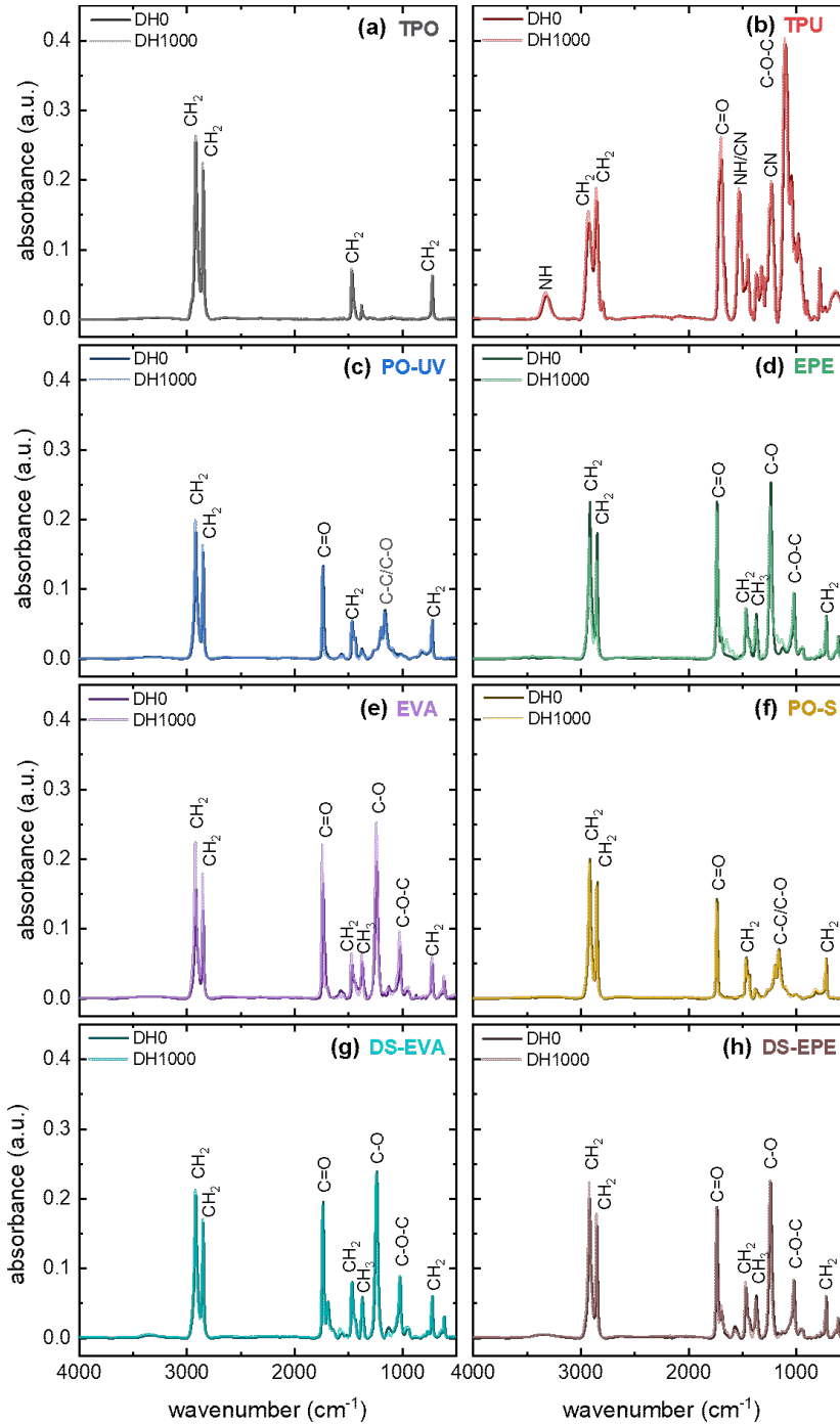
Figure 5.17: Normalized FTIR spectra of encapsulant samples (a) TPO, (b) TPU, (c) PO-UV, (d) EPE, (e) EVA, (f) PO-S, (g) DS-EVA, and (h) DS-EPE before and after 1000 h of the DH test.
