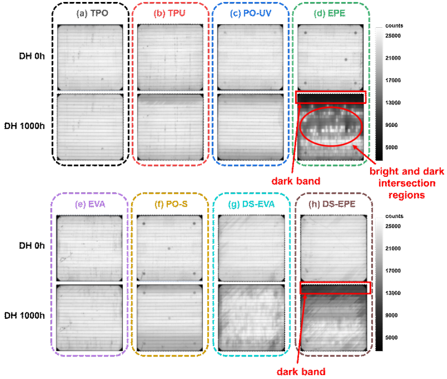
Figure 5.8: EL images (low current injection, J = 2.05 \text{ mA/cm}^2 ) of the solar modules with different encapsulants before and after 1000 h of the DH test.
