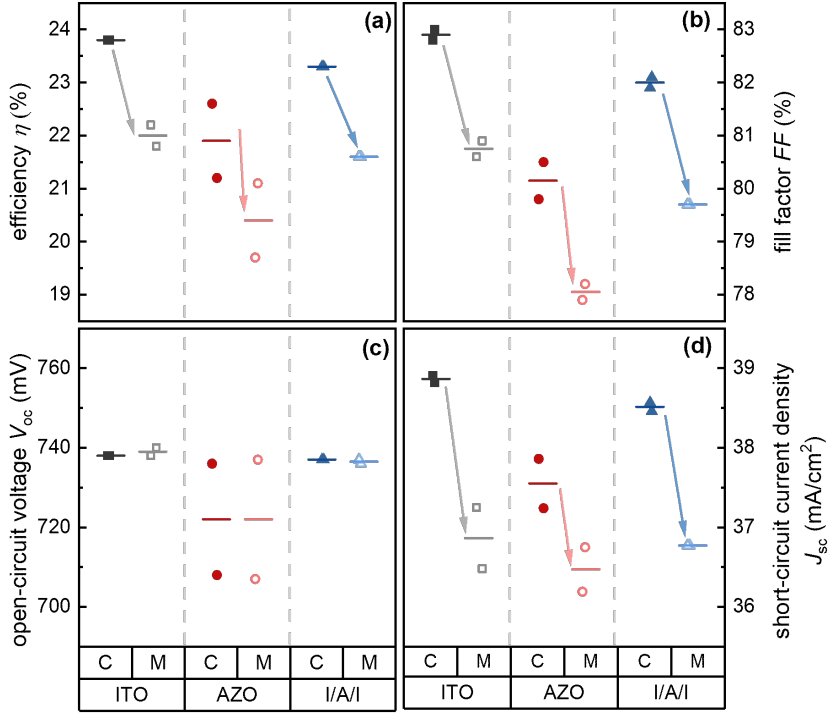
Figure 4.14: CTM analysis of (a) efficiency ( \eta ), (b) fill factor ( FF ), (c) open-circuit voltage ( V_{oc} ), and (d) short-circuit current density ( J_{sc} ). 'C' denotes the solar cell, 'M' denotes the solar module, and 'I/A/I' denotes the ITO/AZO/ITO.
