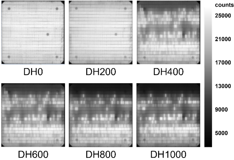
Figure 5.10: Evolution of EL images (low current injection, J = 2.05 \text{ mA/cm}^2 ) of the EPE solar module in every 200 hours during DH aging.
