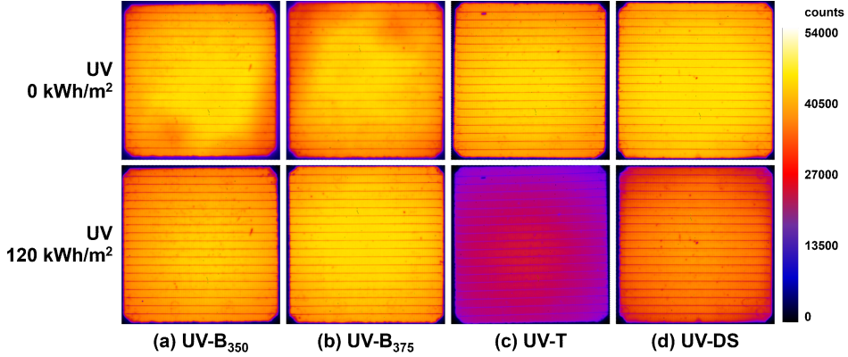
Figure 6.9: PL images of the lightweight SHJ solar modules incorporating encapsulants with different UV-transmission properties: (a) UV-B 350 , (b) UV-B 375 , (c) UV-T, and (d) UV-DS, before and after 120 kWh/m 2 of UV exposure.
