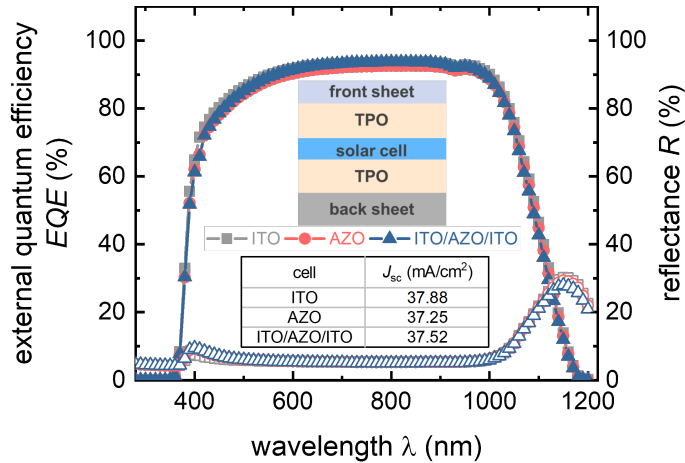
Figure 4.15: EQE (solid symbols) and reflectance (hollow symbols) spectra of the solar modules with three types of TCO layers. A schematic of the single-cell solar module sample is shown in the inset.
