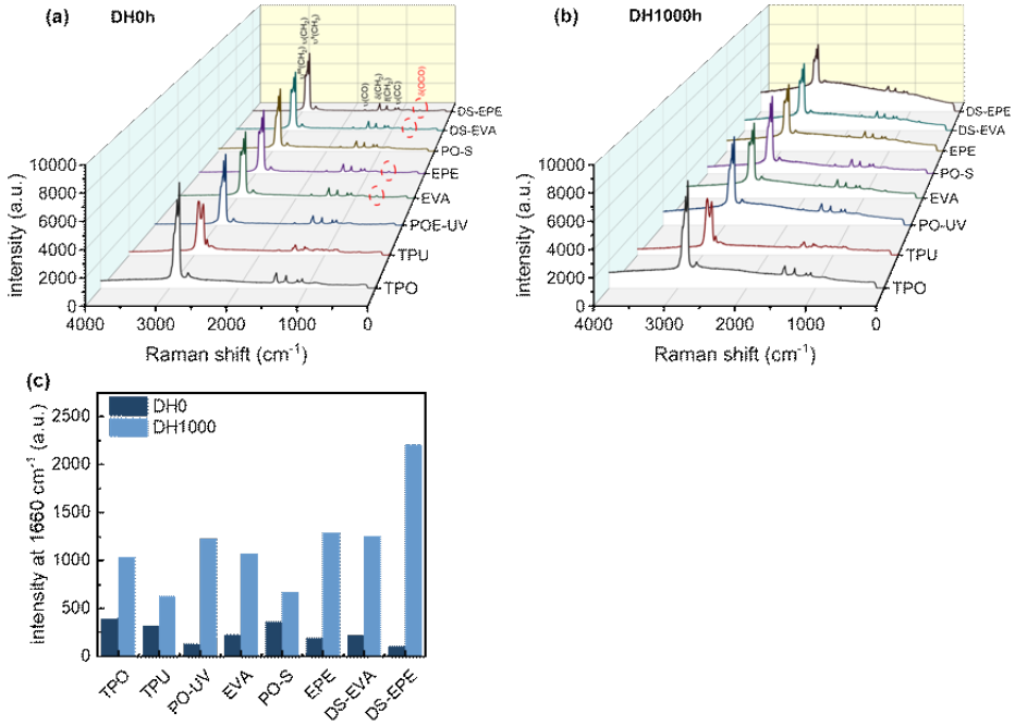
Figure 5.14: Raw Raman spectra of encapsulant samples (a) before and (b) after 1000 h of the DH test. (c) Fluorescence background intensity of the solar modules at 1660 cm -1 before and after 1000 h of the DH test.
