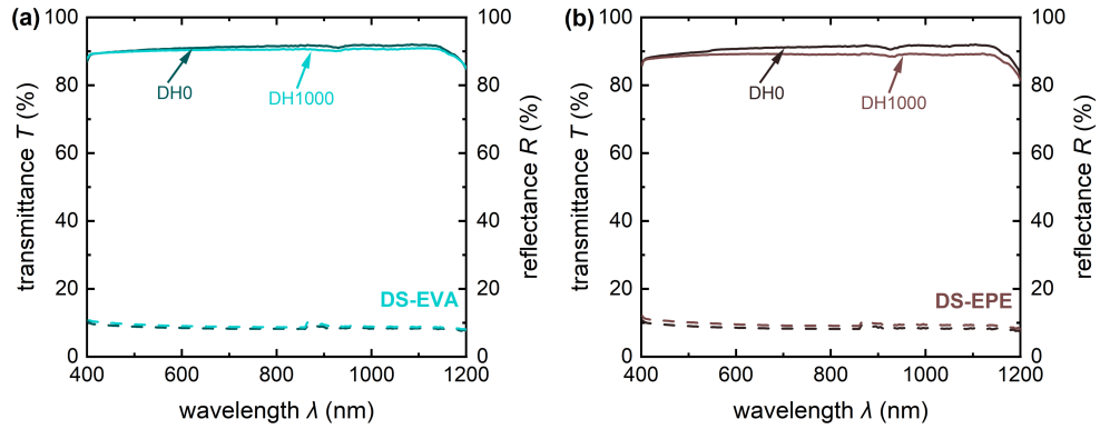
Figure 5.19: Transmittance T (solid line) and reflectance R (dashed line) of (a) DS-EVA encapsulant foil and (b) DS-EPE encapsulant foil before and after 1000 h of the DH test.
