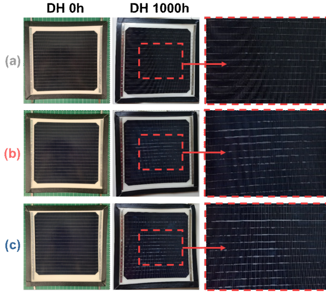
Figure 4.19: Visual inspection images of the lightweight SHJ solar modules with different TCOs: (a) ITO, (b) AZO, and (c) ITO/AZO/ITO before and after 1000 h of DH test. Delamination along the interconnection wires is clearly visible in (b) AZO and (c) ITO/AZO/ITO samples, indicating severe adhesion failure. The slight yellow tint in the images taken before the DH test is due to differences in lighting conditions during photography.
