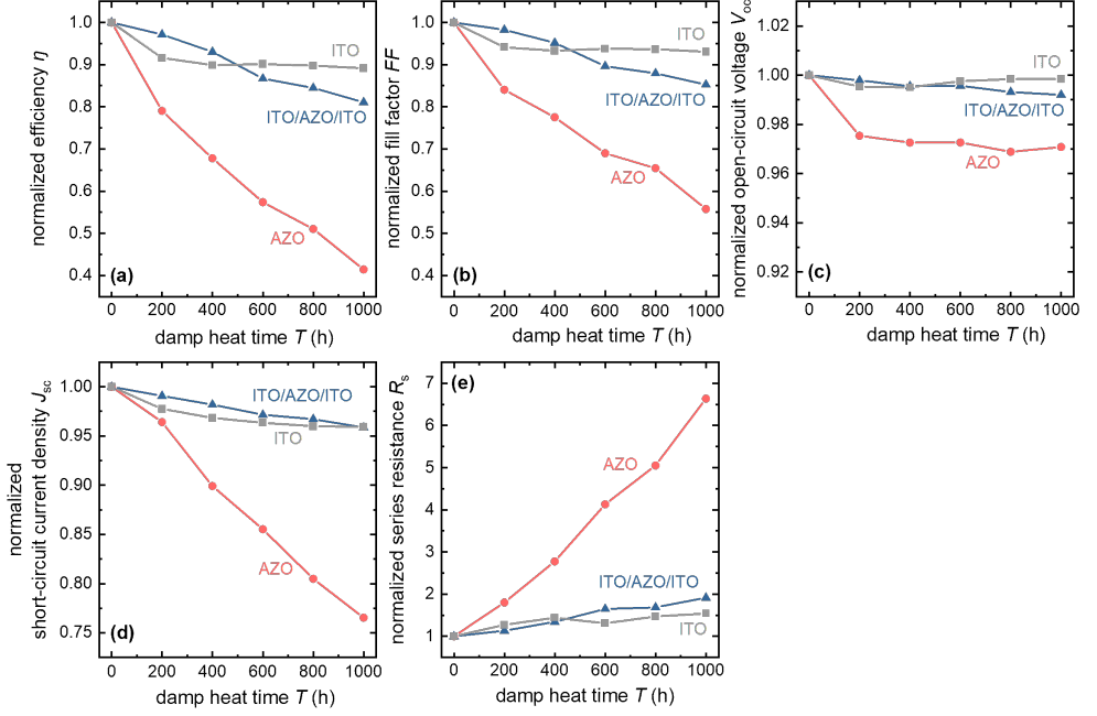
Figure 4.16: Normalized values of (a) efficiency ( \eta ), (b) fill factor ( FF ), (c) open-circuit voltage ( V_{oc} ), (d) short-circuit current density ( J_{sc} ), and (e) series resistance ( R_s ) as a function of damp-heat exposure time for lightweight SHJ solar modules with different TCO layers.
