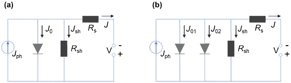
Figure 3.14: The equivalent circuit diagram of the (a) one-diode model, and (b) two-diode model, including the series resistance ( R_s ) and the shunt resistance ( R_{sh} ).
