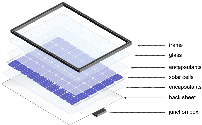
Figure 2.2: Schematic structure of a typical glass c-Si solar module.
