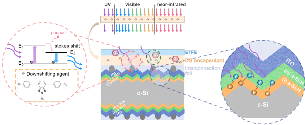
Figure 6.14: Schematic diagram of the working principle of UV-downshifting effect (marked by red circle), degradation mechanism of the downshifting (DS) effect (marked by green circle), and UVID mechanism in SHJ solar cells (marked by blue circle).
