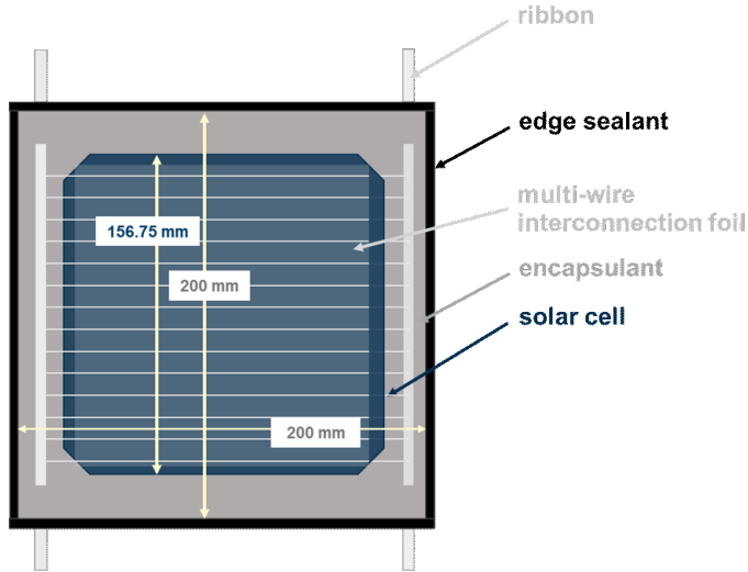
Figure 3.3: Top view of the lightweight SHJ single-cell solar module (preliminary design).
