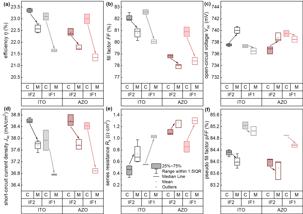
Figure 4.24: CTM analysis of (a) efficiency ( \eta ), (b) fill factor ( FF ), (c) open-circuit voltage ( V_{oc} ), (d) short-circuit current density ( J_{sc} ), (e) series resistance ( R_s ), and (f) pseudo fill factor ( pFF ). 'C' denotes the solar cell, and 'M' denotes the solar module.
