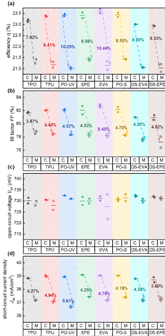
Figure 5.6: CTM loss of (a) efficiency ( \eta ), (b) fill factor ( FF ), (c) open-circuit voltage ( V_{oc} ) and (d) short-circuit current density ( J_{sc} ) of solar modules with different encapsulants. 'C' denotes the solar cell, and 'M' denotes the solar module.
