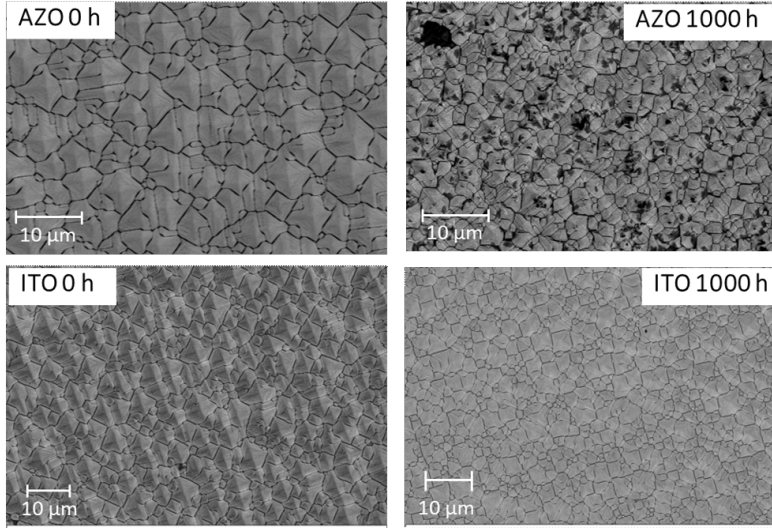
Figure 4.8: SEM images of AZO- and ITO-incorporated SHJ solar cells before and after 1000 h of the DH test.
