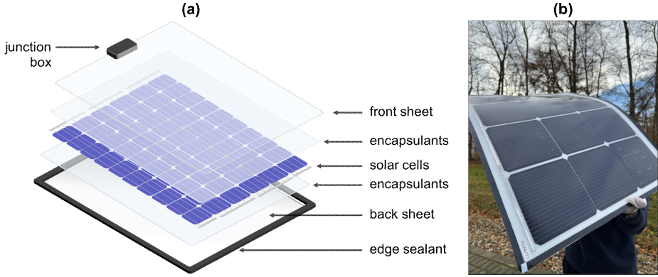
Figure 2.3: (a) Schematic structure of a lightweight c-Si solar module and (b) a prototype lightweight SHJ solar module developed in this work.
