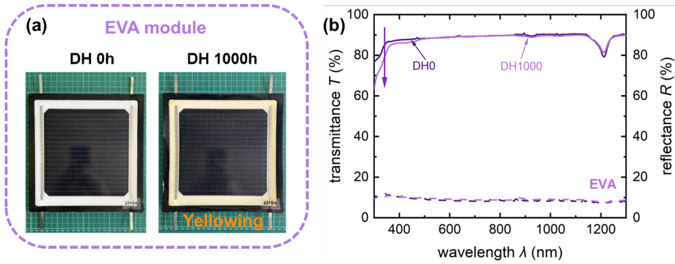
Figure 5.13: (a) Visual images of EVA-encapsulated solar modules before and after 1000 h of the DH test. (b) Transmittance (solid line) and reflectance (dashed line) of EVA encapsulant foil before and after 1000 h of the DH test.
