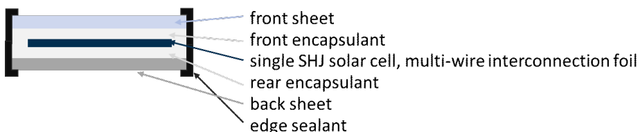
Figure 3.1: Schematic cross-section of the lightweight SHJ single-cell solar module (preliminary design).
