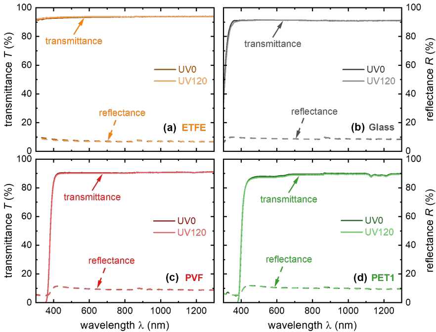
Figure 6.1: Transmittance ( T , solid line) and reflectance ( R , dashed line) spectra of different front sheet materials: (a) ETFE, (b) glass, (c) PVF, and (d) PET1, before and after 120 kWh/m 2 of UV exposure.
