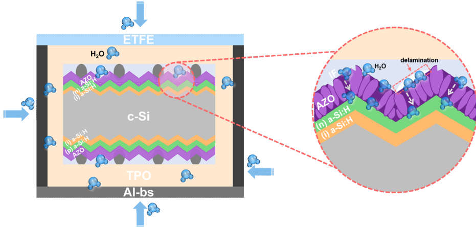
Figure 4.21: Schematic diagram of moisture ingress and degradation mechanisms in lightweight AZO-incorporated SHJ solar modules.
