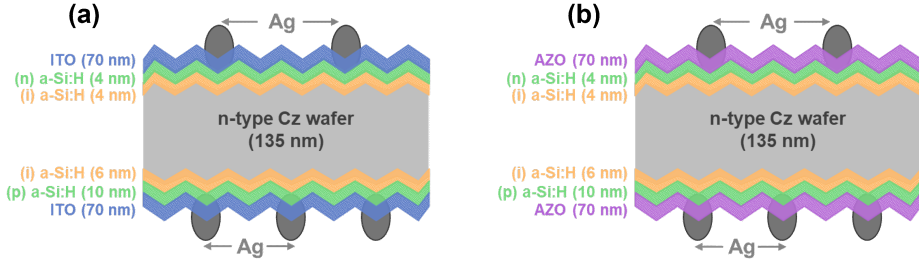
Figure 4.1: Schematic cross-section of SHJ solar cells with different TCO layers: (a) ITO at the front and rear sides and (b) AZO at the front and rear sides.
