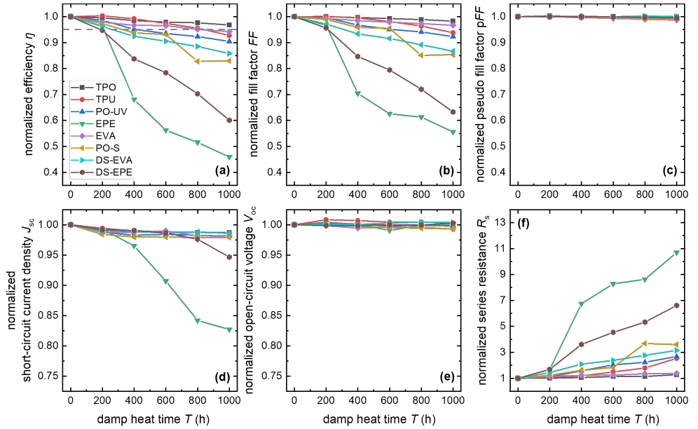
Figure 5.7: Normalized values of (a) efficiency ( \eta ), (b) fill factor ( FF ), (c) pseudo fill factor ( pFF ), (d) short-circuit current density ( J_{sc} ), (e) open-circuit voltage ( V_{oc} ), and (f) series resistance ( R_s ) as a function of damp-heat time for solar modules encapsulated with different encapsulants.
