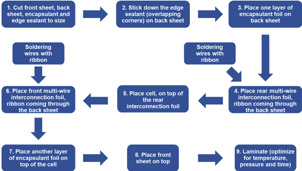
Figure 3.9: Fabrication process of lightweight SHJ single-cell solar modules (optimized design).
