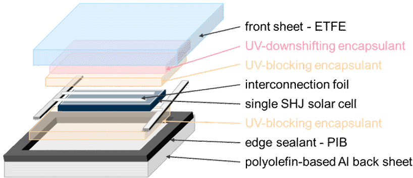
Figure 6.18: Schematic of the lightweight SHJ single-cell solar module with a dual-layer front encapsulant.
