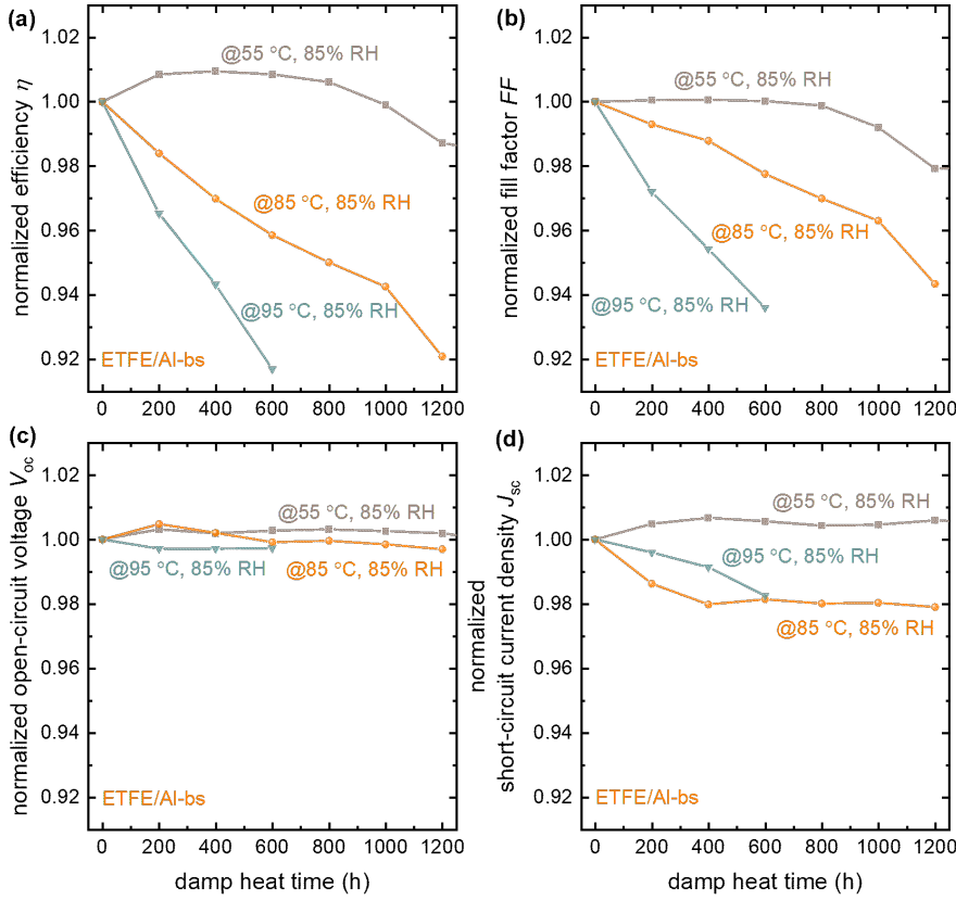
Figure 5.26: Normalized values of (a) efficiency ( \eta ), (b) fill factor ( FF ), (c) open-circuit voltage ( V_{oc} ), and (d) short-circuit current density ( J_{sc} ) as a function of damp-heat exposure time for the ETFE/Al-bs solar module under DH test conditions of 85°C, 85% RH, 55°C, 85% RH, and 95°C, 85% RH.
