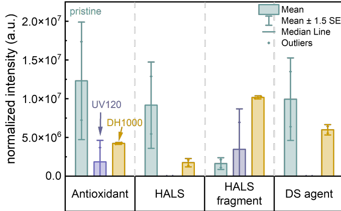
Figure 6.4: Normalized intensity of the additives before and after 120 kWh/m 2 UV or 1000 h DH exposure, quantified by Pyrolysis-Gas chromatography-Mass spectrometry (PY-GC-MS).
