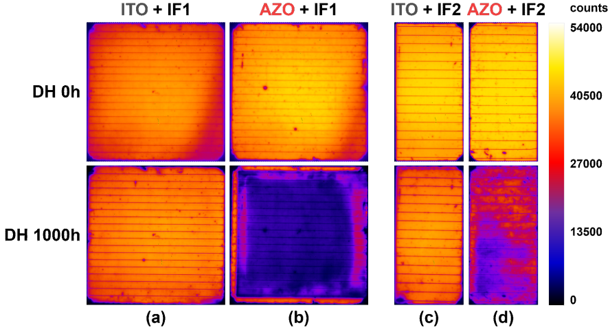
Figure 4.28: PL images of ITO- and AZO-incorporated FS/BS solar modules in combination with two different interconnection foils (IF1 and IF2), before and after 1000 h of DH. (a) ITO + IF1, (b) AZO + IF1, (c) ITO + IF2, and (d) AZO + IF2.
