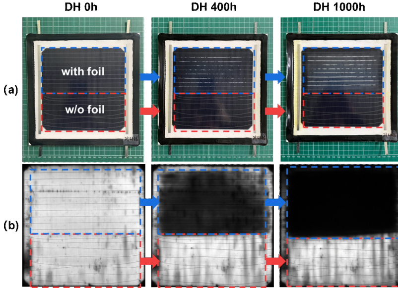
Figure 4.20: AZO-incorporated SHJ solar module with interconnection foil (wires and interconnection foil, blue dashed line) and without interconnection foil (only wires, red dashed line). (a) Visual images before, after 400 h, and after 1000 h of the DH test; (b) EL images at low current injection ( J = 2.03 \text{ mA/cm}^2 ) taken before, after 400 h, and after 1000 h of the DH test.
