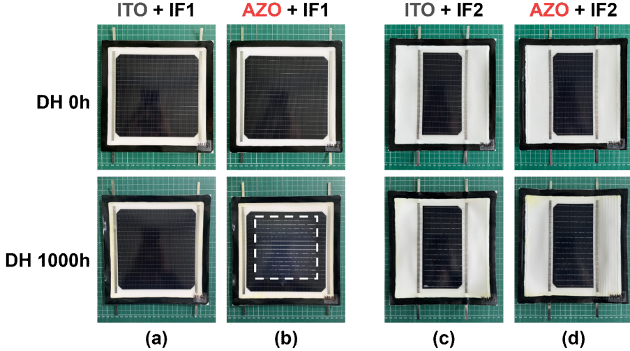
Figure 4.26: Visual images of ITO- and AZO-incorporated FS/BS solar modules in combination with two different interconnection foils (IF1 and IF2), before and after 1000 h of the DH test. (a) ITO + IF1, (b) AZO + IF1, (c) ITO + IF2, and (d) AZO + IF2.
