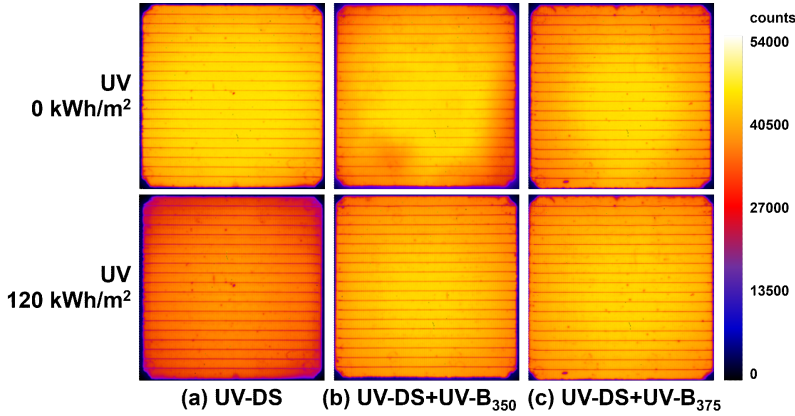
Figure 6.20: PL images of lightweight SHJ solar modules with (a) UV-DS, (b) UV-DS+UV-B 350 , and (c) UV-DS+UV-B 375 before and after 120 kWh/m 2 of UV exposure.
