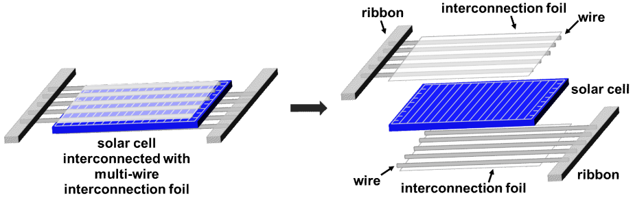
Figure 3.2: Schematic of a single 0BB SHJ solar cell interconnected with a multi-wire interconnection foil and its layer stack.
