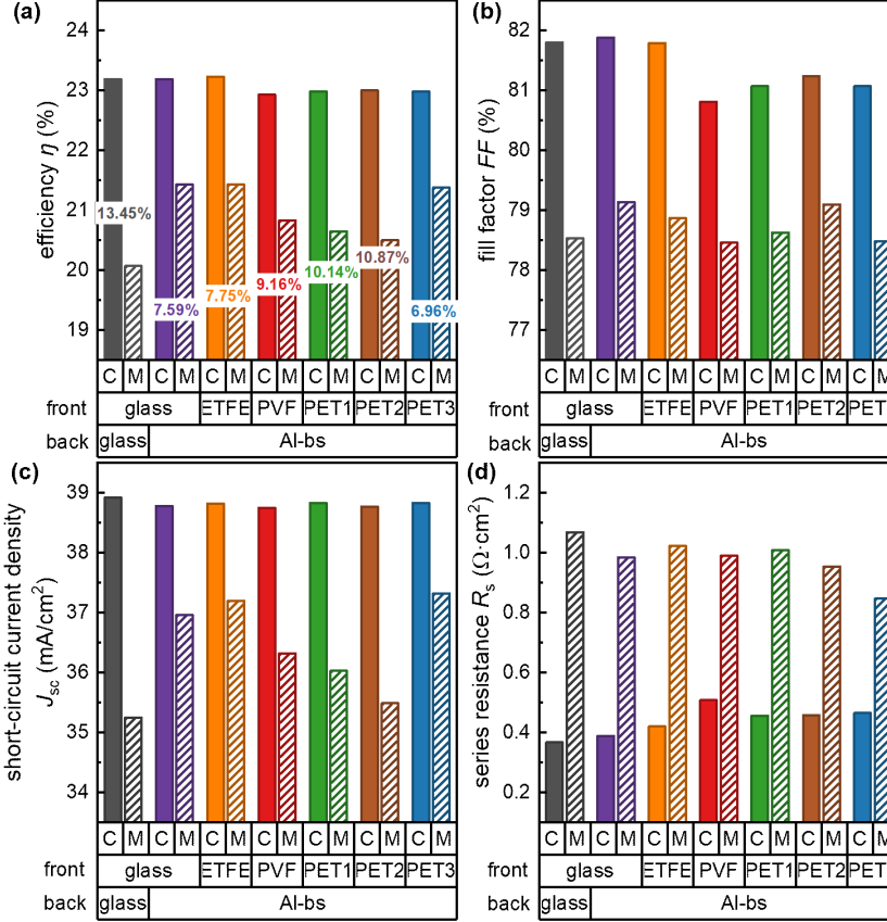
Figure 5.22: CTM loss from (a) efficiency ( \eta ), (b) fill factor ( FF ), (c) short-circuit current density ( J_{sc} ), and (d) series resistance ( R_s ) of solar modules with different configurations. 'C' denotes solar cell, and 'M' denotes solar module. The numbers in the graph indicate the CTM efficiency loss.
