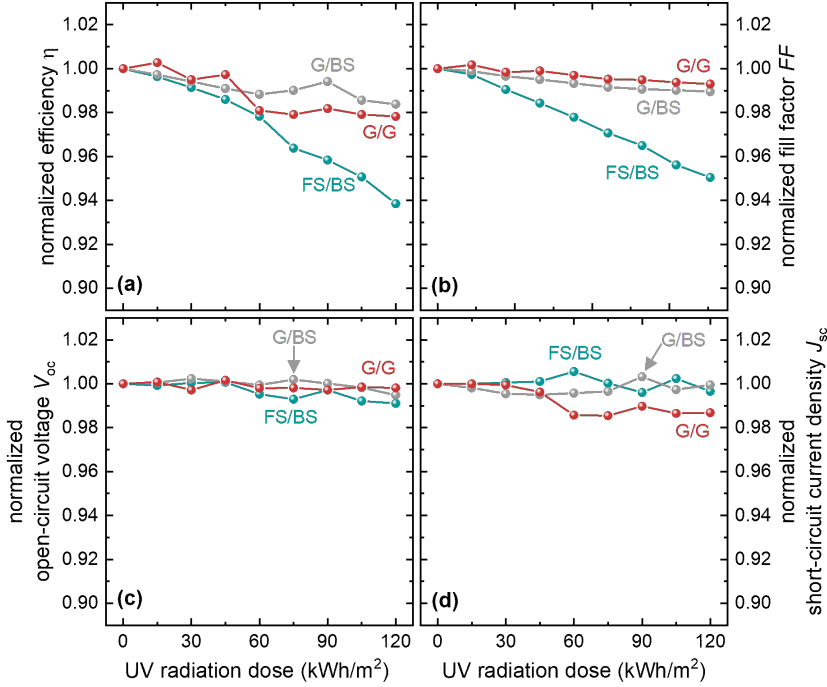
Figure 6.15: Normalized values of (a) efficiency ( \eta ), (b) fill factor ( FF ), (c) open-circuit voltage ( V_{oc} ) and (d) short-circuit current density ( J_{sc} ) as a function of UV radiation dose for solar modules with UV-DS encapsulant in different solar module structures: front sheet/back sheet (FS/BS), glass/back sheet (G/BS) and glass/glass (G/G) solar modules.
