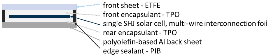
Figure 4.23: Schematic cross-section of the lightweight SHJ single-cell solar module.
