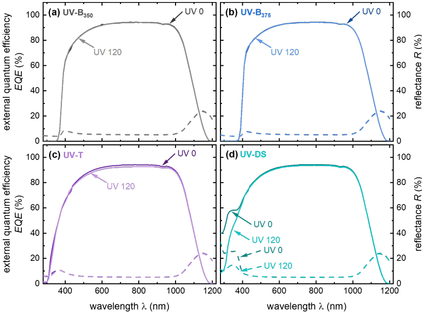
Figure 6.11: EQE (solid line) and reflectance (dashed line) of lightweight SHJ solar modules incorporating encapsulants with different UV-transmission properties: (a) UV-B 350 , (b) UV-B 375 , (c) UV-T, and (d) UV-DS, measured before and after 120 kWh/m 2 of UV exposure.
