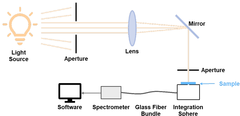
Figure 3.12: Schematic mechanism of the adapted optical measurement setup.
