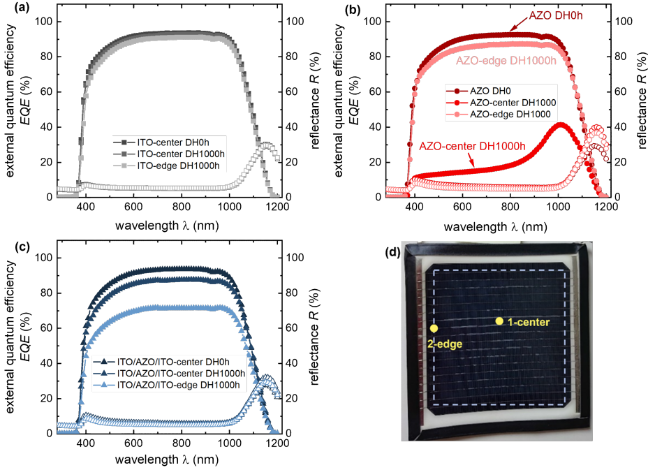
Figure 4.22: EQE (solid symbols) and reflectance (hollow symbols) of (a) ITO-, (b) AZO-, (c) ITO/AZO/ITO-incorporated SHJ lightweight solar modules before and after 1000 h of the DH test. (d) The light spot positions, 1-center and 2-edge.
