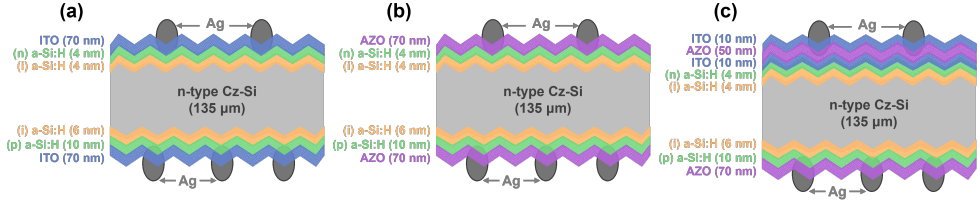
Figure 4.12: Schematic cross-section of SHJ solar cells with different TCO layers: (a) ITO layers at both the front and rear sides, (b) AZO layers at both the front and rear sides, and (c) a triple-layer front TCO stack of ITO/AZO/ITO and an AZO layer at the rear side.
