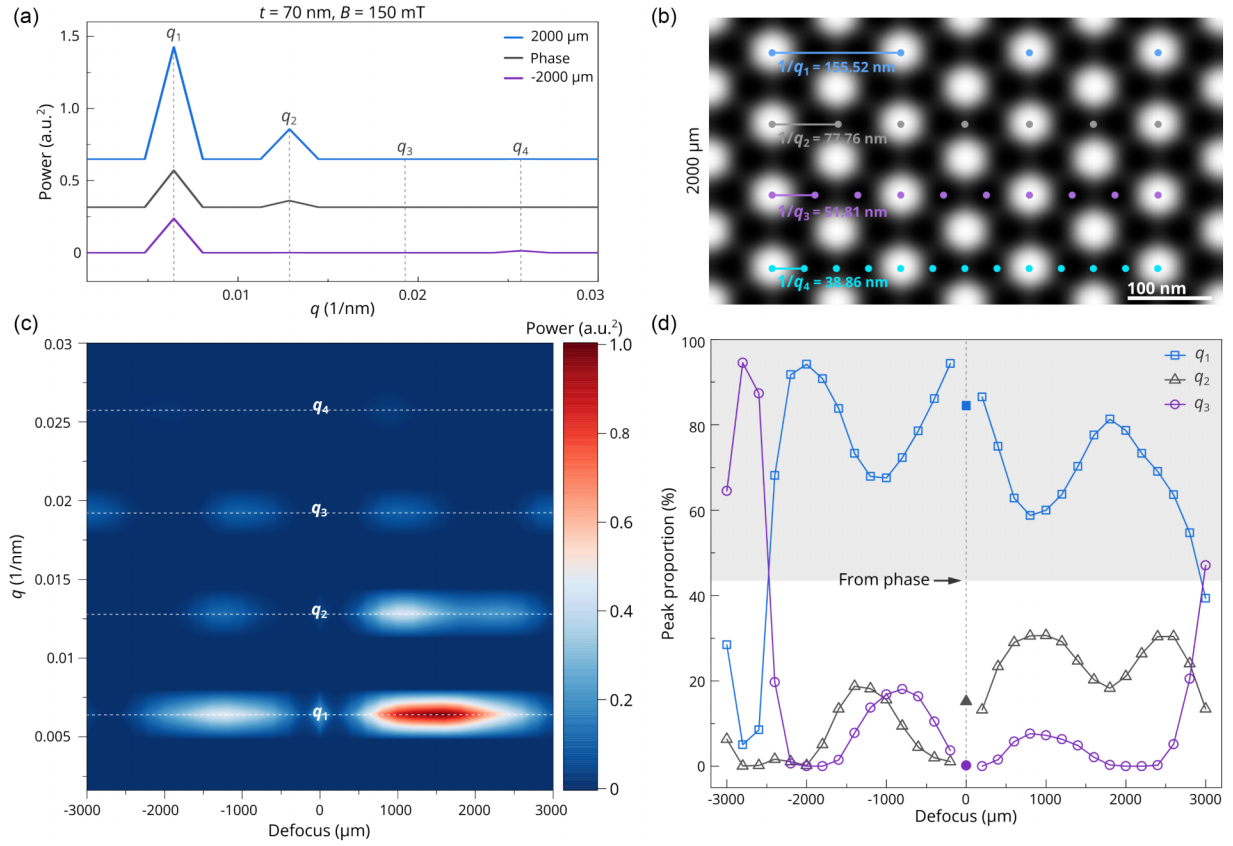
FIG. 8. Periodicity analyses of skyrmion-lattice patterns as a function of the defocus distance in the 70-nm-thick sample. (a) Representative FFT power spectra of the intensity profile along the gray line [marked in Fig. 6(a)]. The intensity profiles are from the Lorentz images at a defocus distance of 2000 \mu m. The FFT power spectrum of the phase is also used for comparison. The applied magnetic field is 150 mT. The characteristic peaks in the frequency domains are labeled as q_1 , q_2 , q_3 , and q_4 . Their corresponding spatial spacings are marked in (b) on the over-focus Lorentz images at a defocus distance of 2000 \mu m. (c) Two-dimensional FFT power spectra as a function of the defocus distance. Each vertical line in the spectrum corresponds to a similar spectrum shown in (a). The dominant peaks are localized judging from the values and labeled. (d) Evolution of the proportions of three dominant peaks (characteristic frequencies) as a function of the defocus. The dominant peaks from the phase are also plotted for comparison.
