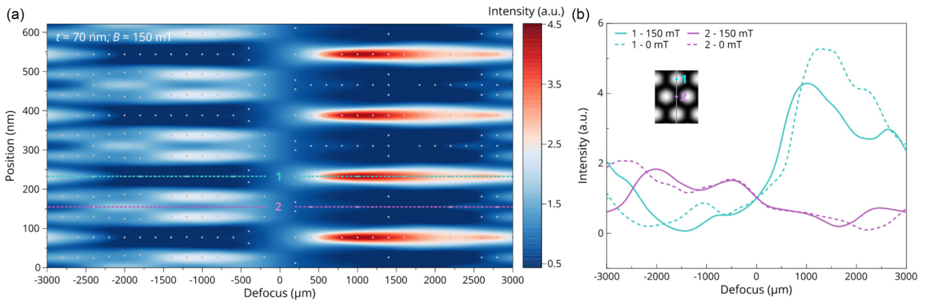
FIG. 7. Analyses of simulated Lorentz TEM images of the skyrmion lattice in the 70-nm-thick sample. (a) Intensity map for the points along the gray line [marked in Fig. 6(a)] as a function of the defocus distance. (b) Intensity profiles for the two particular points as a function of the defocus distance. “1” and “2” denote the skyrmion center and the center between two adjacent skyrmions, respectively [see the inset in (b)]. Two lines mark the positions of the two points in (a). In addition, intensity profiles for the lattice at 0 mT (dashed lines) are also plotted for comparison.
