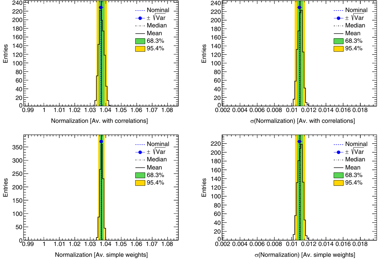
FIG. 5. Distributions of the normalization rescaling factor \gamma_1 (left) and its uncertainty propagated from the covariance matrices of the lattice QCD and dispersive results (right), obtained by sampling the bootstrap replicas of the lattice covariance matrix. These figures show the effects of different approaches to determining \gamma_1 and its uncertainty in the low-mass region below 0.96 GeV. Two moment integrals are considered here, with the lattice covariance matrix 0. In the first row, we consider normalization fits using the full covariance matrices of the \tilde{\gamma}_j for determining the averaging weights. In the second row, we consider normalization fits with the averaging weights proportional to the inverse of the \tilde{\gamma}_j uncertainties squared. The blue horizontal line indicates the asymmetric variance of the distribution, computed on each side of the nominal value (dashed blue vertical line). The median (dash-dotted black line), mean (black continuous line), 68.3% and 95.4% quantiles (colored bands) of the distribution are also indicated.
