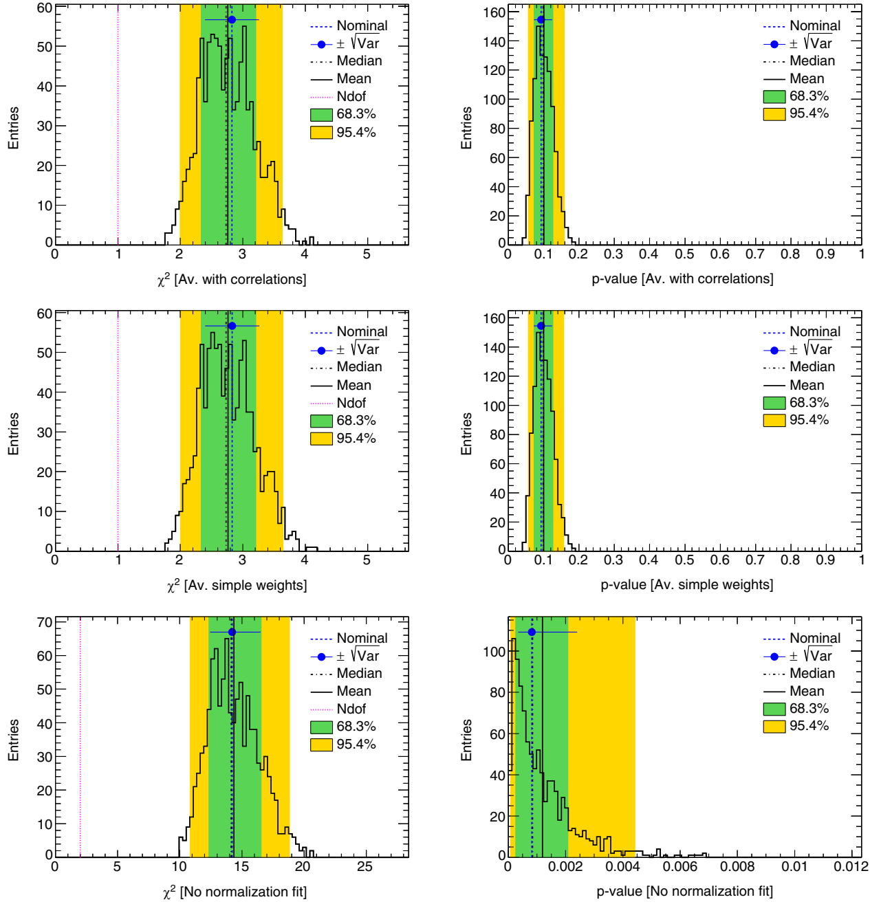
FIG. 4. Distributions of \chi^2 (left) and p -value (right) obtained by sampling the bootstrap replicas of the lattice covariance matrix. These figures show the effects of different approaches to determining \gamma_1 and its uncertainty in the low-mass region below 0.96 GeV. Two moment integrals are considered here, with the lattice covariance matrix 0. In the first row, we consider normalization fits using the full covariance matrices for determining the averaging weights—their comparison with the two plots in the following row is discussed in Appendix D. In the middle row, we consider normalization fits with the averaging weights proportional to the inverse of the \tilde{\gamma}_j uncertainties squared, as considered in the present section. In the final row, we set the \gamma_b normalization coefficients to unity, i.e., we perform no rescaling—these are discussed in Sec. VA. The blue horizontal error bar indicates the asymmetric variance of the distribution, computed on each side of the nominal value (blue point and blue dashed vertical line). The median (dash-dotted black line), mean (black continuous line), 68.3% and 95.4% quantiles (colored bands) of the distribution are also indicated. The number of degrees of freedom in the \chi^2 calculation is indicated by the dotted pink line. Note that the scales in the last row of plots (corresponding to no rescaling) are very different from those of the two previous rows (in which rescaling is allowed) to account for the fact that the \chi^2 and p -values with no rescaling are very poor.
