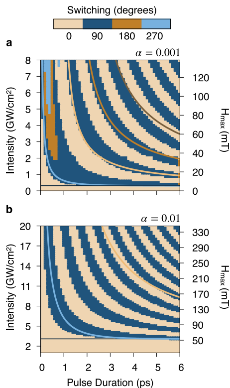
Fig. 4 | Switching phase diagram in terms of laser intensity and duration. Colours represent the end change of angle from \langle 110 \rangle . The corresponding maximum field strength for the laser intensity is given on the second y-axis. Solid colour lines show the analytic H_{crit} values from Eq. (7) a for \alpha = 0.001 . Black line: H_{crit} = \omega_A / (2\gamma) = 5.16 mT. b \alpha = 0.01 Black line: 10 \times H_{crit} , showing that the critical field scales linearly with damping parameter.
