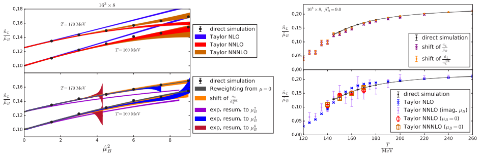
Figure 1. Left: The direct results for \hat{n}_L at non-zero \mu_B compared with different approximations (or extrapolations): the Taylor method to different orders up to p_8 and the exponential resummations [5] to order N = 2, 4 and 6 , calculated from the ensemble at \mu_B = 0 , as well as the shifting n_L/n_L^{\text{SBL}} method calculated from imaginary chemical potential simulations and reweighting from \mu_B = 0 . Right: The density \hat{n}_L as a function of the temperature T for \hat{\mu}_B = 3 for the ordinary Taylor expansion (bottom) and the resummation schemes based on shifting \hat{n}_L/\hat{\mu}_B and \hat{n}_L/\hat{n}_L^{\text{SBL}} (top). The direct Taylor data from \mu_B = 0 simulations has smaller errors than the fit to imaginary \mu_B data. This is mainly due to the small volume in our study. For larger volumes, the signal-to-noise ratio of the direct p_6 and p_8 would be considerably larger. A spline interpolation of the direct results is included to lead the eye.
