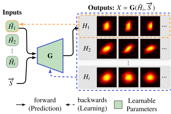
Fig. 2. Adapted StyleGAN architecture for focal spot prediction. This diagram illustrates how heliostat properties, represented as vectors \tilde{H}_i , and sun position vectors \vec{S} , feed into the StyleGAN generator G to produce focal spots. The process involves comparing predicted focal spots with actual measurements to inform the training loss. Each heliostat's specific parameters \tilde{H}_i are fine-tuned based on its associated focal spots, whereas the generator G is universally trained across the entire dataset.
