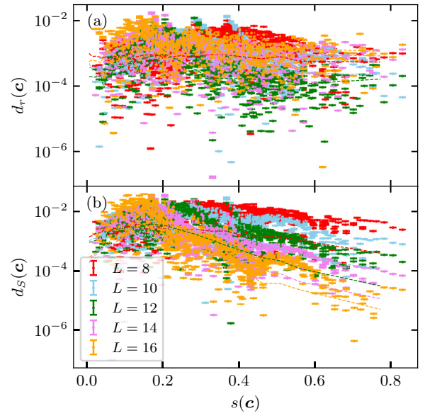
FIG. 10. Distance of (a) the gap ratio r(c, L) and (b) entanglement entropy S(c, L) to the reference values r(c_s, L) and S(c_s, L) on the SWAP line. Dashed lines are error bars of r(c_s, L) and S(c_s, L) . The SWAP reference points are computed by using spline interpolation of the curves shown in Fig. 4. The points are the same data as shown in Fig. 3.
