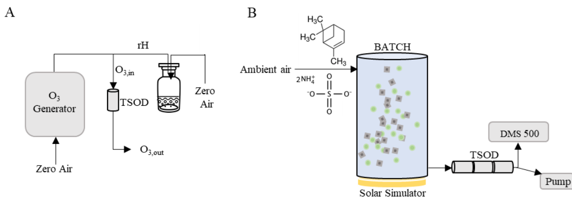
Figure 1. Schematic of the laboratory test-bed for assessing the \text{O}_3 removal efficiency (A) and potential particle losses of TSODs (B). (A) \text{O}_3 was generated, diluted with zero air, humidified to \sim 50\% relative humidity, and passed through the TSOD. Downstream \text{O}_3 mixing ratios were measured using an \text{O}_3 analyzer. (B) For particle loss tests, the setup was connected to the BATCH, where SimOA was generated from \alpha -pinene oxidation with ammonium sulfate seed particles and ambient air. The aerosol flow was directed through three TSODs, and particle size distributions were measured downstream using a DMS500.
