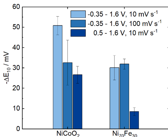
Fig. 3. Activation ( -\Delta E_{10} ) at 10 \text{ mA cm}^{-2} of \text{NiCoO}_2 and \text{Ni}_{70}\text{Fe}_{30} due to conditioning performed in 1 M KOH at RT with SEQ01 ( -0.35 – 1.6 \text{ V} vs. RHE, 10 \text{ mV s}^{-1} ), SEQ02 ( -0.35 – 1.6 \text{ V} vs. RHE, 100 \text{ mV s}^{-1} ) and SEQ03 ( 0.5 – 1.6 \text{ V} vs. RHE, 10 \text{ mV s}^{-1} ). Please note that the bulk \text{Ni}_{70}\text{Fe}_{30} underwent 46 cycles (5 h, 0.5 h and 2.8 h total conditioning time for SEQ01, SEQ02 and SEQ03, respectively) while all powder-coated anodes underwent 300 cycles (32.5 h, 3.25 h and 18.3 h total conditioning time for SEQ01, SEQ02 and SEQ03, respectively). Catalyst loading is \approx 450 \mu\text{g cm}^{-2} .
