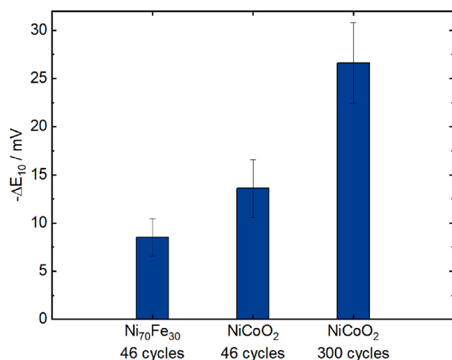
Fig. 2. Activation comparison of \text{Ni}_{70}\text{Fe}_{30} (46 cycles) and \text{NiCoO}_2 (46 cycles and 300 cycles). Conditioning was performed in the potential range of 0.5–1.6 V vs. RHE with 10 \text{ mV s}^{-1} .
