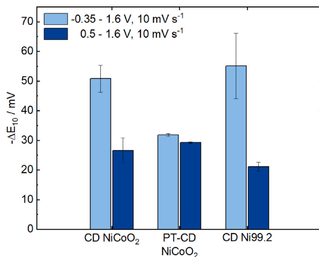
Fig. 6. Activation ( -\Delta E_{10} ) at 10 \text{ mA cm}^{-2} of conditioned NiCoO 2 , additionally plasma-treated NiCoO 2 and conditioned Ni99.2. SEQ01 ( -0.35 - 1.6 \text{ V vs. RHE} , 10 \text{ mV s}^{-1} ) and SEQ03 ( 0.5 - 1.6 \text{ V vs. RHE} , 10 \text{ mV s}^{-1} ) and 300 cycles were used for conditioning.
