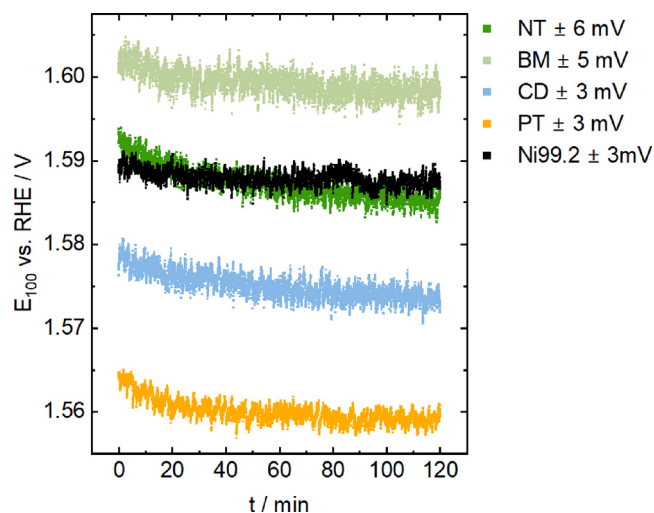
Fig. 4. Comparison of 2h CPs at 100 \text{ mA cm}^{-2} for \text{NiCoO}_2 catalyst layers with different pre-treatment methods: no treatment (NT), ball milling (BM), electrochemically conditioning (CD), plasma treatment (PT). The 2h CP of Ni99.2 is added as point of reference. The shown CP is the final of four CPs, as defined for the PAD protocol (see SI, section S3). The CD sample was conditioned with SEQ03 ( 0.5\text{--}1.6 \text{ V vs. RHE} , 10 \text{ mV s}^{-1} , 300 cycles). The given standard deviation is the mean value of the standard deviation in every time step.
