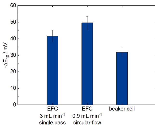
Fig. 1. Comparison of the activation of \text{Ni}_{70}\text{Fe}_{30} in the EFC and the beaker cell employed in this work. Conditioning settings were -0.35 – 1.6 \text{ V} vs. RHE, 100 \text{ mV s}^{-1} , 46 cycles, RT, 1 \text{ M KOH} .
