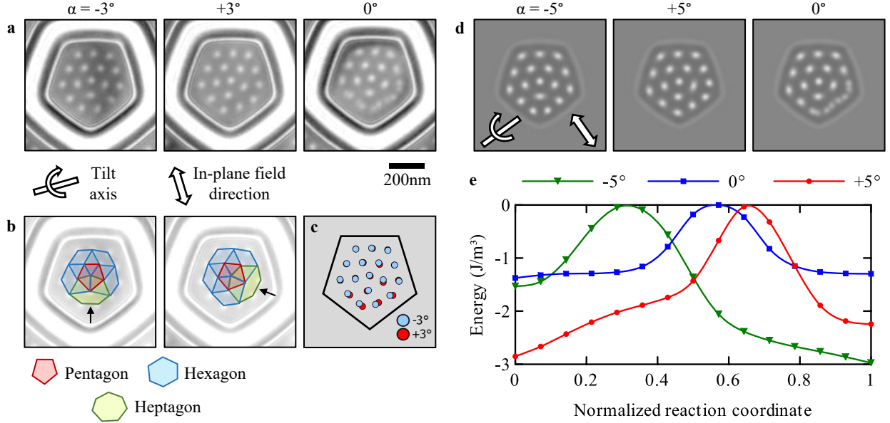
Figure 6. Skyrmion mobility around a disclination. (a) Fresnel images of a skyrmion lattice with S = 17 obtained in the presence of an external magnetic field of 230 mT at different tilt angles \alpha = -3^\circ , +3^\circ and 0^\circ . (b) Images obtained at -3^\circ and +3^\circ overlaid with pentagons, hexagons and heptagons. (c) Positions of the skyrmions in the two tilted images represented by blue and red dots. (d) Lorentz images calculated from micromagnetic simulations showing the lowest energy configuration at \alpha = -5^\circ and +5^\circ tilt angles. The image at 0^\circ is the sum of the previous images. (e) Energy paths for the transition between the two lattice configurations calculated for the three different tilt angles \pm 5^\circ and 0^\circ .
