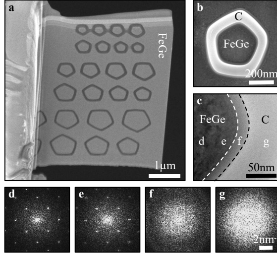
Figure 1. Sample description. (a) Representative scanning electron microscopy image of a TEM lamella of FeGe patterned with pentagons of different sizes. (b) TEM image of a small pentagon. (c) Magnified image of the FeGe/C interface. (d-g) Fourier transforms of different regions indicated in (c).
