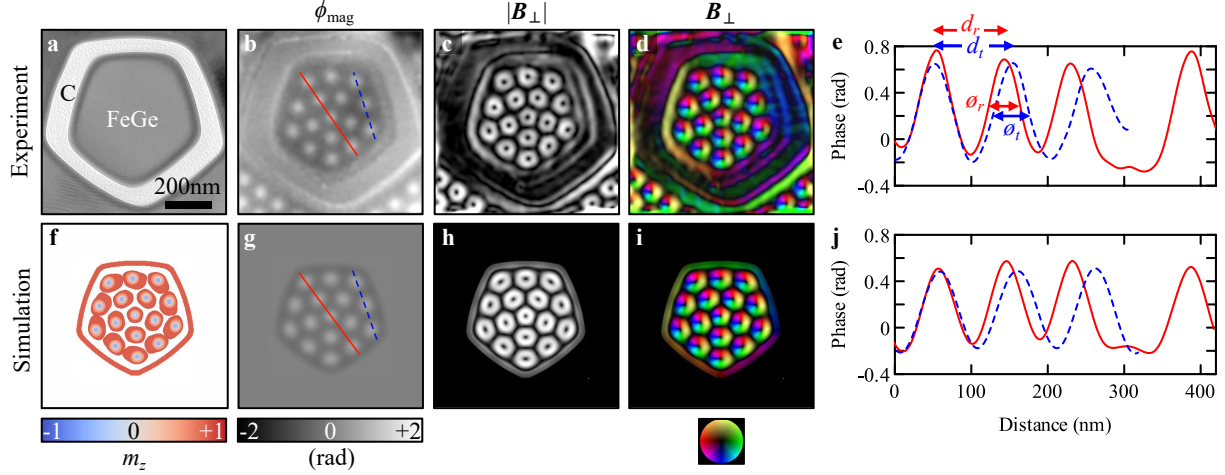
Figure 4. Electron holography of a 5-fold disclination. (a) Electron hologram of a pentagon-shaped sample recorded with an external magnetic field of 240 mT. (b) Magnetic phase image \phi_{\text{mag}} obtained using off-axis electron holography after subtraction of a phase image recorded at room temperature. (c) Magnitude of the in-plane magnetic induction field |\mathbf{B}_{\perp}| . (d) Corresponding color-coded map showing the direction of \mathbf{B}_{\perp} . (e) Phase profiles extracted from (b) along the solid and dashed lines. (f) Isosurface representation of the normalized out-plane component m_z of a magnetization model calculated using micromagnetic simulation. (g-j) Corresponding phase image, magnetic field maps and phase profiles.
