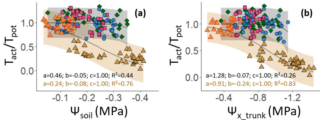
FIGURE 6. Relationships between (a) \Psi_{\text{soil}} and T_{\text{act}}/T_{\text{pot}} and (b) \Psi_{\text{x\_trunk}} and T_{\text{act}}/T_{\text{pot}} . The brown triangles, blue circles, pink squares and green diamonds correspond, respectively, to the subplots CBa, CBb, DWa and DWb. The brown triangles surrounded in red are data collected in 2023 in CBa. The relationships were fitted with 95 % functional prediction intervals (shaded area). The fitted parameters (a, b and c) in equation 4 and the fitting coefficient ( R^2 ) are given in the plots. Points corresponding to CBb, DWa and DWb have been assembled to predict the relationships between T_{\text{act}}/T_{\text{pot}} with \Psi_{\text{soil}} and \Psi_{\text{x\_trunk}} since these relationships are not different between these subplots ( p -value > 0.05; Table S1). \Psi_{\text{soil}} is equivalent to \Psi_{\text{x\_trunk\_PD}} .
