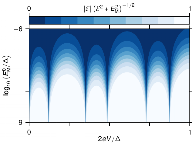
FIG. 5. The ratio |E|(\mathcal{E}^2 + E_M^2)^{-1/2} where \mathcal{E} = g_R/2 plotted as a function of the applied voltage V = \dot{\phi}/(2e) . All parameters are the same as in Fig. 2 in the main text, except for the number of lattice sites, which is here J = 400 instead of J = 200 . As a consequence, this doubles the frequency of oscillations as a function of V .
