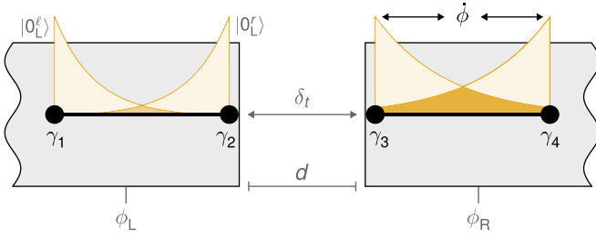
FIG. 1. Two tunnel-coupled topological superconducting wires, represented by the four Majoranas \{\gamma_1, \gamma_2, \gamma_3, \gamma_4\} . The wires are placed on top of two superconductors (gray), which interconnect at the far ends to form a loop threaded by a time-dependent magnetic field. The applied field leads to a phase difference \phi = \phi_R - \phi_L . The phase drop is included entirely in the right wire. The induced emf (owing to the time-dependent phase) strongly modifies the coupling between Majoranas \gamma_3 and \gamma_4 , which can be regarded as a strong renormalization of the overlap between the exponential tails of the Majoranas.
