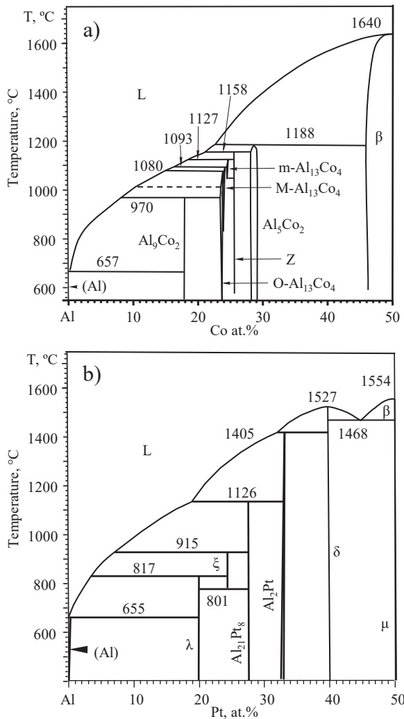
Fig. 1. Al-rich regions of the binary phase diagrams of: a) Al–Co according to Refs. [1,2], b) Al–Pt according to Refs. [3,4]. The provisional broken line in (a) separates the regions of L–O'-Al 13 Co 4 (above) and L–O-Al 13 Co 4 (below).
