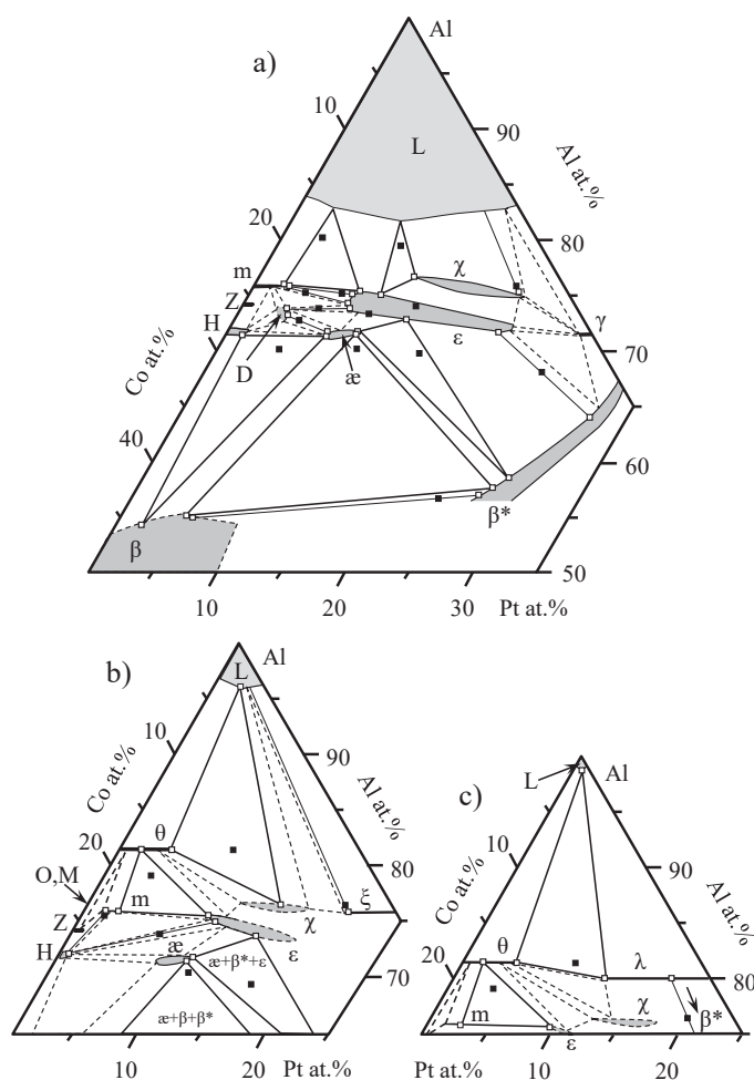
Fig. 5. Partial isothermal sections of Al–Co–Pt at: a) 1100 °C, b) 850 °C and c) 700 °C. L is the liquid. Provisional lines are shown broken. Measured compositions of the phases are marked by open squares and of the alloys by closed squares.
