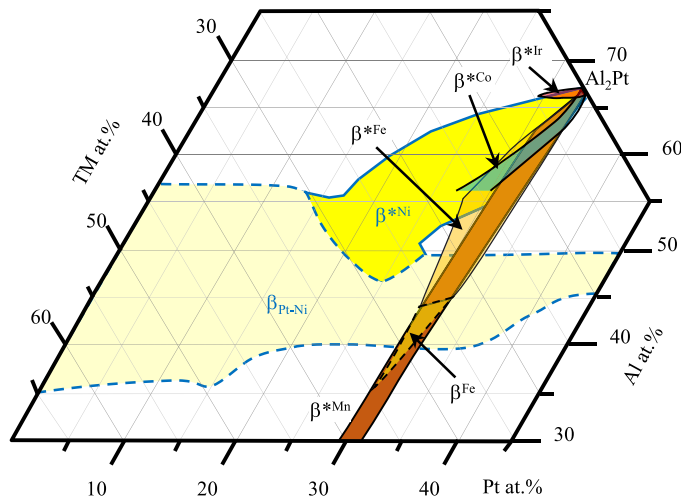
Fig. 6. Comparison of the ternary compositional regions of the \beta^* -phases forming in the Al–TM–Pt alloy systems. TM = Ni, Co, Fe, Mn, Ir and the compositional regions are designated as \beta^*_{\text{Ni}} [8], \beta^*_{\text{Co}} (this work), \beta^*_{\text{Fe}} [7], \beta^*_{\text{Mn}} [5], \beta^*_{\text{Ir}} [11], respectively with the corresponding references. The compositional region of the Al–Ni–Pt \beta_{\text{Pt-Ni}} phase is extrapolated to higher temperatures basing on the data in Ref. [8]. (in color in the web version).
