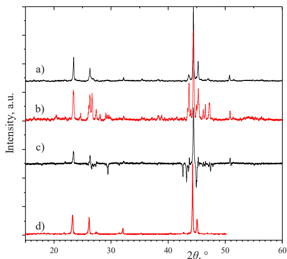
Fig. 4. Powder XRD patterns (Cu K \alpha 1 radiation) of the D-phase: a) in the as-cast Al 73 Co 22 Pt 5 alloy, b) in the same alloy annealed at 1100 °C for 142 h, c) as in (b) after subtraction of the powder XRD pattern of the Al 70 Co 25 Pt 5 alloy annealed at 1100 °C for 171 h. For comparison, in Fig. 4d the powder XRD pattern of the Al 71.4 Co 22.6 Ir 6 D-phase is reproduced from Fig. 8c of Ref. [16]. (in color in the web version).
