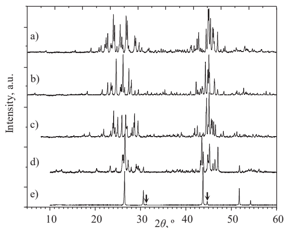
Fig. 2. Powder XRD patterns (Cu K \alpha 1 radiation) of the: a) Al 77 Co 3.5 Pt 19.5 alloy annealed at 850 °C for 431 h and containing the essentially single \xi_{\text{Pt}} -phase, b) Al 77 Co 3.5 Pt 19.5 alloy annealed at 1100 °C for 142 h and containing the major \chi -phase, c) Al 74 Co 13 Pt 13 alloy annealed at 1100 °C for 171 h and containing the single \epsilon_6 -phase, d) Al 70 Co 19 Pt 11 alloy annealed at 1100 °C for 142 h and containing the major \alpha -phase and minor \beta^* and \beta_{\text{Co}} , e) Al 57 Co 19 Pt 24 alloy annealed at 1100 °C for 171 h and containing the major \beta^* -phase and minor \beta_{\text{Co}} -phase (marked by arrows).
