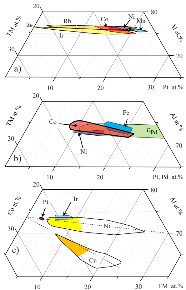
Fig. 7. Comparison of the compositional regions of the ternary: a) \chi -phases in Al–TM–Pt (TMs marked in the figure are Ir [11], Rh [10], Ni [8], Mn [5], Co); b) \epsilon -phases in Al–TM–Pt (TMs marked in the figure are Ni [8], Fe [7], Co) and in Al–Co–Pd [14]; c) D-phases in Al–Co–TM (TMs marked in the figure are Cu [15], Ni [15], Ir [16], Pt). In the Co-rich subregions colorized in (c), the D-phase with the periodicity of \sim 0.8 nm in the specific direction ( D_2 -phase) was revealed. The extrapolations of these compositional regions towards the binary Al–Co terminal marked by broken lines led to a composition of \sim \text{Al}_{73}\text{Co}_{27} . (in color in the web version).
