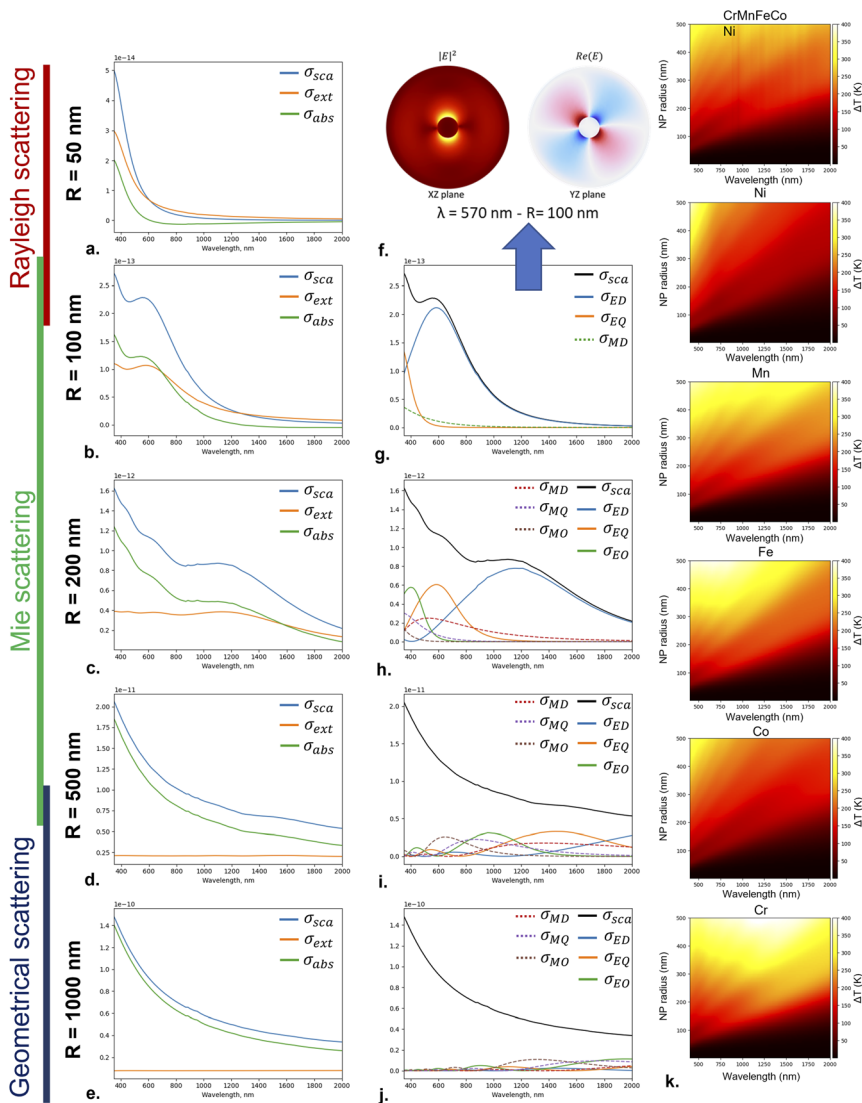
Fig. 6 Calculation of optical cross-sections and field distributions for HEA nanoparticles of different sizes. (a–e) Evolution of scattering ( \sigma_{\text{sca}} , blue), absorption ( \sigma_{\text{abs}} , green), and extinction ( \sigma_{\text{ext}} , orange) cross-sections for nanoparticles with radii of 50, 100, 200, 500, and 1000 nm, showing transitions from Rayleigh to Mie and then to geometrical scattering regimes. (f) Electric field distribution around a 100 nm radius nanoparticle at 570 nm wavelength in the XZ and YZ planes, revealing dipole-like behaviour. (g–j) Multipole decomposition of scattering cross-sections for nanoparticles of increasing size, showing contributions from various electric and magnetic modes (E: electric mode, M: magnetic mode, D: dipole, Q: quadrupole, O: octupole) (k) Temperature elevation of nanoparticles as a function of their radius and the incident wavelength for an incident power of I = 0.1 \mu\text{W} \mu\text{m}^{-2} .
