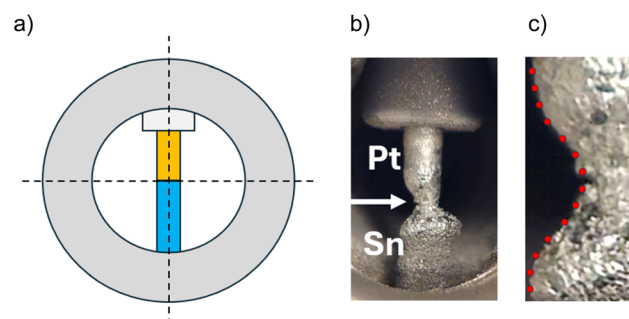
Fig. 2 (a) “Double rod” cathode configuration, where the two rods of Sn and Pt come into contact with each other, aligning the interface with the source centreline. (b) Image of the cathode after source operation, with the arrow highlighting the point of erosion. (c) Zoomed-in view of image (b), showing the Gaussian-like profile of the erosion.
