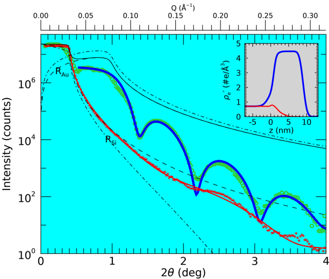
Figure 4 XRR from a 10 \times 10 \mu\text{m} Au island on a macroscopic Si wafer and from the bare substrate. The measured data from the Au island (open green symbols) are shown together with simulated Fresnel curves for the interfaces Si/vacuum and Au/vacuum (dashed lines), thereby taking into account that the 90 \times 90 \text{ nm} beam is only partly reflected from the island for small angles. Both Gaussian (dash) and Lorentzian (dash-dot) beam profiles are evaluated (see text for more details). Their combined reflectivity is shown as a black solid line. A fit to the data, starting from 2\theta = 0.55^\circ omitting the lower angles, and using a slab model consisting of a Au layer on a Si substrate, is also shown (blue). The XRR curve for the bare substrate, measured just beside the Au island, is shown as well (red asterisks), along with a fit (red). The inset shows the resulting (electron) scattering density profiles as obtained from the fitting procedures for the Au island (blue) and the bare Si substrate (red).
