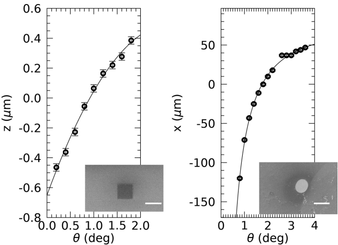
Figure 3 Results of sample alignment positions in grazing-incidence geometry. (Left) At different \theta – 2\theta positions, the height z of the sample, which consists of a 10 \times 10 \mu\text{m} Au island on a Si wafer, was scanned and the maximum reflected intensity was determined. The result of fitting equation (2) is shown as a solid line (black); fit parameters are listed in Table 1. The fit result using equation (4) is nearly identical and therefore not shown. The inset shows a scanning electron microscopy (SEM) image of the square Au island (scale bar represents 10 \mu\text{m} ). (Right) Lateral sample positions (symbols) whereby an approximately 100 \mu\text{m} polycrystalline Pt marker was aligned in the beam at grazing angle \theta and the Pt 111 (powder) Bragg reflection recorded. A fit of equation (1) is shown as a solid line (black); fit parameters are listed in Table 1. The fit result using equation (3) is nearly identical and therefore not shown. The inset shows an SEM image of the elliptical Pt marker (scale bar represents 100 \mu\text{m} ).
