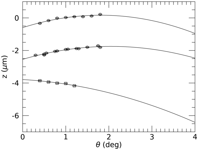
Figure 5 Alignment scans of Au islands. Shown are the results for the same 10 \times 10 \mu\text{m} Au island (open circles) as shown in Fig. 3, but with different prior alignment settings, such as sample tilts. Also shown are the results of a 100 \times 100 \mu\text{m} Au island (open squares). The results of fitting equation (2) are shown as solid lines; fit parameters are listed in Table 2.
