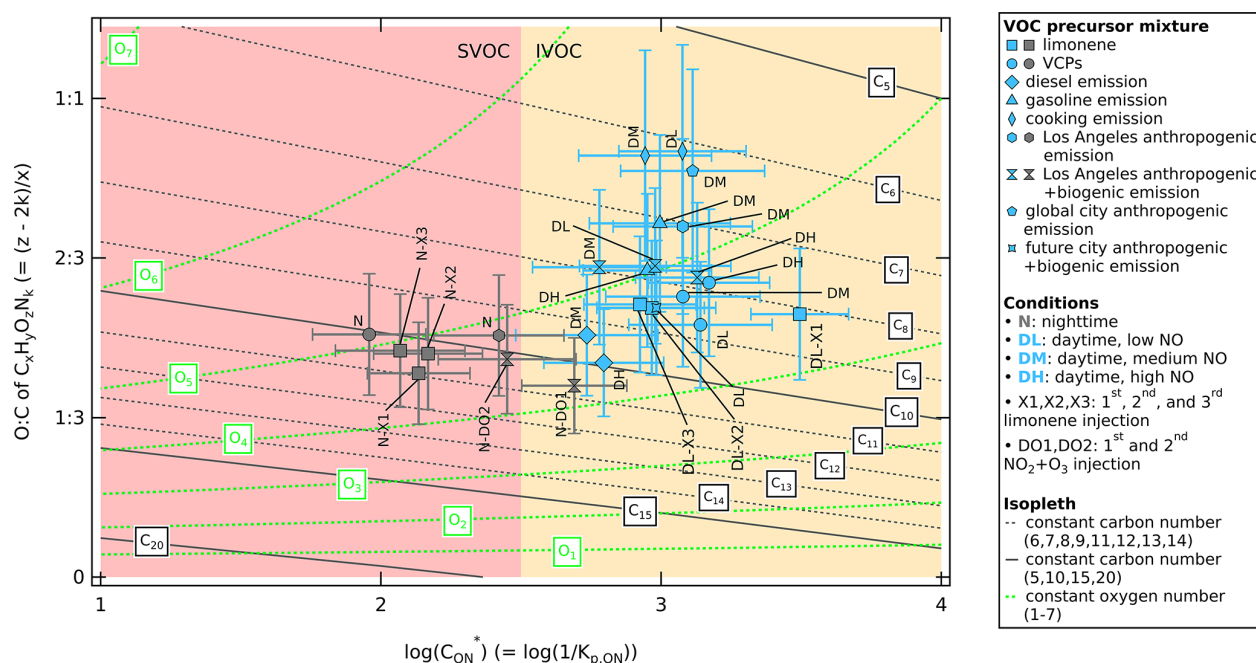
Figure 5. Two-dimensional volatility basis set mapping expressed as logarithm of effective saturation concentration of organic nitrate ( \log(C_{\text{ON}}^*) = \log(1/K_{\text{p,ON}}) ) in a 2D space with \log(C_{\text{ON}}^*) on the x axis and O : C ratio of \text{C}_x\text{H}_y\text{O}_z\text{N}_k ( = (z - 2k)/x ) on the y axis. The values of \log(C_{\text{ON}}^*) during SAPHIR-CHANEL campaigns for various urban VOC-NO x mixture experiments are shown color-coded by daytime (light blue) and nighttime (dark grey) conditions. The horizontal whiskers represent the uncertainty of \log(C_{\text{ON}}^*) (see Sect. S3.3 for uncertainty propagation). The vertical whiskers represent the uncertainty from using WALL-E signal as an indication of concentration (estimated to be 50 %). Organic composition from the group contribution method based on the carbon number ( n_{\text{C}}^i ) and oxygen number ( n_{\text{O}}^i ) are shown to describe organic aerosol volatility as isopleths at 300 K following Donahue et al. (2011), with parameterizations following Stolzenburg et al. (2018) as described in Sect. 2.5.1. The dark grey lines represent carbon number isopleths and the light green curves represent oxygen number isopleths. The volatility range of semi-volatile organic compounds (SVOC) and intermediate-volatility organic compounds (IVOC) are highlighted red and yellow, respectively.
