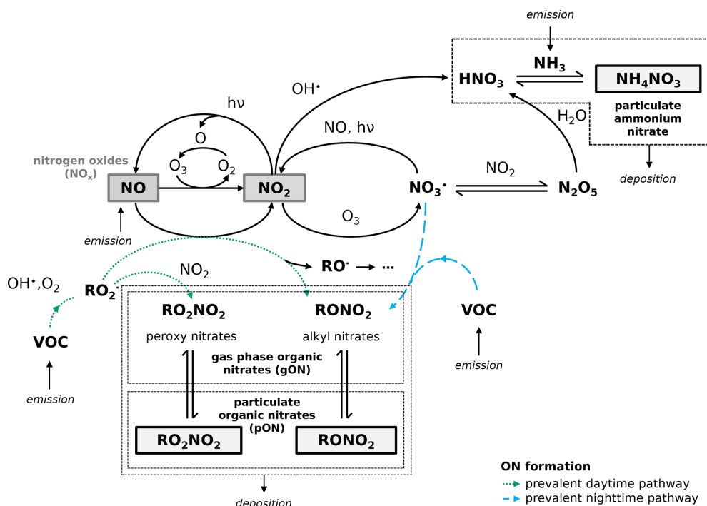
Figure 1. Reactive nitrogen species formation in the troposphere involving emissions of \text{NO}_x , \text{NH}_3 , VOCs, and their reactions with oxidants (e.g., \text{OH}^\bullet , and \text{NO}_3^\bullet ) to form particulate ammonium nitrate ( \text{NH}_4\text{NO}_3 ) and ONs that are in equilibrium between gas phase ON (gON) and particulate ON (pON). The dashed blue arrows represent the \text{NO}_3^\bullet chemistry pathway for ON formation prevalent during nighttime, while the dotted green arrows represent the \text{OH}^\bullet chemistry pathway for ON formation prevalent during daytime.
