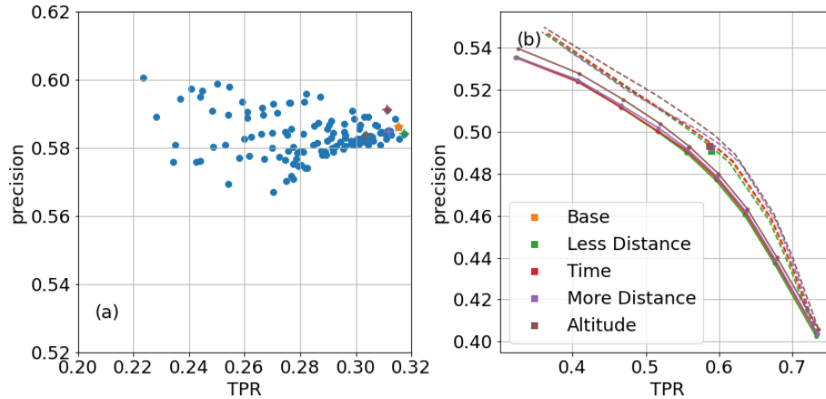
Figure 7. (a) Same as Fig. 3 but including the different thresholds in Table 4. The orange star shows the base case while the crosses show the other cases. (b) Same as Fig. 5a, but covering the different cases shown in Table 4.
