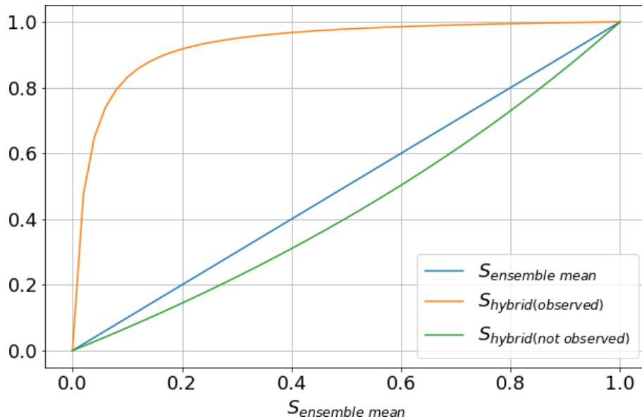
Figure 4. Scores computed using Eqs. (1) and (3). We can see that observing a contrail leads to a large increase in score compared to S_{\text{ensemble mean}} , while not observing a contrail leads to a small decrease in score.
