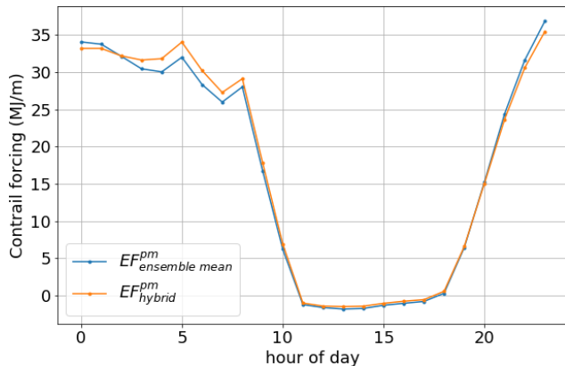
Figure 8. Energy forcing as a function of local time of day, for both EF_{ensemble}^{pm} and EF_{hybrid}^{pm} . We see that both have similar values and exhibit the expected diurnal pattern of warming at night and ambiguous results during the day.
