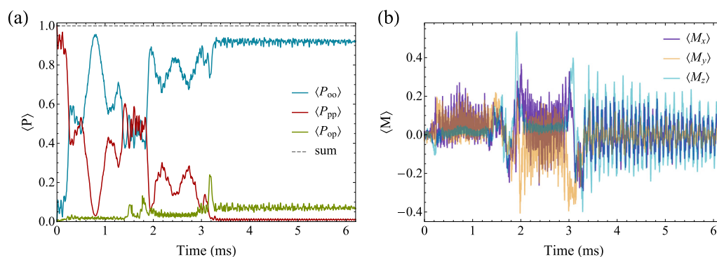
Fig. 13. Time evolution of the populations \langle P_{oo} \rangle , \langle P_{pp} \rangle , and \langle P_{op} \rangle (a), along with the average total spin projection components \langle M_x \rangle , \langle M_y \rangle , and \langle M_z \rangle (b) for the magnetic field shown in Fig. 9c with B_0 = 2.1 mT. All molecules are initially prepared in the para state.
