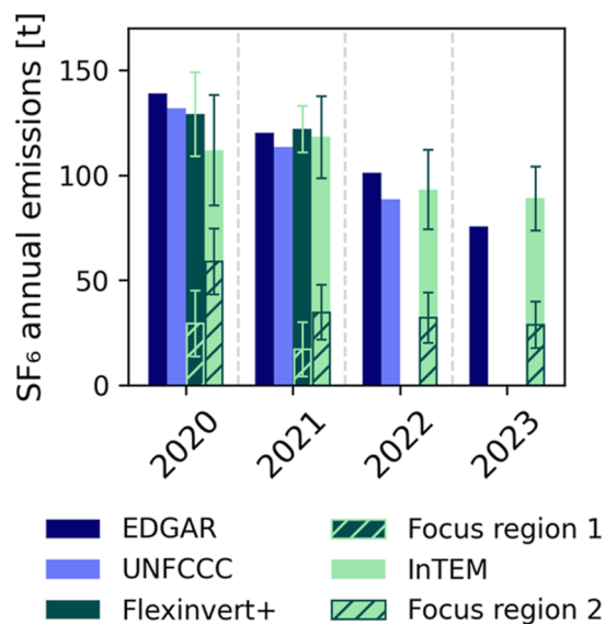
Figure 4. German \text{SF}_6 emission estimates [ \text{t yr}^{-1} ] from EDGAR (2020–2023), 70 UNFCCC inventory (2020–2022), 28 Flexinvert+ (2020–2021) 31 with focus region 1 (48.75 °N to 50.0 °N, 8.25 °E to 10.00 °E) and InTEM (2020–2023) with focus region 2 (48.637 °N to 49.807 °N, 8.404 °E to 10.164 °E). The error bars describe the 2\sigma uncertainty of the ensemble distribution for Flexinvert+ and the InTEM inversion results.
