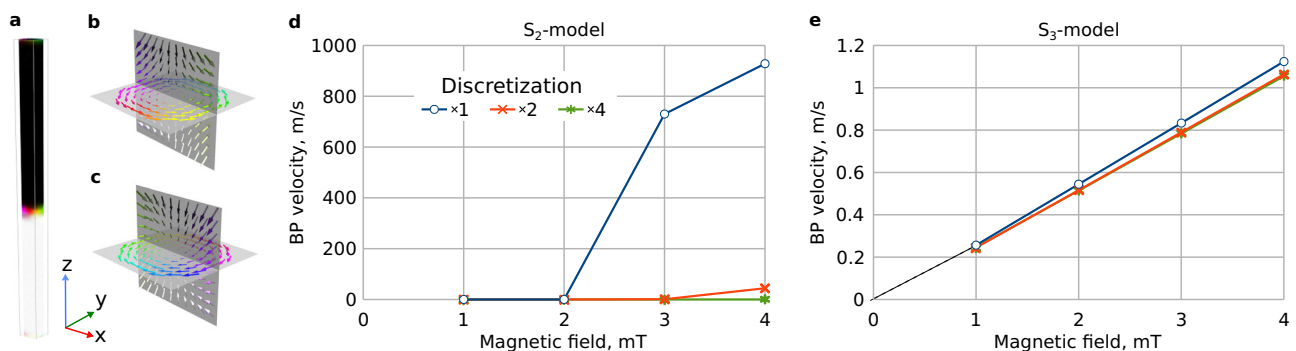
Fig. 3 | Bloch point dynamics in a nanowire. a A magnetic nanowire containing two domains magnetized along +\mathbf{e}_z (white) and -\mathbf{e}_z (black), which are separated by a domain wall containing a Bloch point (BP). In an external magnetic field B_{\text{ext}} \parallel \mathbf{e}_z , the BP moves along the wire axis. Simulations were performed for two domain-wall configurations, shown in (b) and (c) . Both configurations exhibit identical BP dynamics. d and (e) show the BP velocity as a function of the external magnetic field strength, computed using the standard and regularized LLG equations, respectively.
