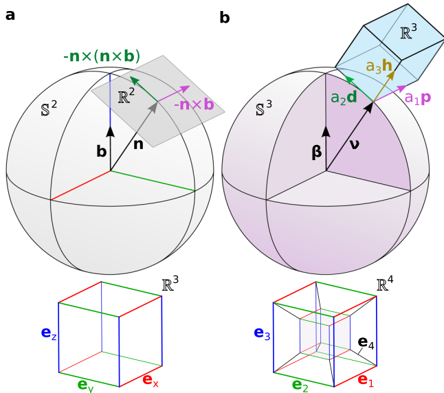
Fig. 1 | Geometric interpretation of the LLG equations in the S^2 and S^3 models. a,b illustrate the configuration spaces of the order parameter for the standard micromagnetic model constrained to the two-sphere S^2 , and the regularized model defined on the three-sphere S^3 , respectively. In (a) the three-dimensional unit vector \mathbf{n} lies on the two-sphere embedded in \mathbb{R}^3 space. The associated tangent space \mathbb{R}^2 contains orthogonal directions corresponding to the conventional basis vectors: \mathbf{n} \times \mathbf{b} (precession) and \mathbf{n} \times (\mathbf{n} \times \mathbf{b}) (damping). In (b) the four-dimensional unit vector \mathbf{v} is defined on the three-sphere S^3 embedded in \mathbb{R}^4 space. Note that in (b) , the vectors \mathbf{v} , \mathbf{p} , \mathbf{d} , and \mathbf{h} are mutually orthogonal in four-dimensional space; this orthogonality is represented schematically, as it cannot be faithfully depicted in a two-dimensional figure.
