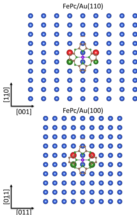
Fig. 9 Schematic representation of the \text{S}_{\text{b}}\text{Au}_{110}^{\text{nn}} and \text{S}_{\text{a}}\text{Au}_{100}^{\text{nn}} 6s AOs SALCs of symmetry b on the Au(110) (upper panel) and Au(100) (lower panel) bulk-terminated surfaces superimposed to the optimized \text{pmc}^{\text{FePc}} placed at 2.85 Å above the substrate and oriented with Fe–N Py bonds aligned to the [110] and [001] directions. Only Au(110) and Au(100) topmost layer atoms are displayed for clarity. Large spheres represent \text{S}_{\text{b}}\text{Au}_{110}^{\text{nn}} and \text{S}_{\text{a}}\text{Au}_{100}^{\text{nn}} 6s AOs, while different colors account for their different phases.
