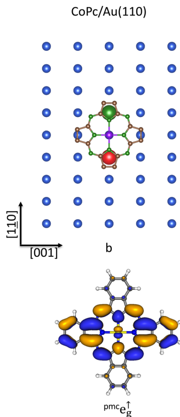
Fig. 6 Schematic representation of the {}^7\text{Au}_{110}^{\text{nnn}} 6s AOs SALC of symmetry b on the Au(110) bulk-terminated surfaces superimposed to the optimized {}^{\text{pmc}}\text{CoPc} placed at 3.0 Å above the substrate and oriented with Co–N py bonds aligned along the [110] and [001] directions. Only Au(110) topmost layer atoms are displayed for clarity. Large spheres represent {}^7\text{Au}_{110}^{\text{nnn}} 6s AOs, while different colors account for their different phases (upper panel). 3D CP of one component of the {}^{\text{pmc}}e_g^{\uparrow} SOs (lower panel). Displayed isosurfaces correspond to \pm 0.02 \text{ e}^2 \text{ Å}^{-3/2} values.
