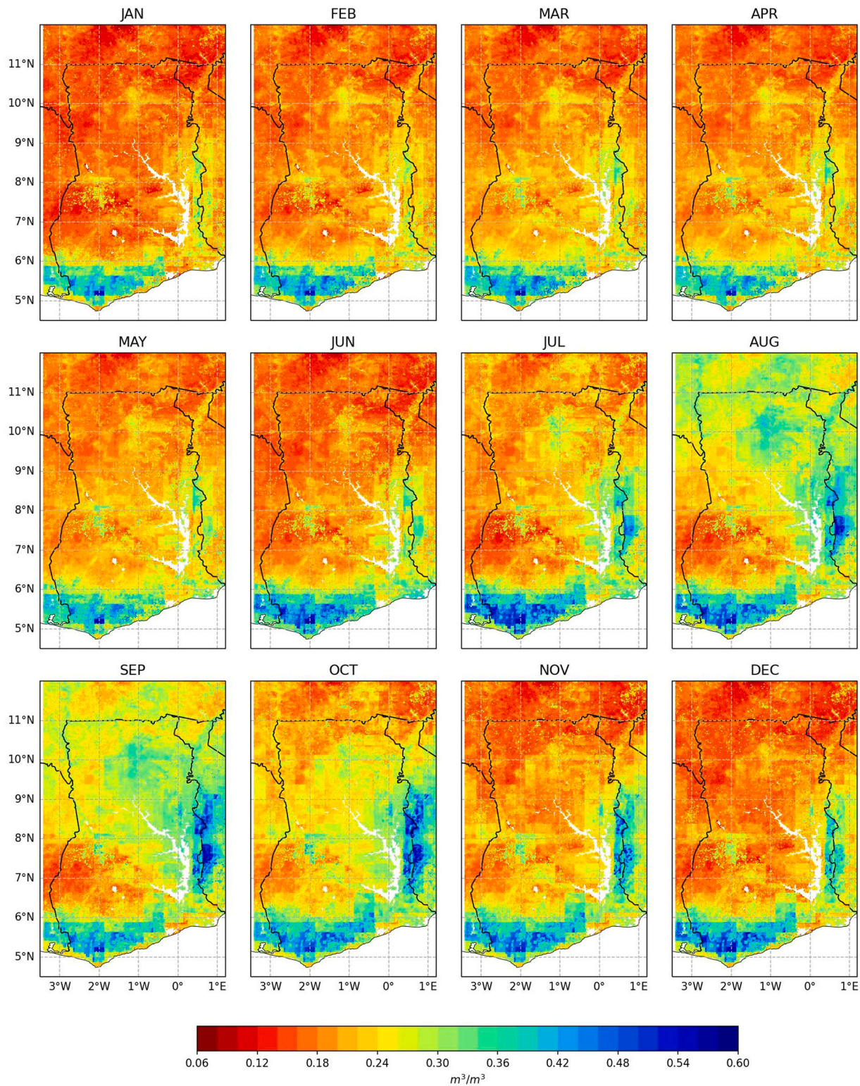
Fig. 2. Spatial distribution of CLM5 mean monthly soil moisture (0–6 cm) over Ghana from 2018 to 2023.
