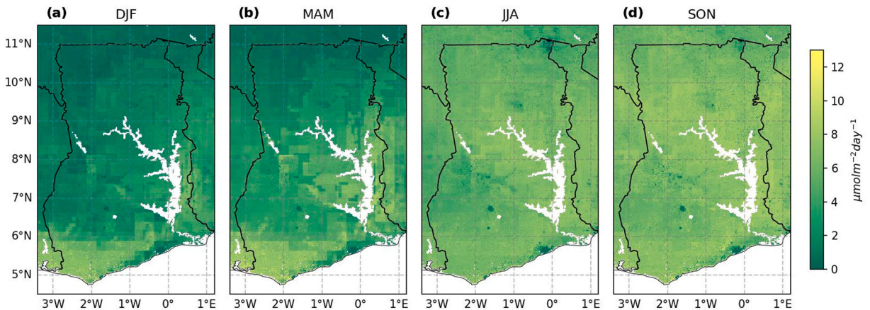
Fig. 7. Mean seasonal distribution of CLM5-simulated gross primary production (GPP) over Ghana between 2020 – 2024.
