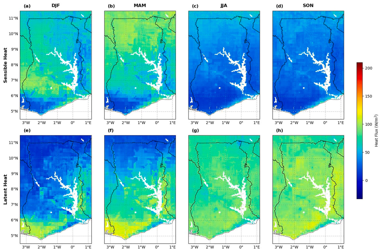
Fig. 5. Simulated mean seasonal distribution of sensible (a-d) and latent (e-h) heat fluxes over Ghana from 2020 to 2023.
