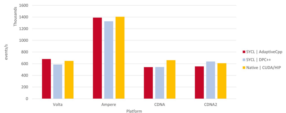
Fig. 11 Native GPU throughput
