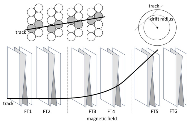
Fig. 2 Arrangement of the straws in the Forward Tracker. Each station is composed of four double layers (top left), with inclined inner layers (center, light, and dark grey). Highlighted straws (top left) respond to an exemplary track passing through the detector and bent by the magnetic field. The single straw response is presented on top, right
