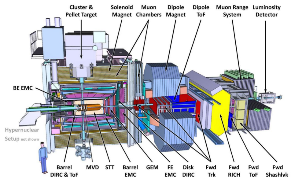
Fig. 1 Complete \overline{\text{P}} ANDA detector setup. Forward Tracker stations FT12, FT34 and FT56 shown as Fwd Trk from left to right
