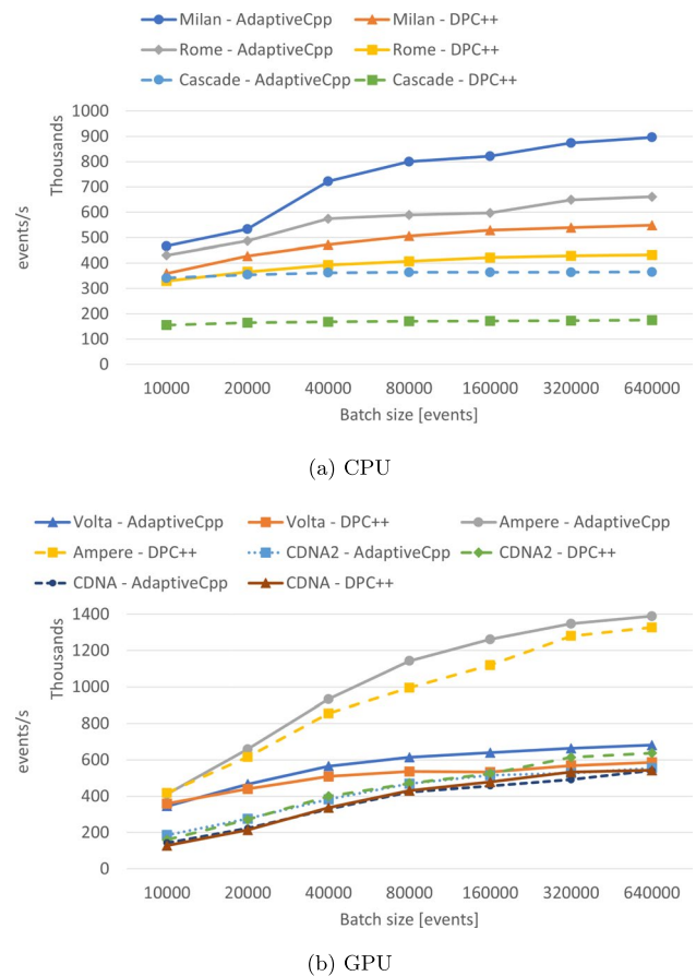
Fig. 5 Throughput changes under different batch sizes
