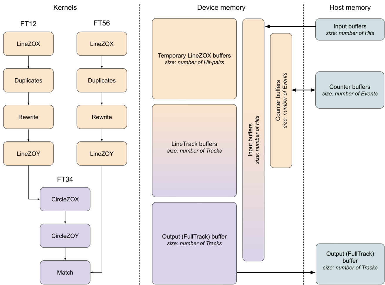
Fig. 4 Kernel data dependency and data flow graph
